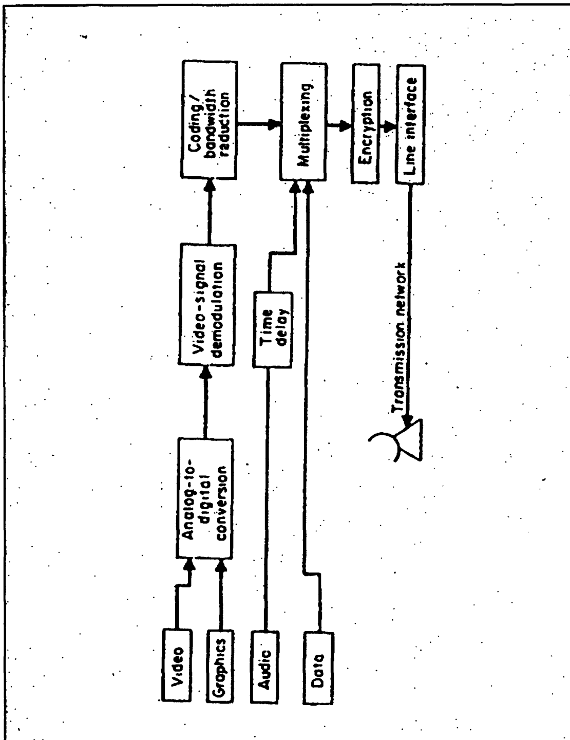
Figure 1 Video CODEC Functional Diagram[Ref. 3:p. 18.8]
