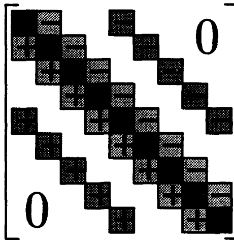
Figure 2. Two-Dimensional System Matrix Structure
