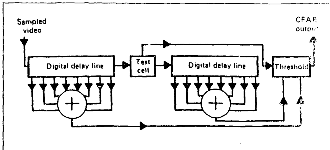
Figure 2 Cell-averaging CFAR
