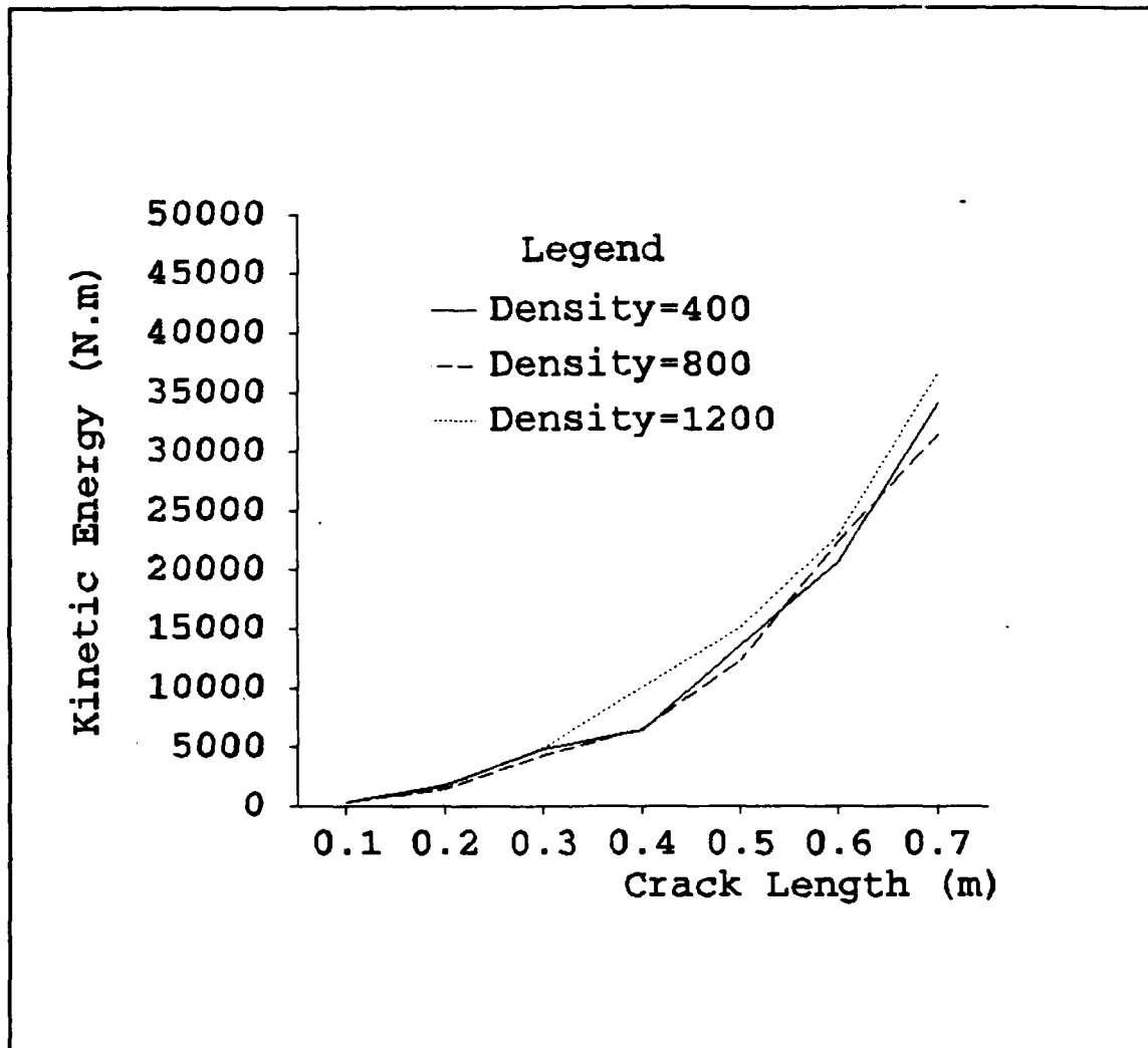
Figure 24 Kinetic Energy Variation for Different Material Densities and Fixed Elastic Modulus Ratio and Crack Velocity
