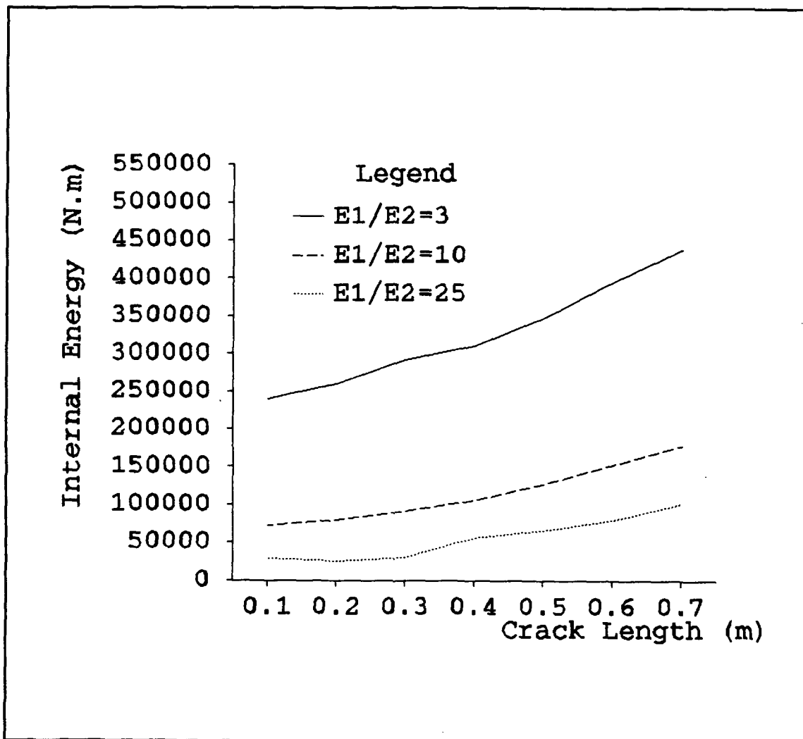
Figure 9 Internal Energy Variation for Different Elastic Modulus Ratios and Fixed Crack Velocity and Material Density
