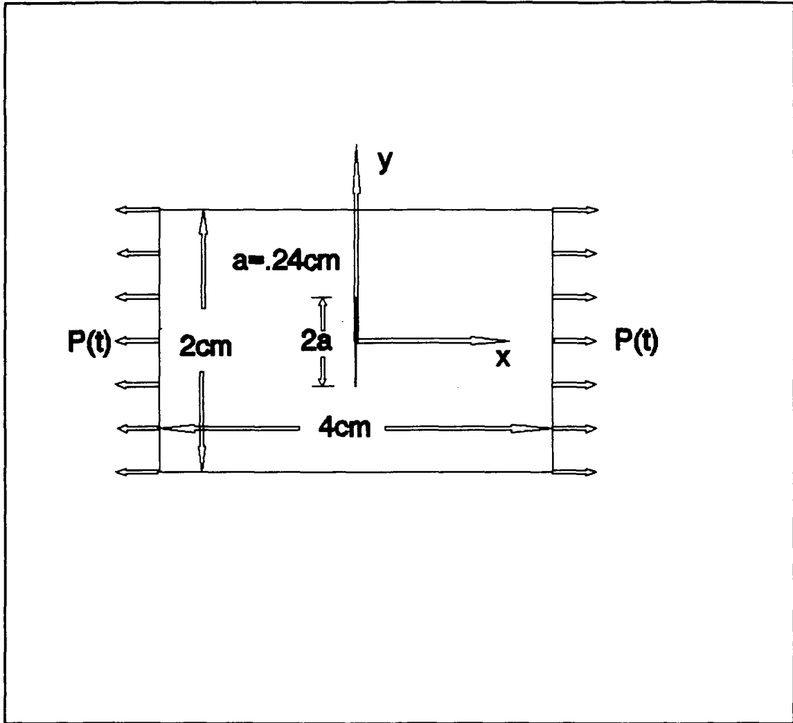
Figure 3 The Geometry of the Stationary Crack Problem
