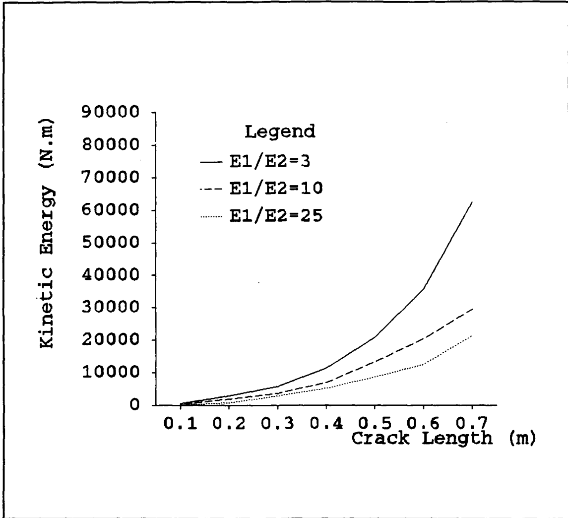
Figure 10 Kinetic Energy Variation for Different Elastic Modulus Ratios and Fixed Crack Velocity and Material Density
