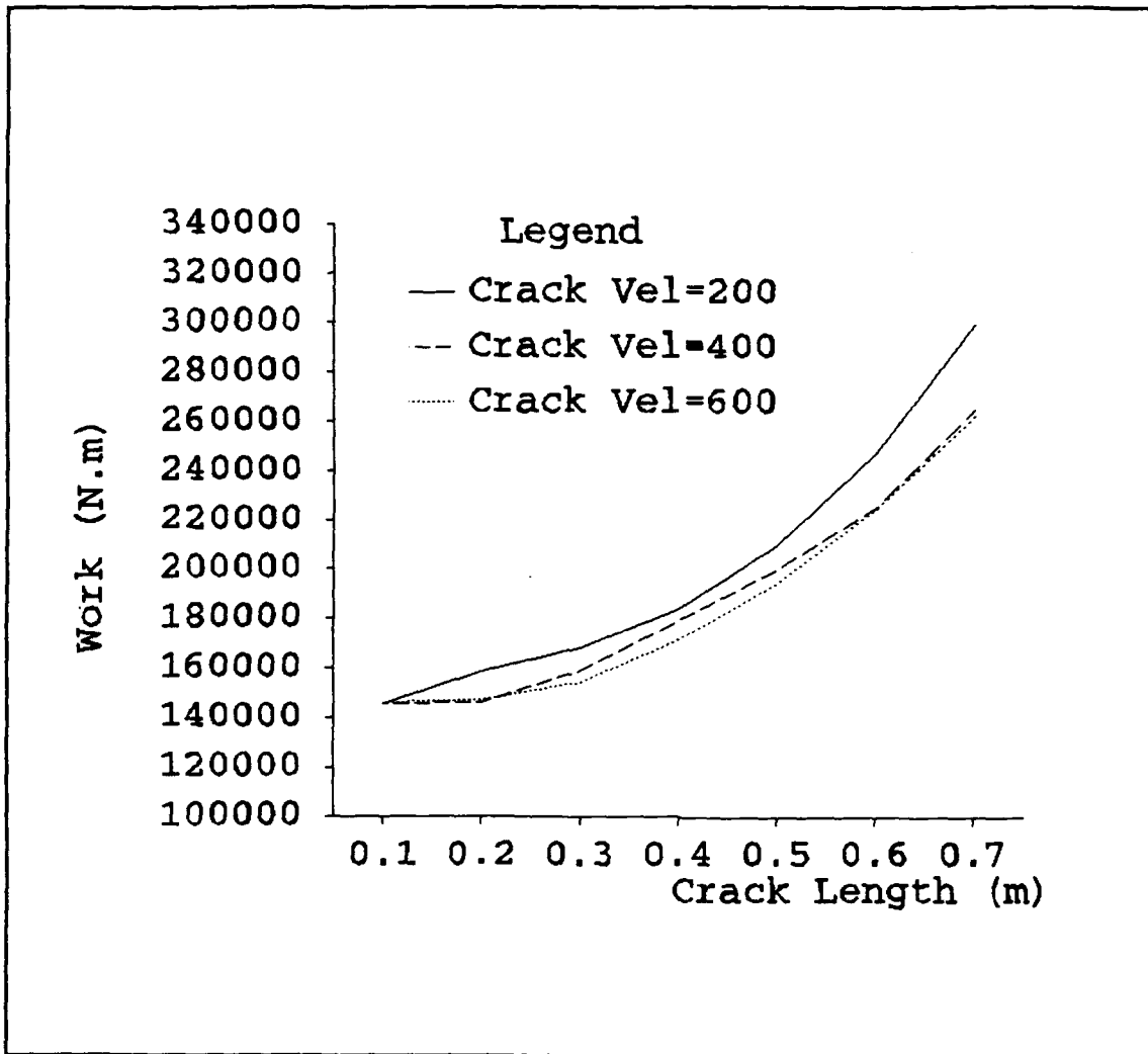
Figure 13 Work Variation for Different Crack Velocities and Fixed Elastic Modulus Ratio and Material Density
