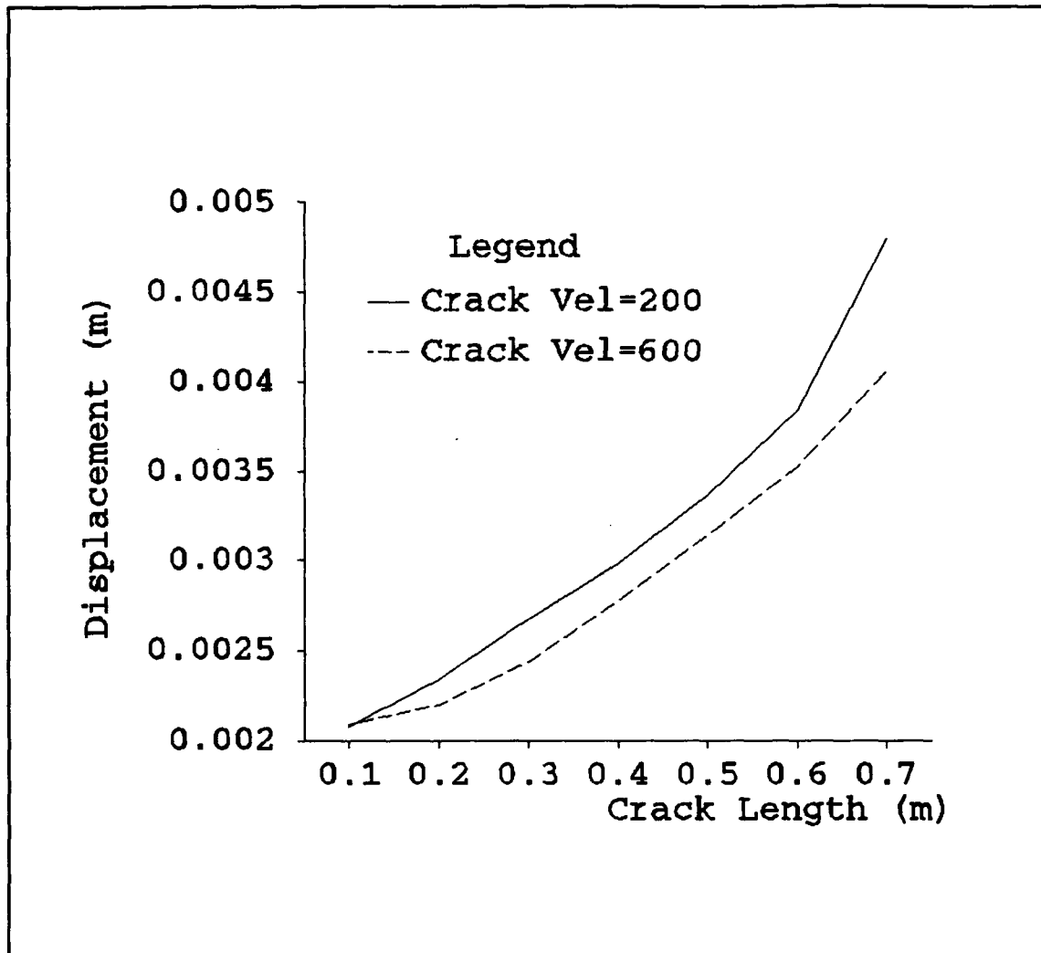
Figure 15 Displacement Values for Different Crack Velocities and Fixed Elastic Modulus Ratio and Material Density
