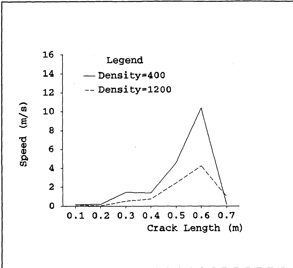
Figure 23 Speed Values for Different Material Densities and Fixed Elastic Modulus Ratio and Crack Velocity
