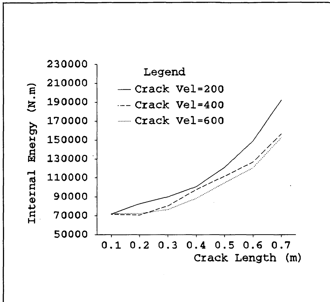
Figure 14 Internal Energy Variation for Different Crack Velocities and Fixed Elastic Modulus Ratio and Material Density
