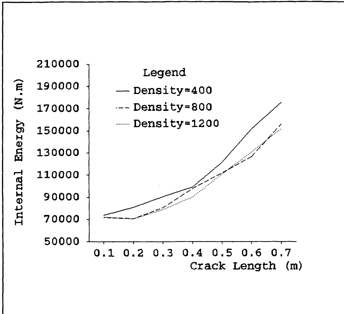
Figure 21 Internal Energy Variation for Different Material Densities and Fixed Elastic Modulus Ratio and Crack Velocity
