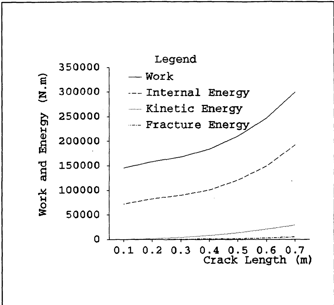
Figure 7 Work and Energy Variation During a Crack Propagation
