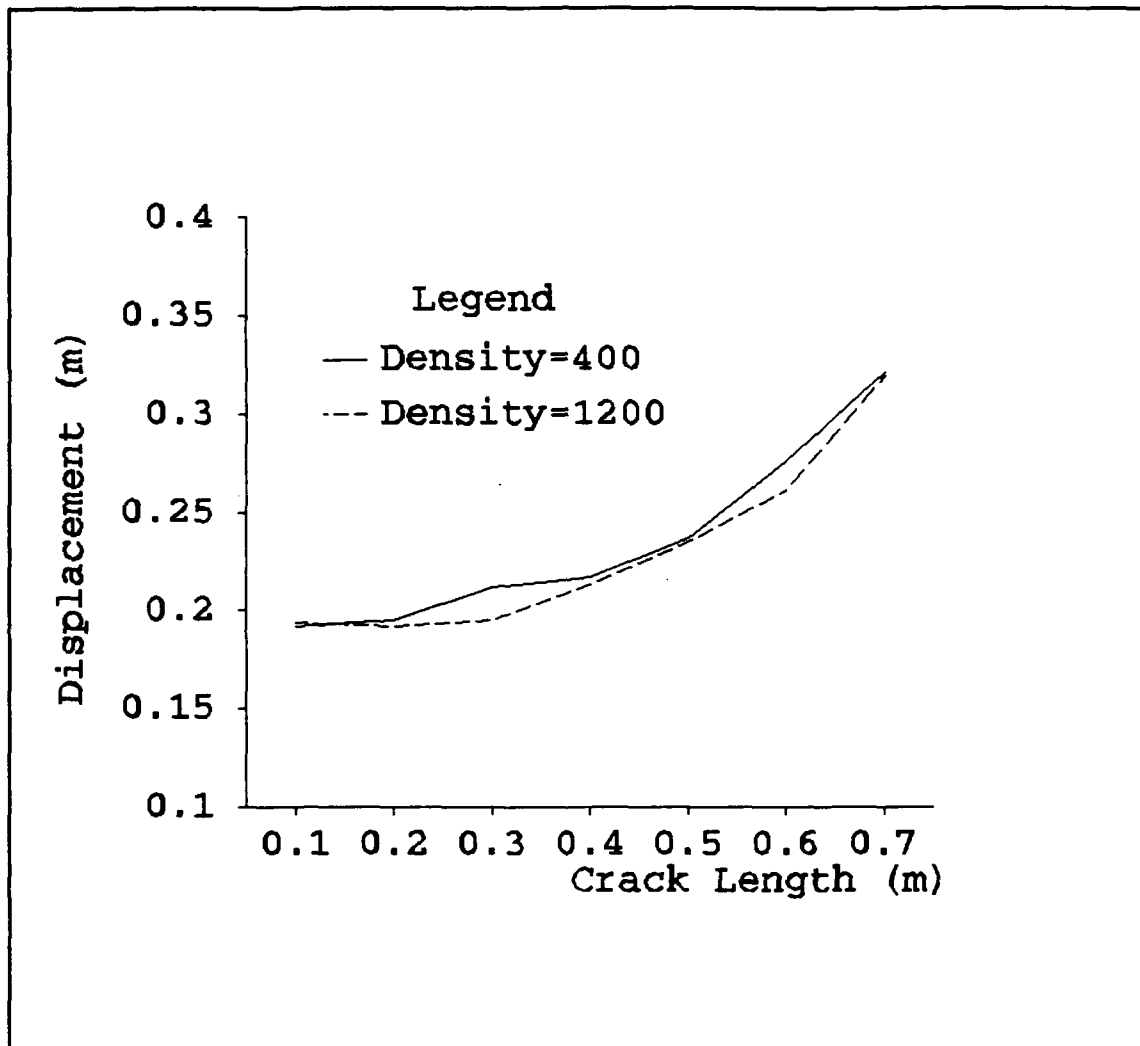
Figure 22 Displacement Values for Different Material Densities and Fixed Elastic Modulus Ratio and Crack Velocity
