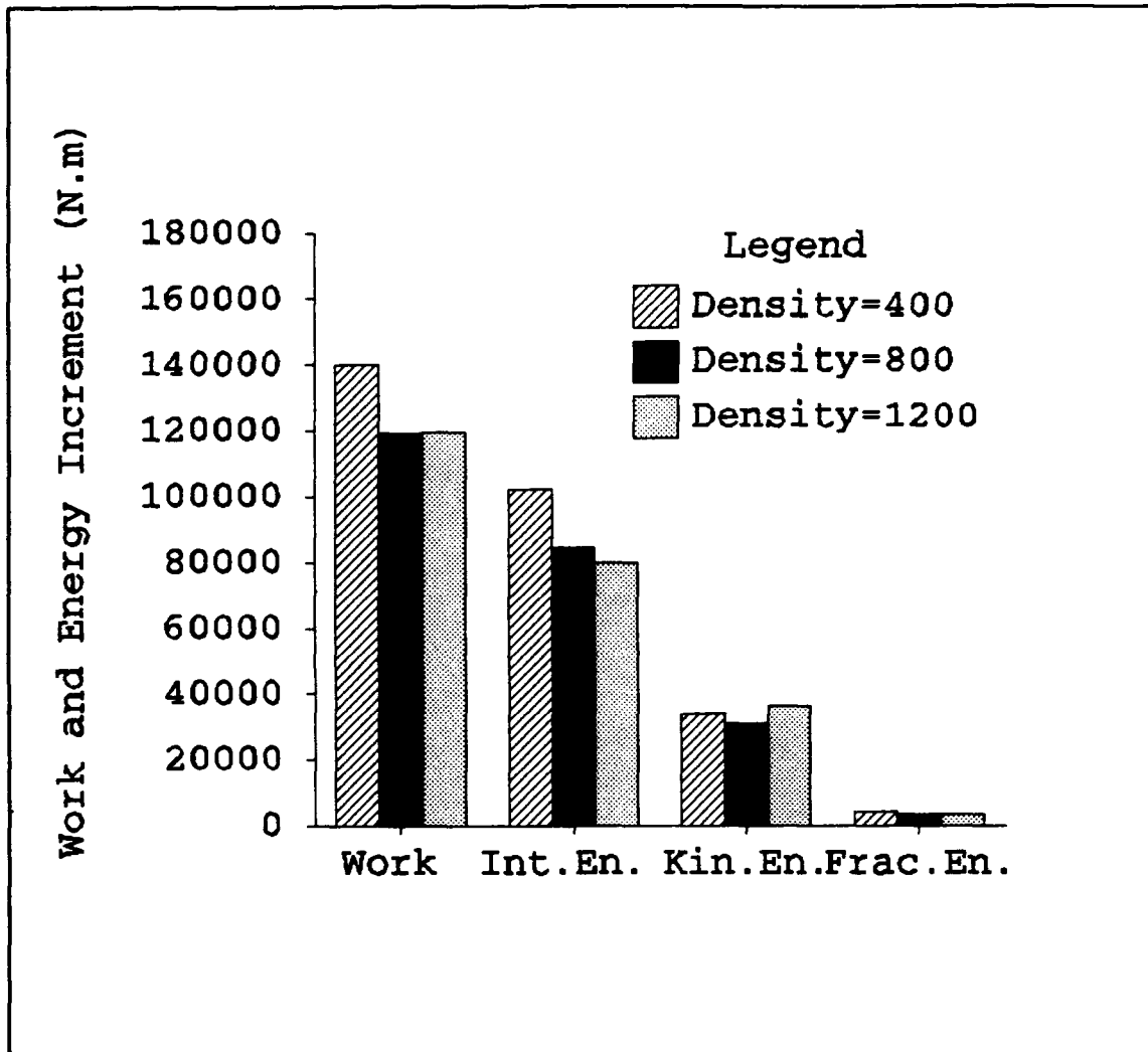
Figure 26 Work and Energy Differences Between the Initial Time and a Late Time for Different Material Densities and Fixed Elastic Modulus Ratio and Crack Velocity
