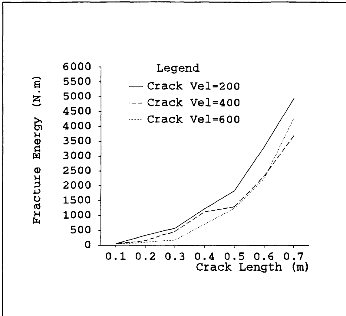
Figure 18 Fracture Energy Variation for Different Crack Velocities and Fixed Elastic Modulus Ratio and Material Density
