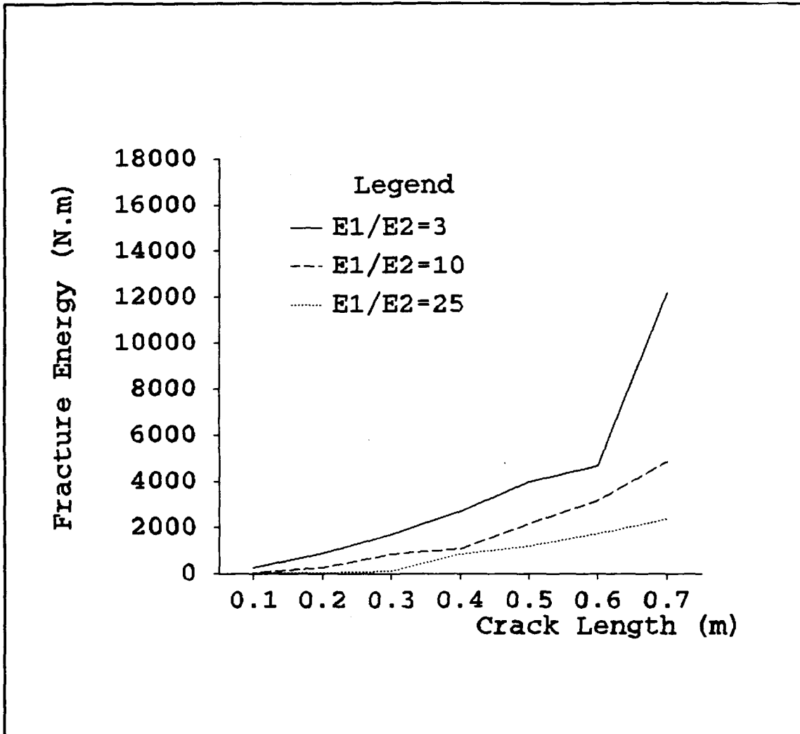
Figure 11 Fracture Energy Variation for Different Elastic Modulus Ratios and Fixed Crack Velocity and Material Density
