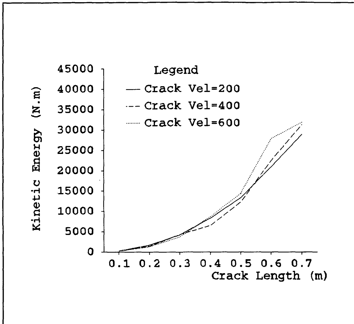
Figure 16 Kinetic Energy Variation for Different Crack Velocities and Fixed Elastic Modulus Ratio and Material Density
