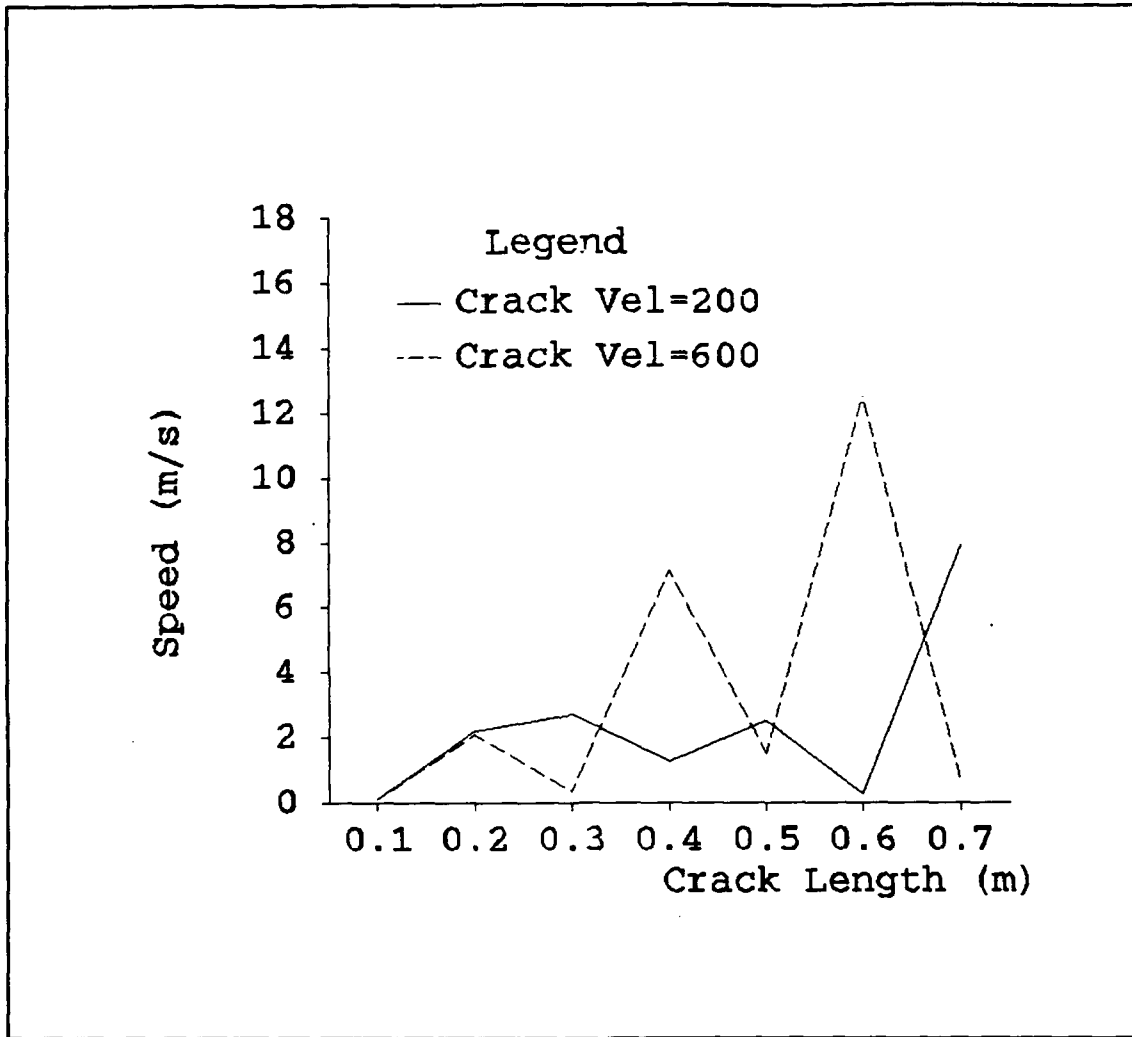
Figure 17 Speed Values for Different Crack Velocities and Fixed Elastic Modulus Ratio and Material Density
