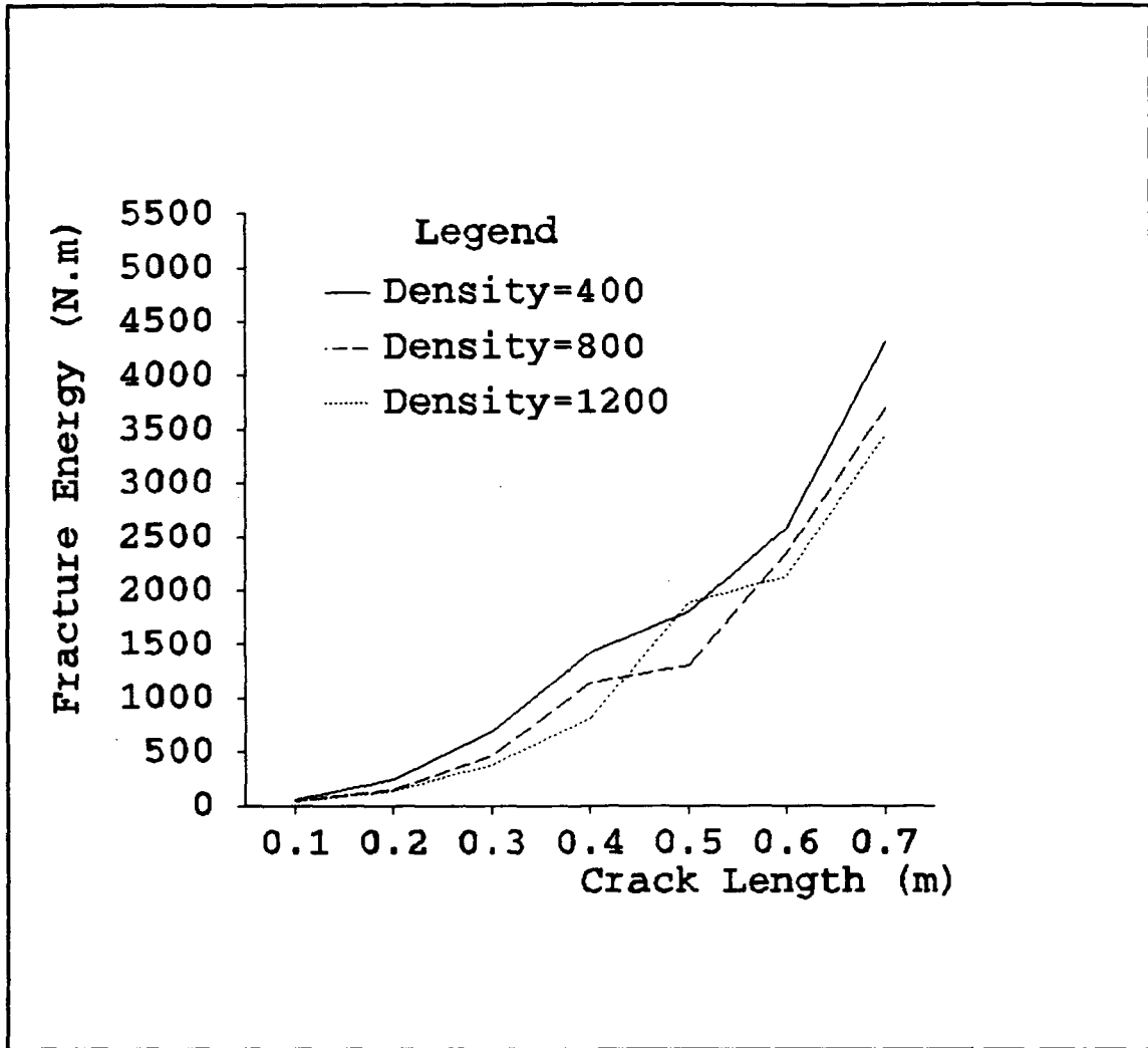
Figure 25 Fracture Energy Variation for Different Material Densities and Fixed Elastic Modulus Ratio and Crack Velocity
