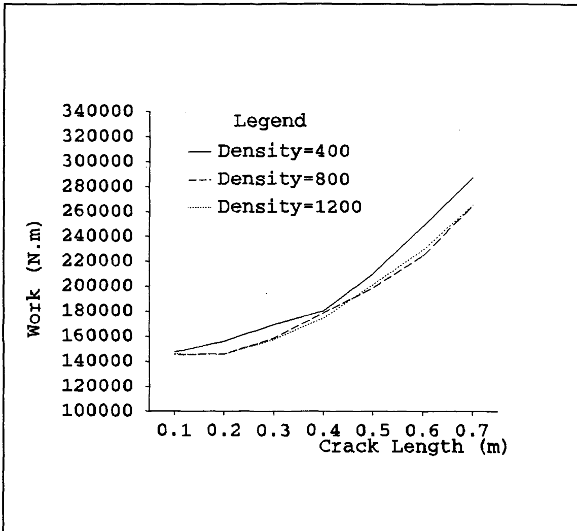
Figure 20 Work Variation for Different Material Densities and Fixed Elastic Modulus Ratio and Crack Velocity
