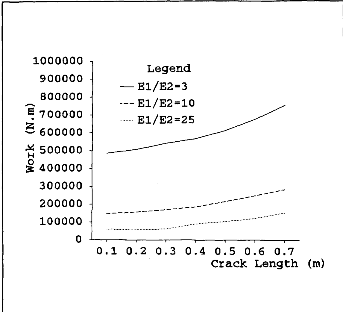
Figure 8 Work Variation for Different Elastic Modulus Ratios and Fixed Crack Velocity and Material Density
