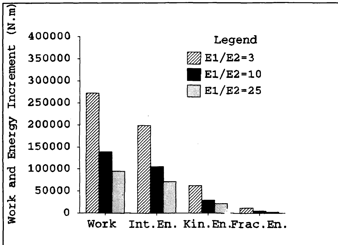
Figure 12 Work and Energy Differences Between the Initial Time and a Late Time for Different Elastic Modulus Ratios and Fixed Crack Velocity and Material Density
