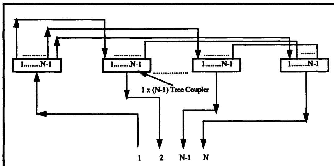
Figure 3. Schematic of Modified Star Coupler
