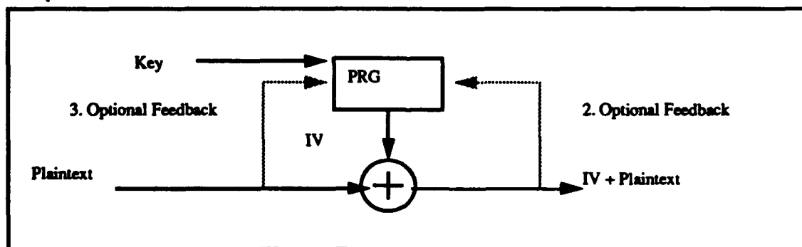
Figure 18. Stream Cipher Variations
