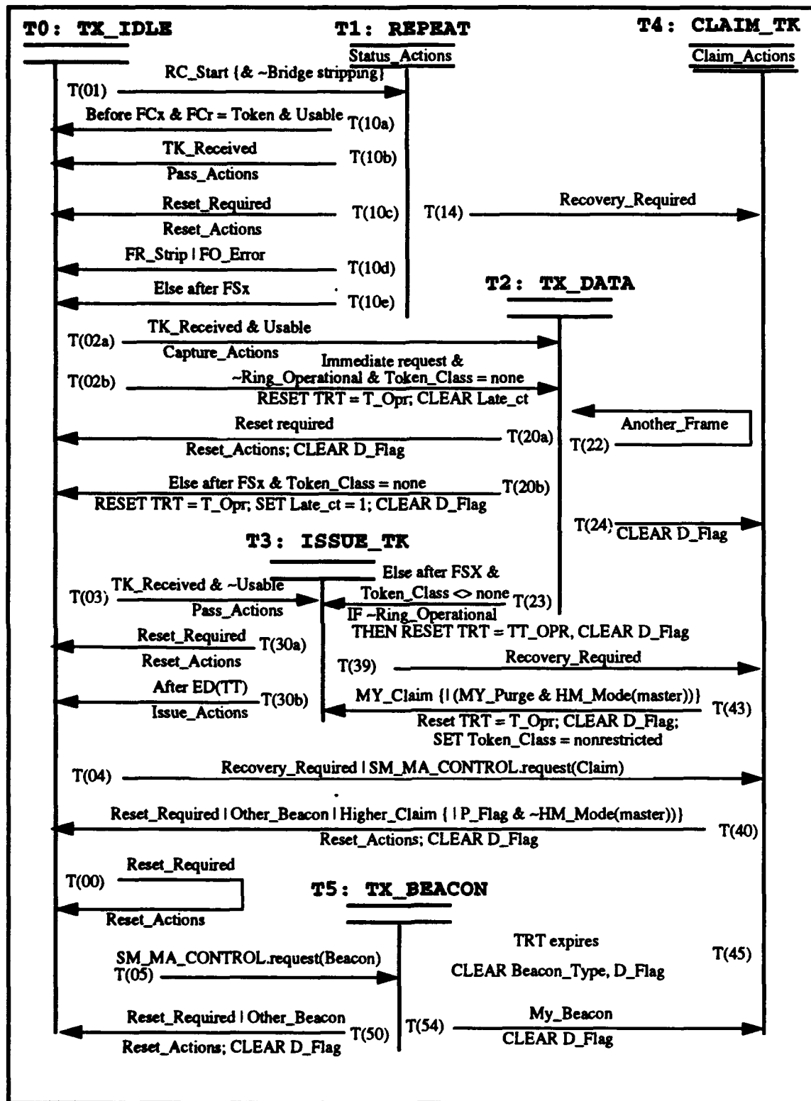
Figure 16. MAC Transmitter State Diagram
