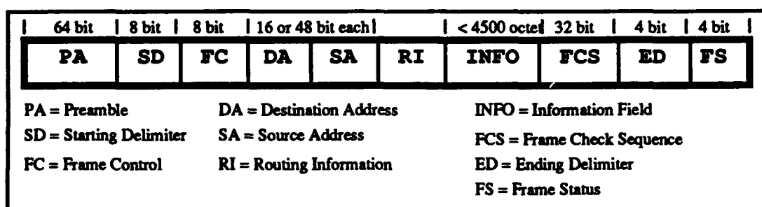
Figure 6. FDDI Frame
