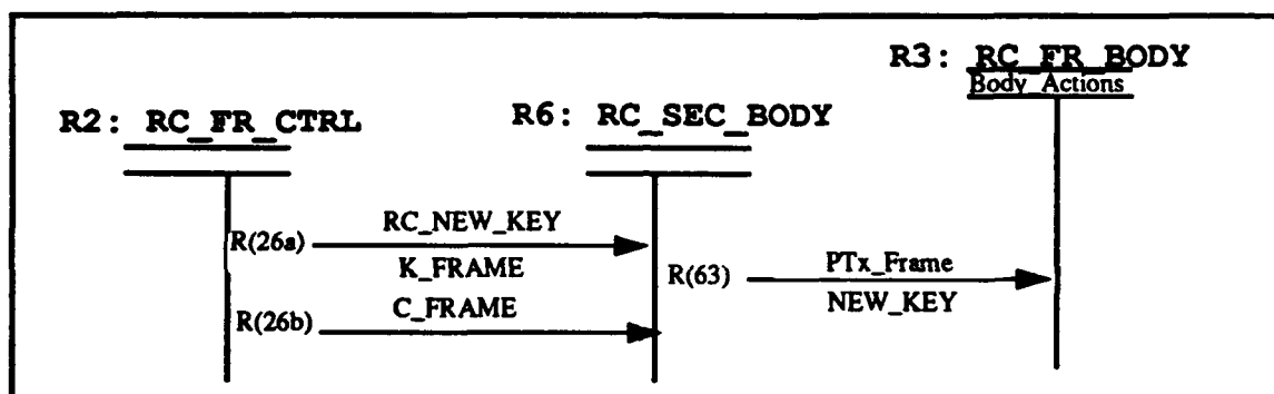
Figure 13. Modified MAC Receiver State Diagram (States Affected)
