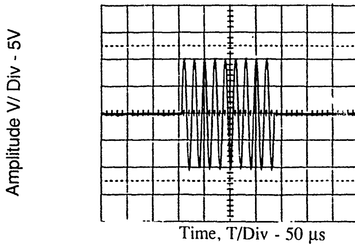
Figure 3.2 Input pulse
