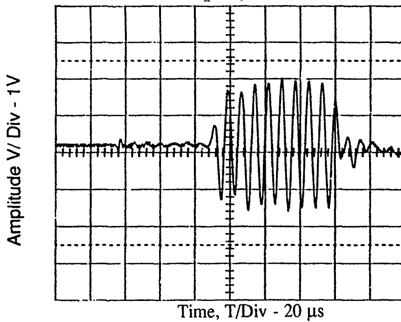
Figure 3.12 Delay of extensional mode due to transducer switch, [0,90]_{4,s} laminate ,130 kHz, B/C transducer combination.
