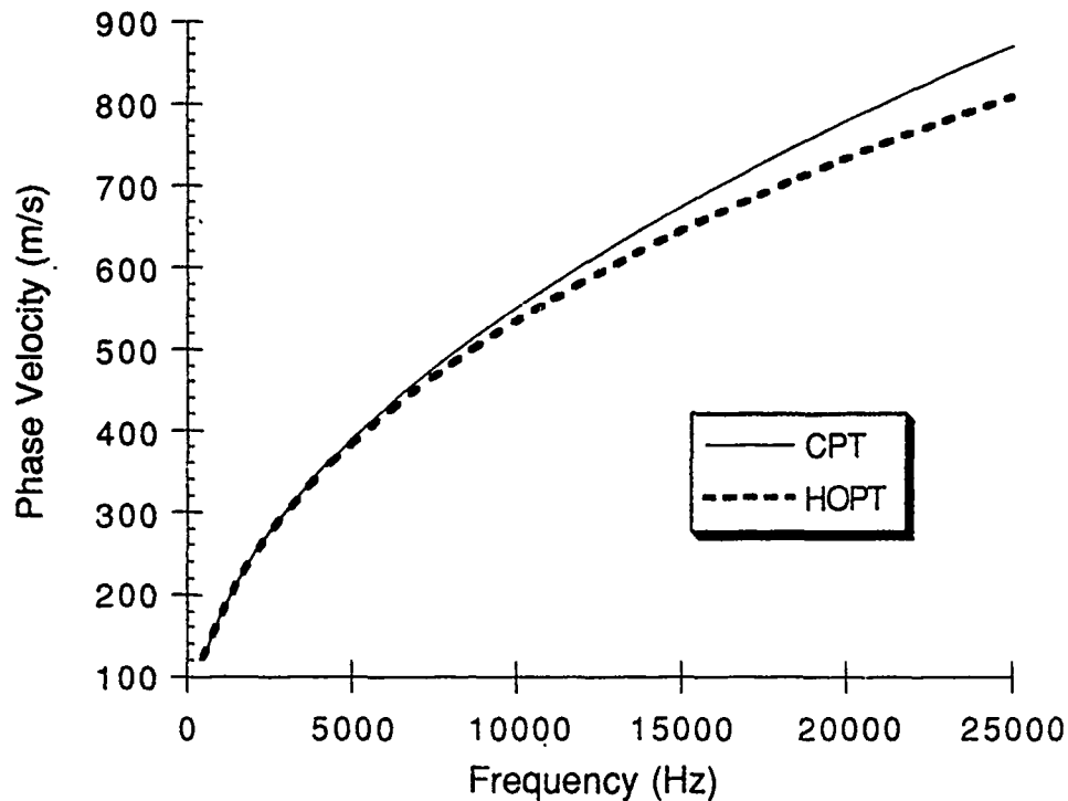
Figure 4.3 CPT vs. HOPT [0,45,90,-45] 2,s laminate, 0° direction
