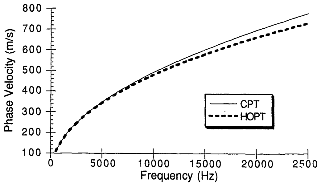
Figure 4.4 CPT vs. HOPT, [0,45,90,-45]_{2,s} laminate , 90^\circ direction
