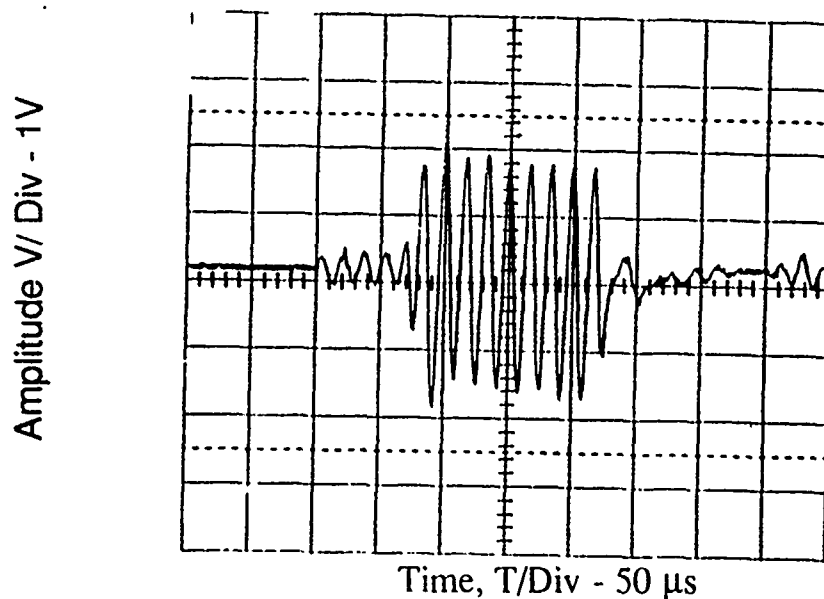
Figure 3.10 Reference wave form , [0,90]_4 s laminate, (frequency= 60kHz)
