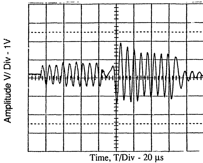
Figure 3.11 Extensional and flexural wave excitation, [0,90]_{4,s} laminate, (frequency= 130 kHz), A/B Transducer Combination
