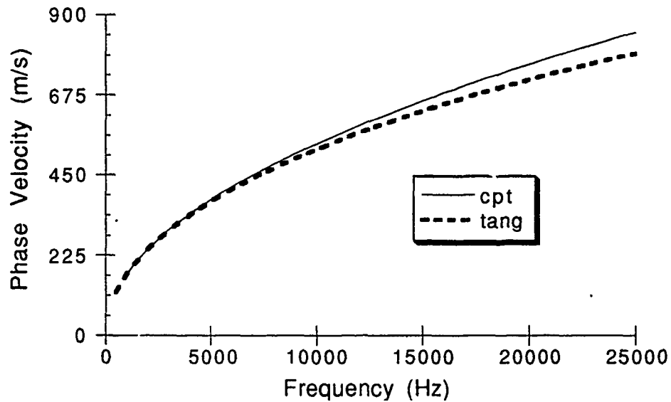
Figure 4.6 CPT vs. HOPT , [0,90]_{4,s} laminate , 90° direction
