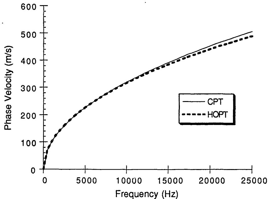
Figure 4.2 CPT vs. HOPT [0]_{16} laminate , 90° direction
