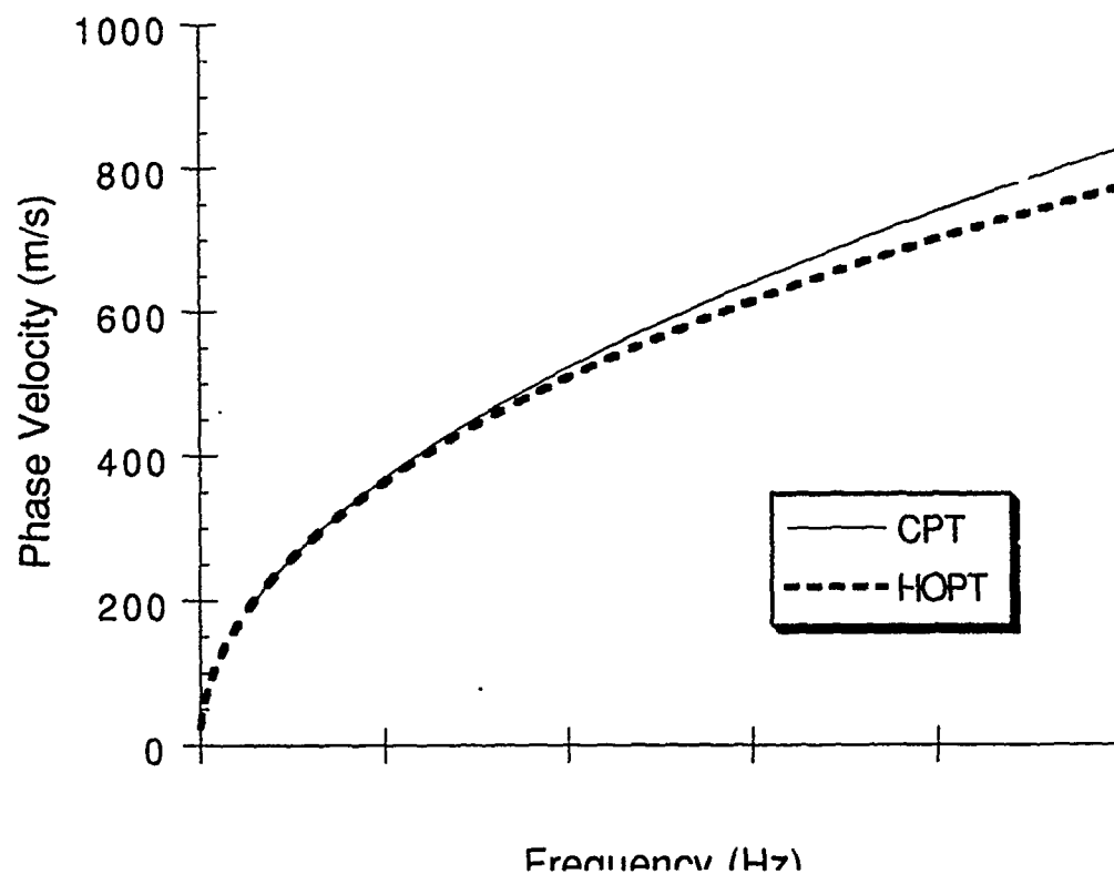
Figure 4.5 CPT vs. HOPT [0,90]_{4,s} laminate , 0^\circ direction
