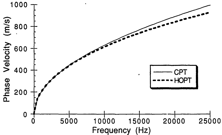
Figure 4.1 CPT vs. HOPT [0]_{16} laminate, 0^\circ direction.
