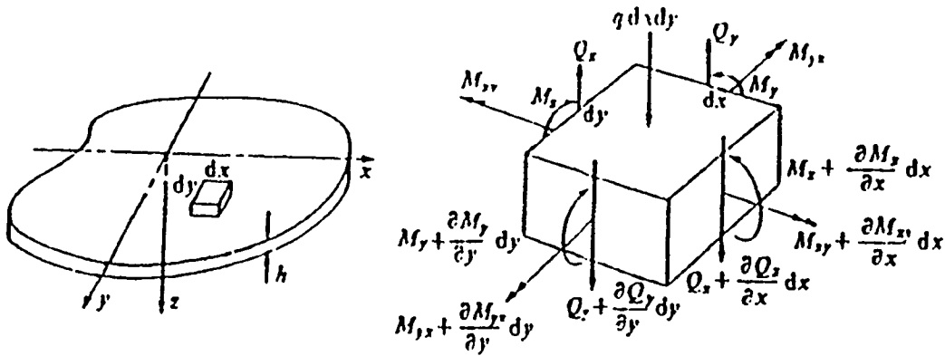
Figure 2.1 Plate Element (after Graff [Ref. 13]).
