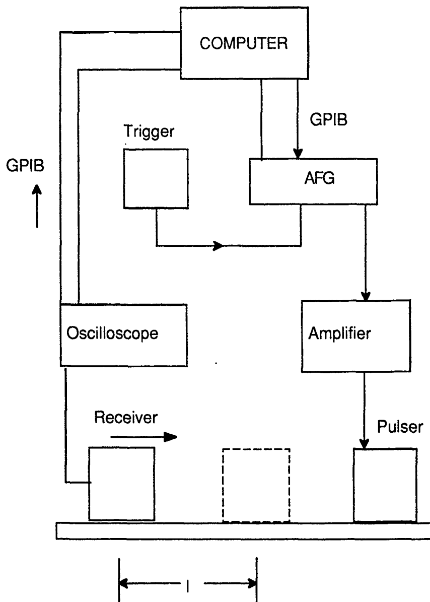
Figure 3.1 Schematic of Experimental Set-up
