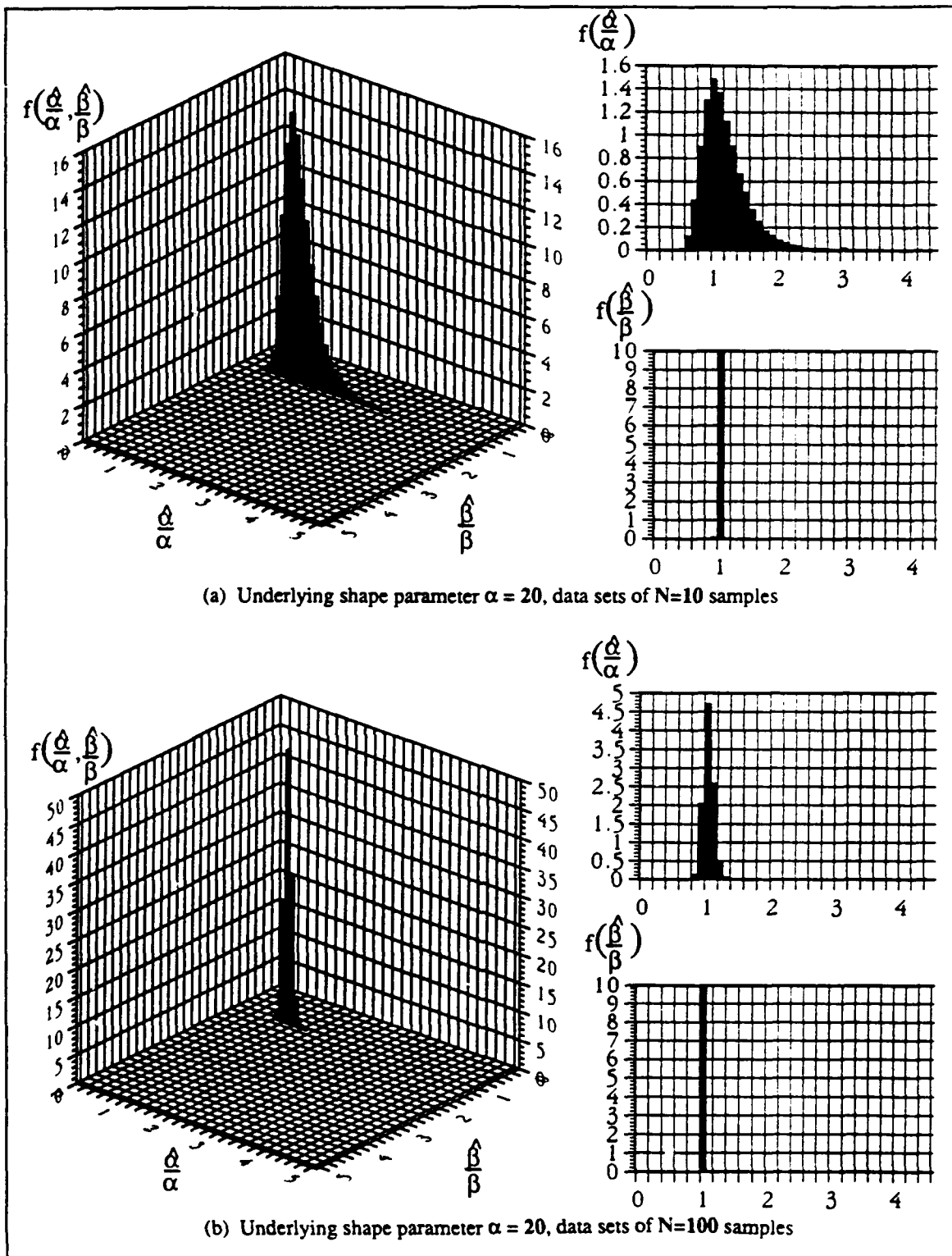
FIGURE 3.8 JOINT HISTOGRAM AND MARGINAL DISTRIBUTIONS OF THE ESTIMATED PARAMETERS FOR \alpha=20
