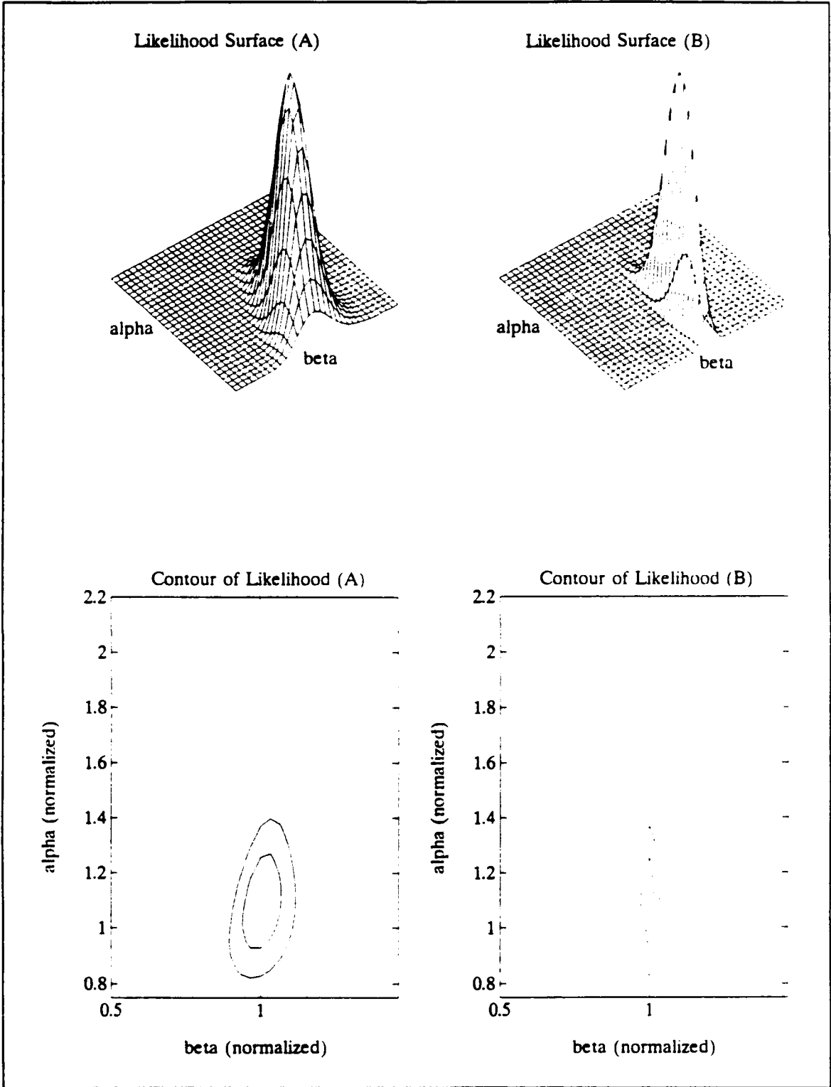
FIGURE B.1 LIKELIHOOD SURFACES AND CONTOUR PLOTS FOR TWO DATA SETS
