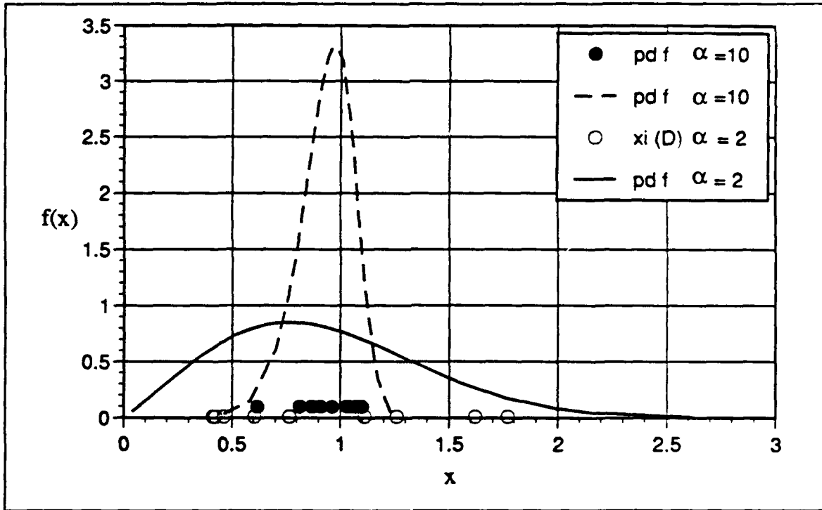
FIGURE 3.3 GRAPH OF THE PDF F(X) FOR TWO DATA SETS
