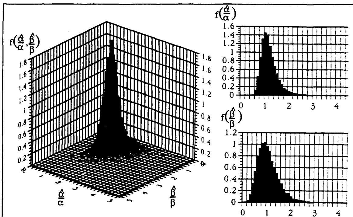
(a) Underlying shape parameter \alpha = 0.8 , data sets of N=10 samples
