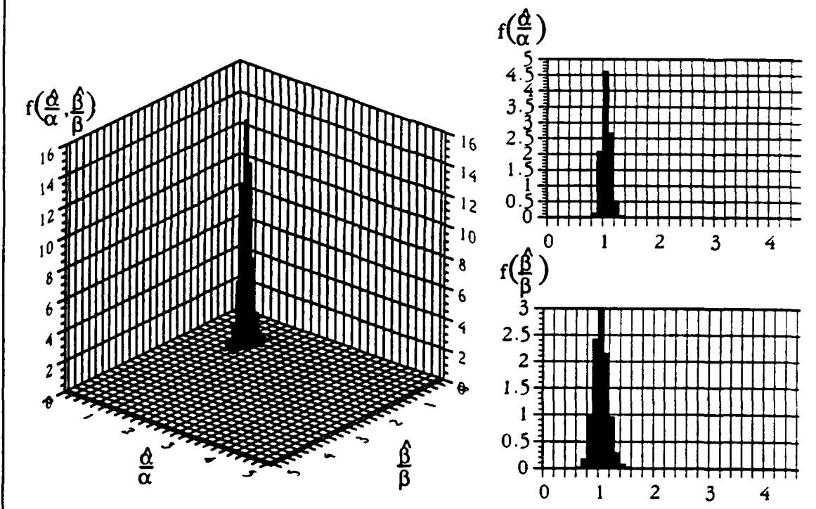
(b) Underlying shape parameter \alpha = 0.8 , data sets of N=100 samples
