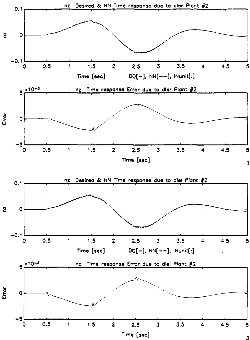
Figure B.36: Normal Acceleration Response Damaged Aircraft Due to Leading Edge Flaps Dipole Command, Multiple-Plant, Single Network Emulation
