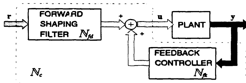
Figure 5.7: Control Architecture
