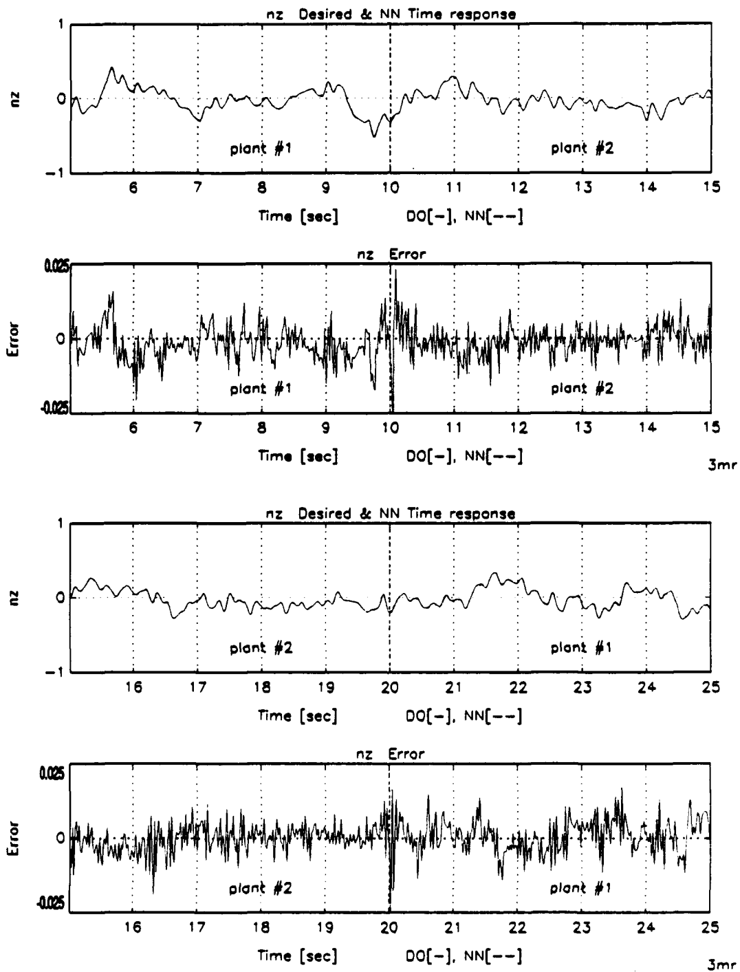
Figure 8.18: Normal Acceleration Response of a Minimally Realized Single Network Emulating Two Plants Due to RBS Excitation of All Inputs
