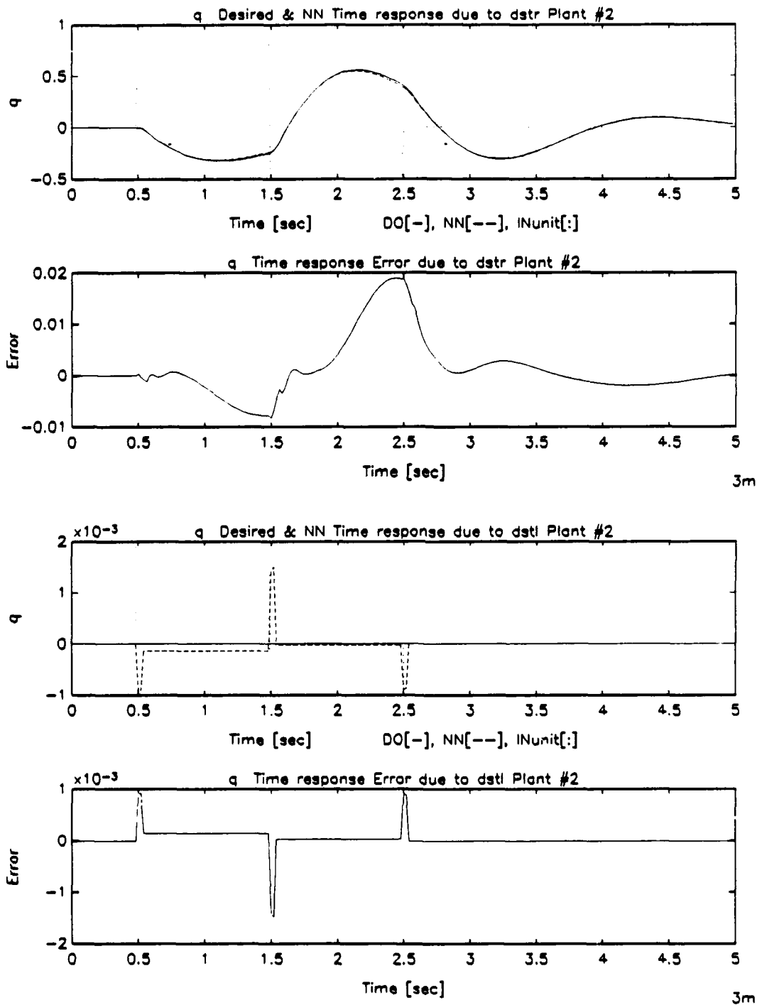
Figure B.55: Pitch Rate Response of Damaged Aircraft Due to Stabilizers Dipole Command, Multiple-Plant, Minimized Network Emulation
