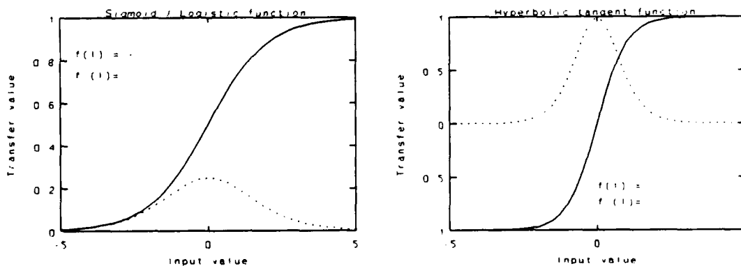
Figure 2.4: Hyperbolic Tangent and Sigmoid Activation Functions and Derivatives
