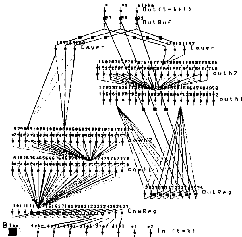
Figure 8.1: Network Structure for a Multiple-Plant F/A-18 Emulation
