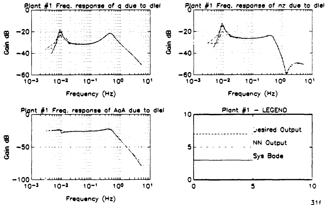
Figure B.1: Spectral Response of Undamaged Aircraft Due to Leading Edge Flaps, Single Plant, Single Network Emulation
