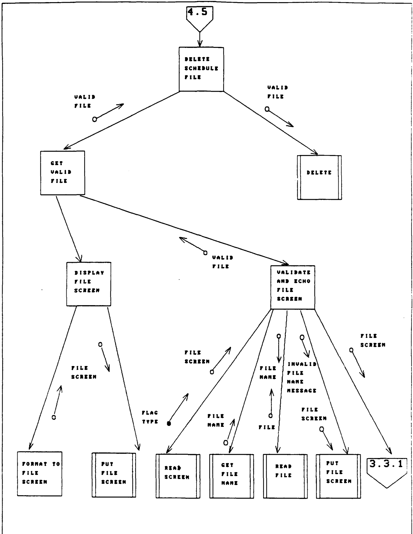
Fig. D-44, DELETE SCHEDULE FILE.
