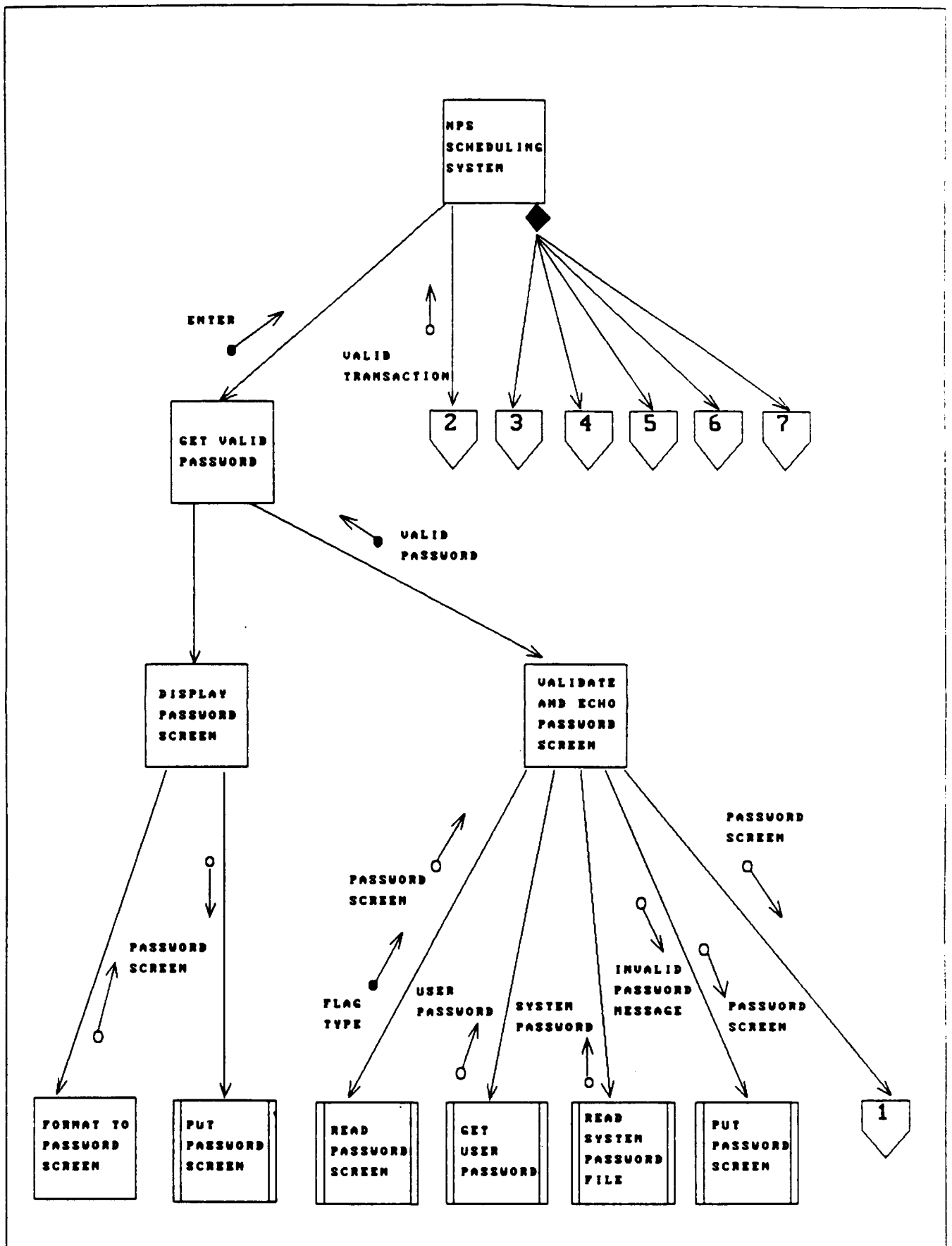
Fig. D-1, NPS SCHEDULING SYSTEM.
