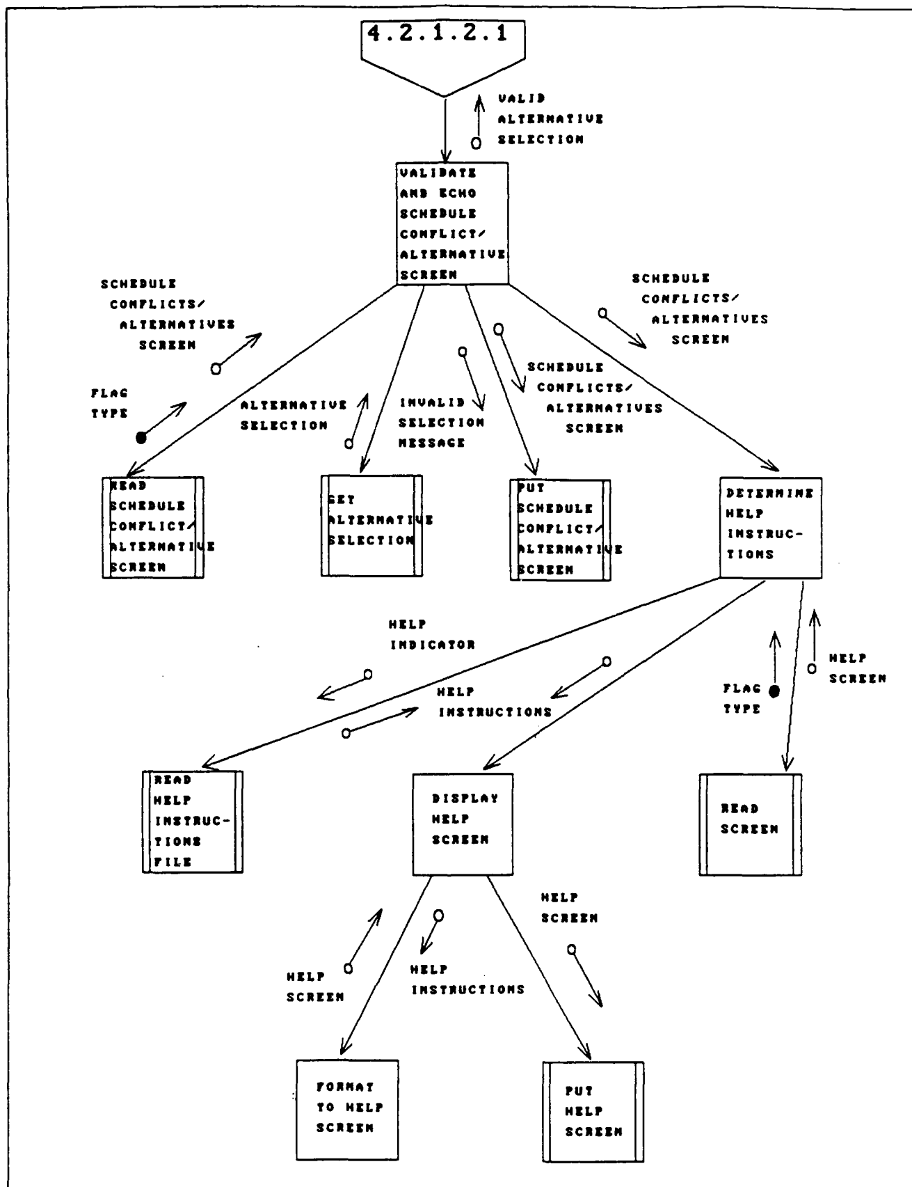
Fig. D-23, VALIDATE AND ECHO SCHEDULE CONFLICT/ALTERNATIVE SCREEN.
