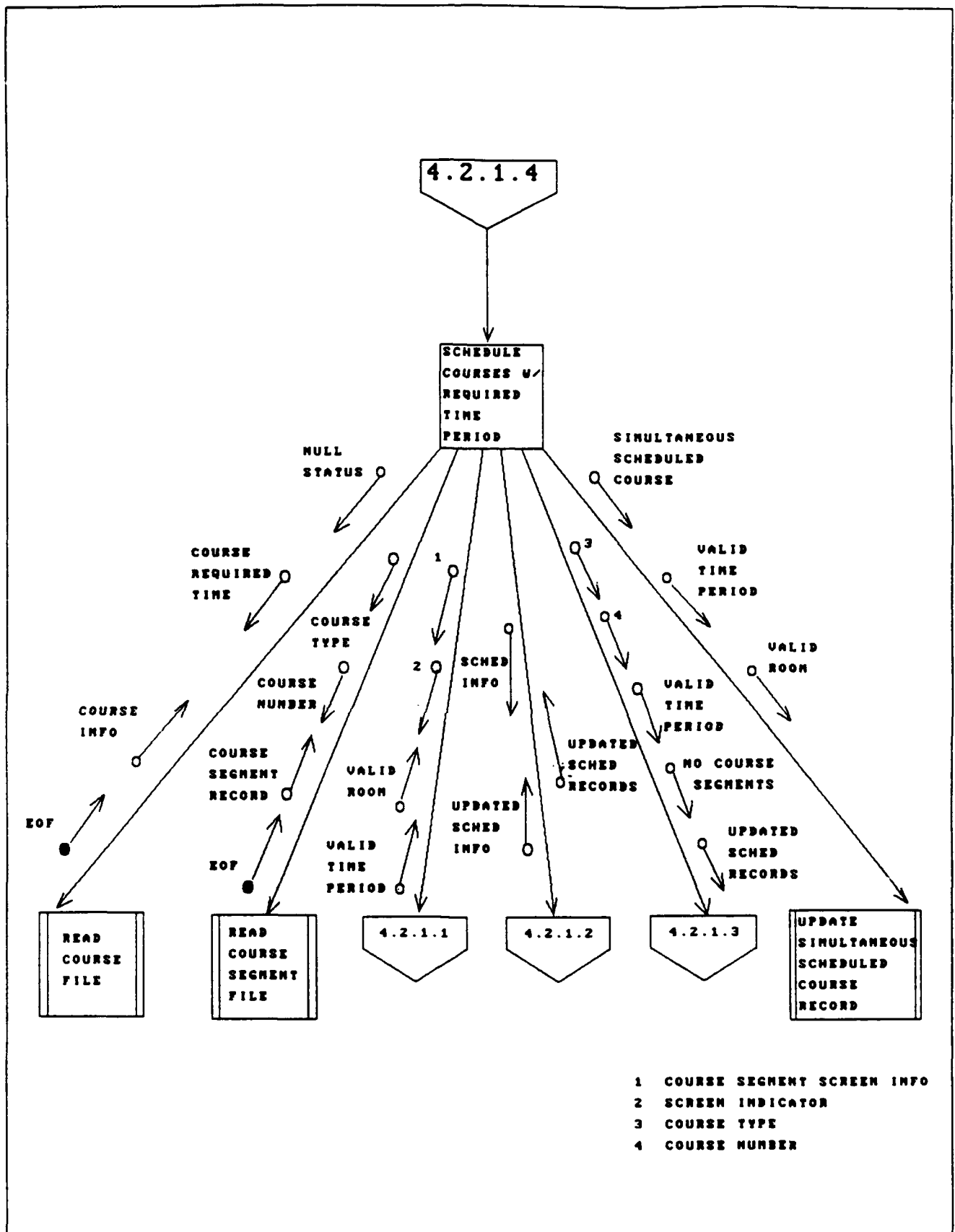
Fig. D-25, SCHEDULE COURSES W/ REQUIRED TIME PERIOD.
