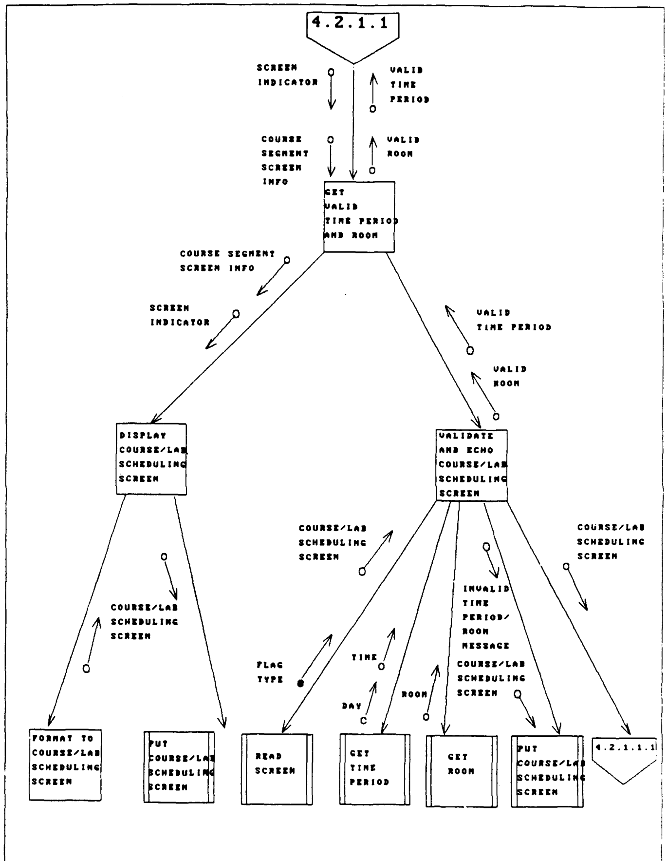
Fig. D-20, GET VALID TIME PERIOD AND ROOM.
