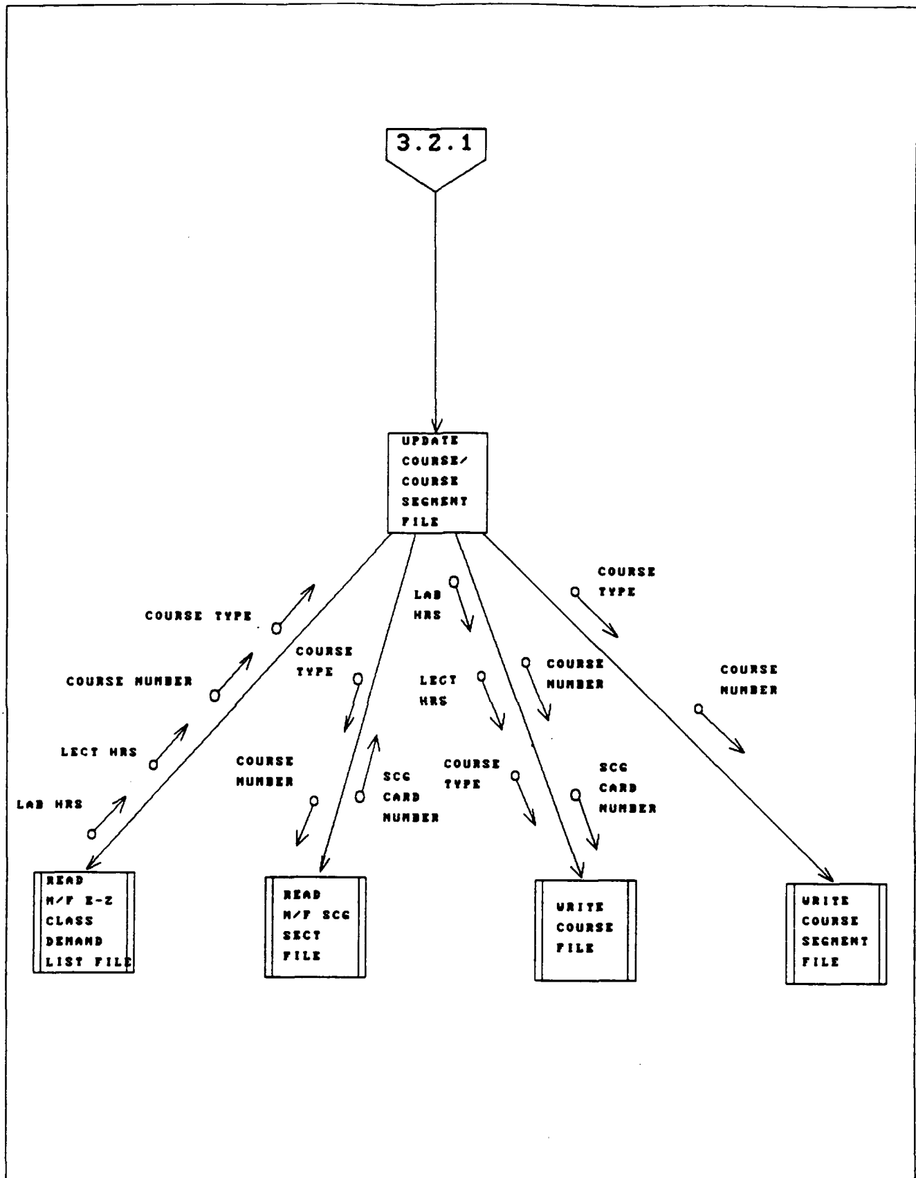
Fig. D-8, UPDATE COURSE/COURSE SEGMENT FILES.
