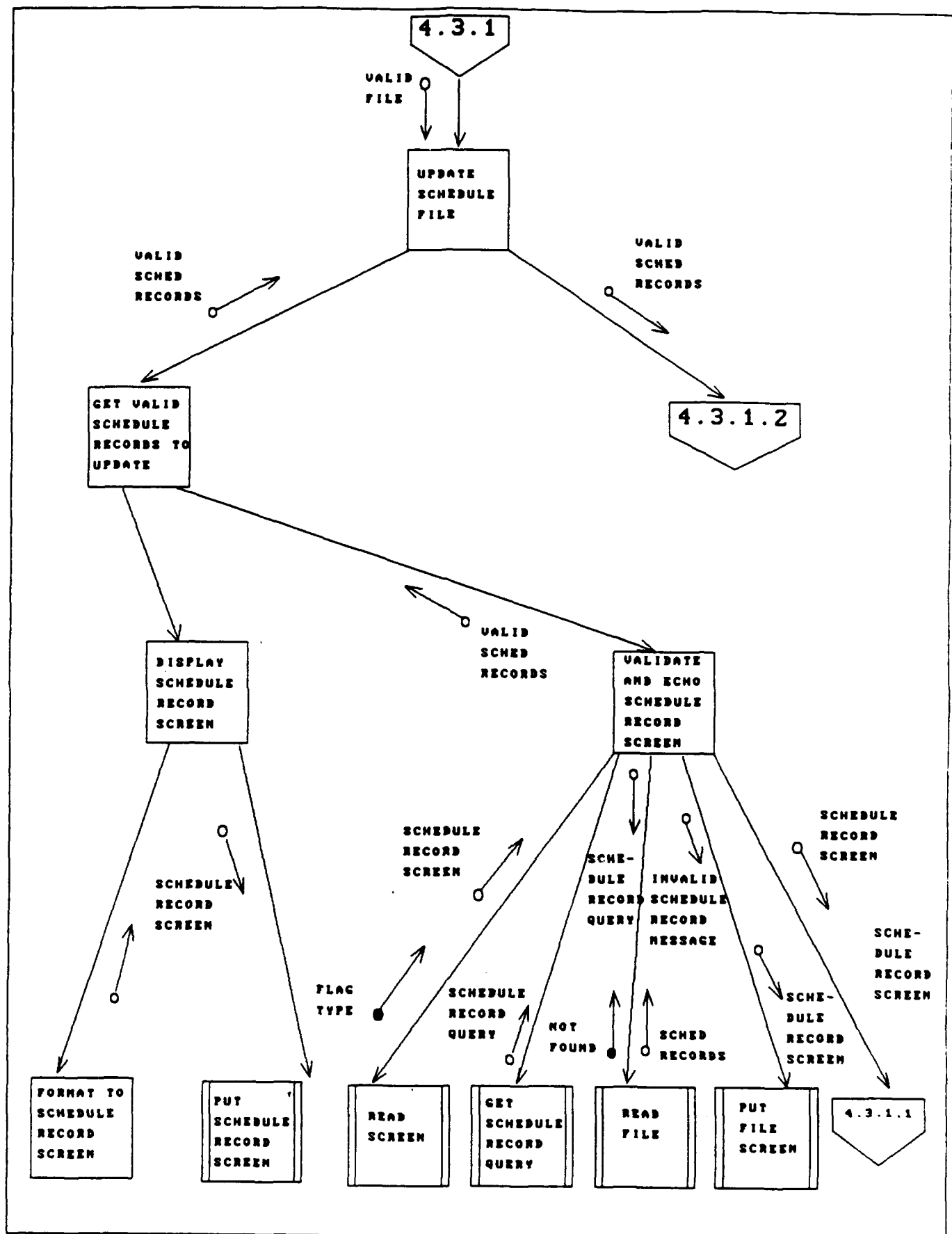
Fig. D-40, UPDATE SCHEDULE FILE.
