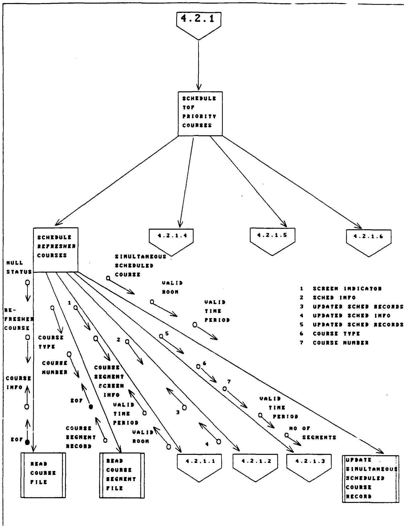
Fig. D-19, SCHEDULE TOP PRIORITY COURSES.
