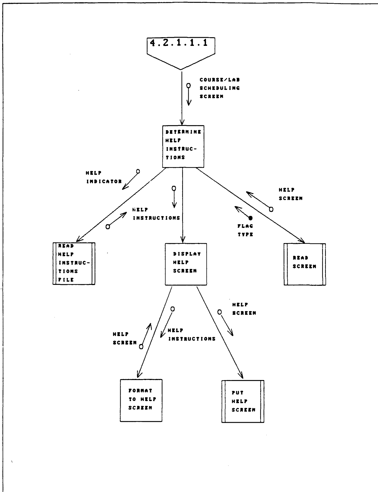
Fig. D-21. DETERMINE HELP INSTRUCTIONS for Course/Lab Scheduling Screen.
