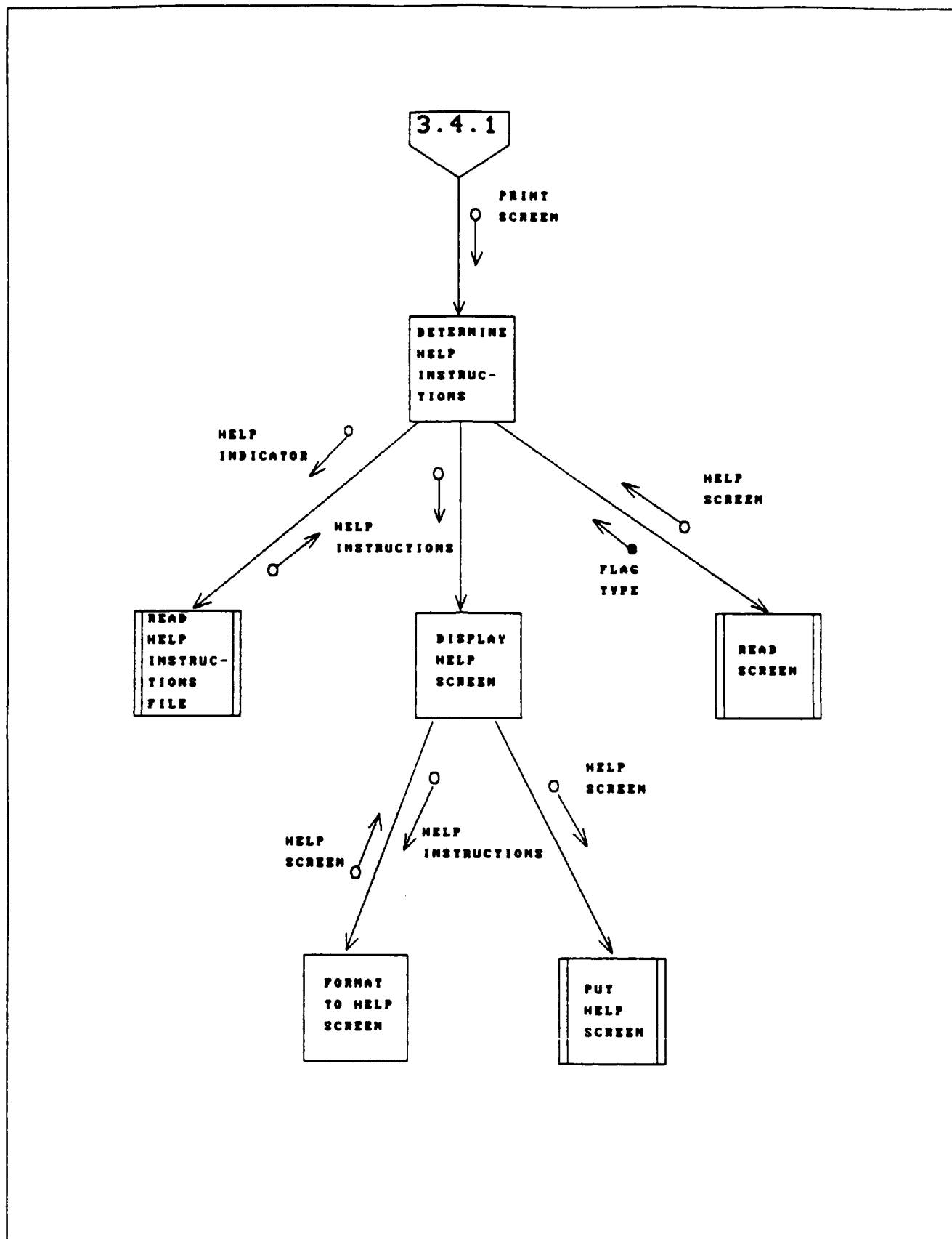
Fig. D-15, DETERMINE HELP INSTRUCTIONS for Print Screen.
