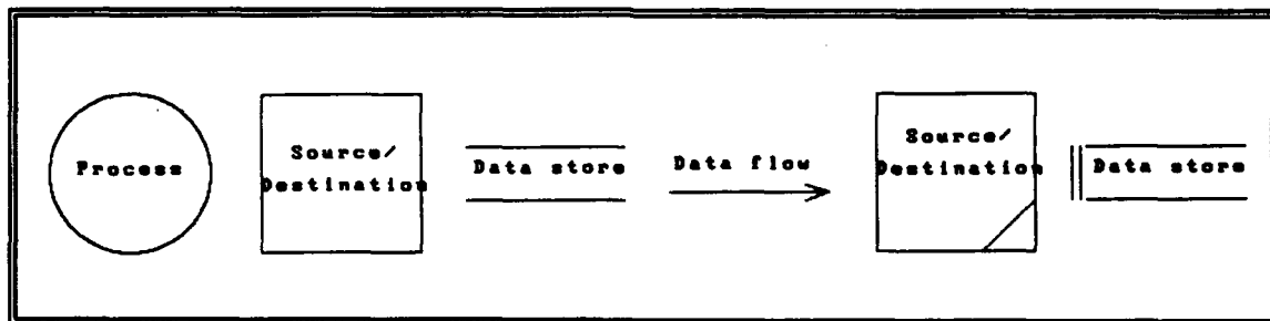
Figure 3.1 Data flow diagram notation
