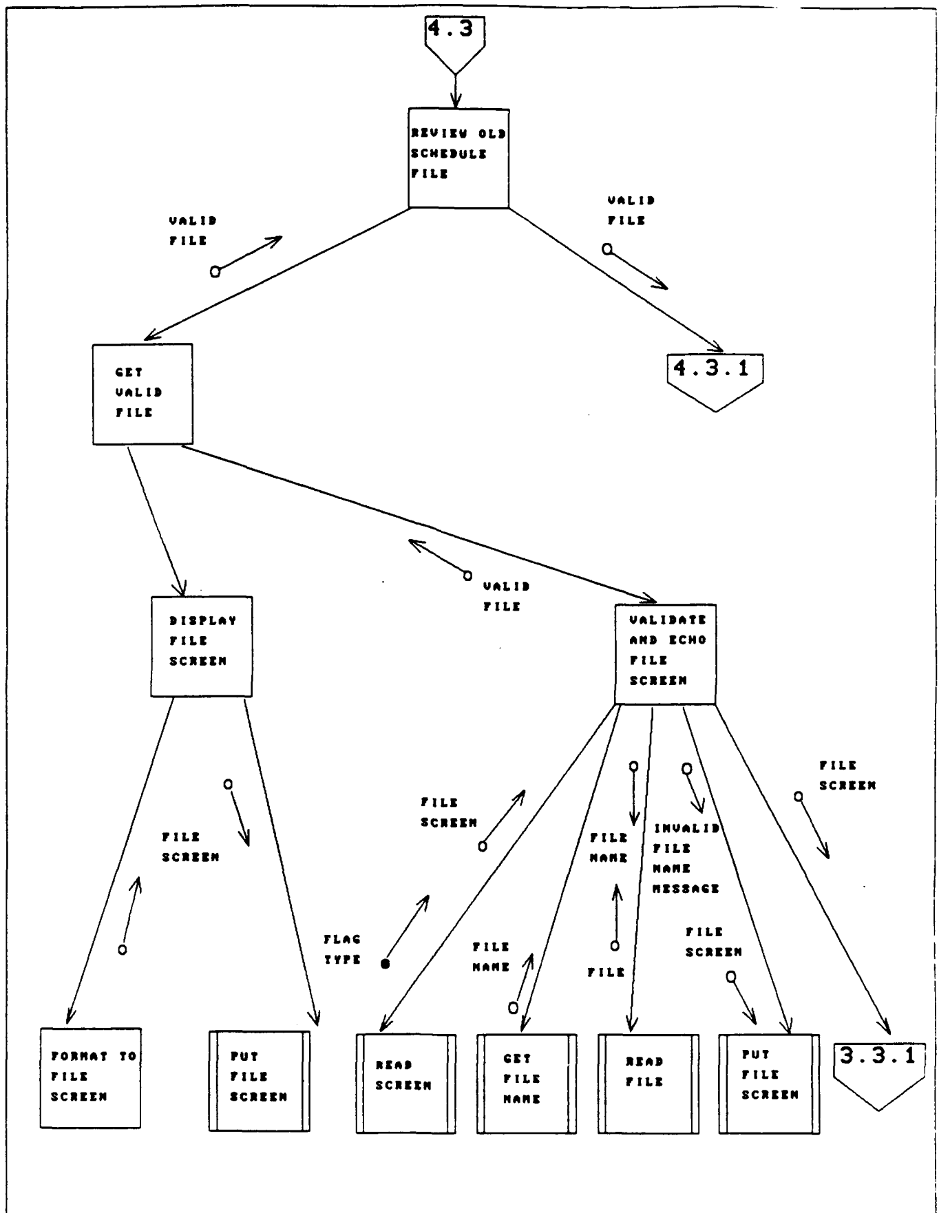
Fig. D-39, REVIEW OLD SCHEDULE FILE.
