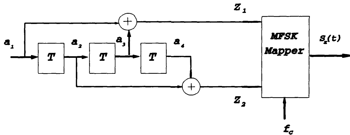
Figure 4.3 Natural Mapper for r = 1/2, v = 3, \text{TCM/4-FSK}
