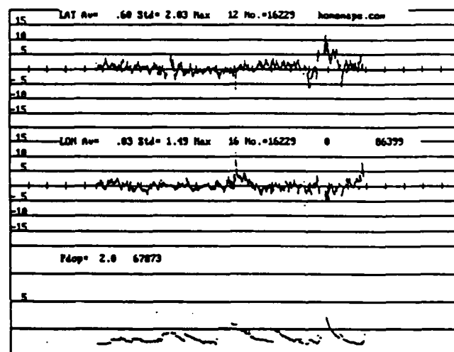
Fig 25 Multi-site DGPS Results (Meters), Day 53
