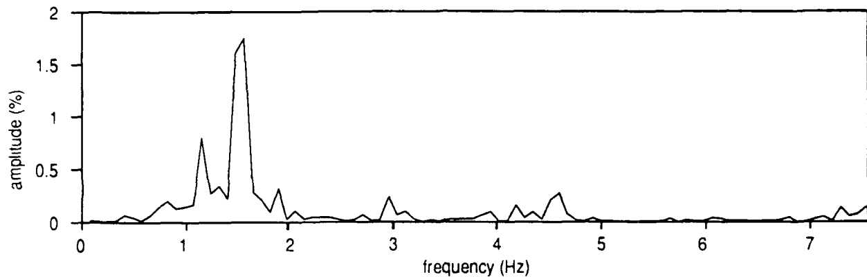
Fourier amplitude spectrum of earthquake input
