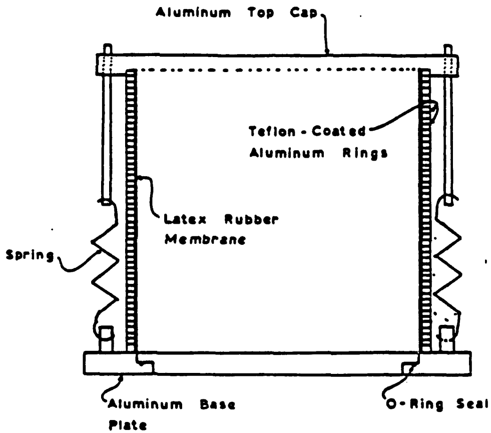
Fig. B25 The stacked ring device at MIT, Whitman et al.
