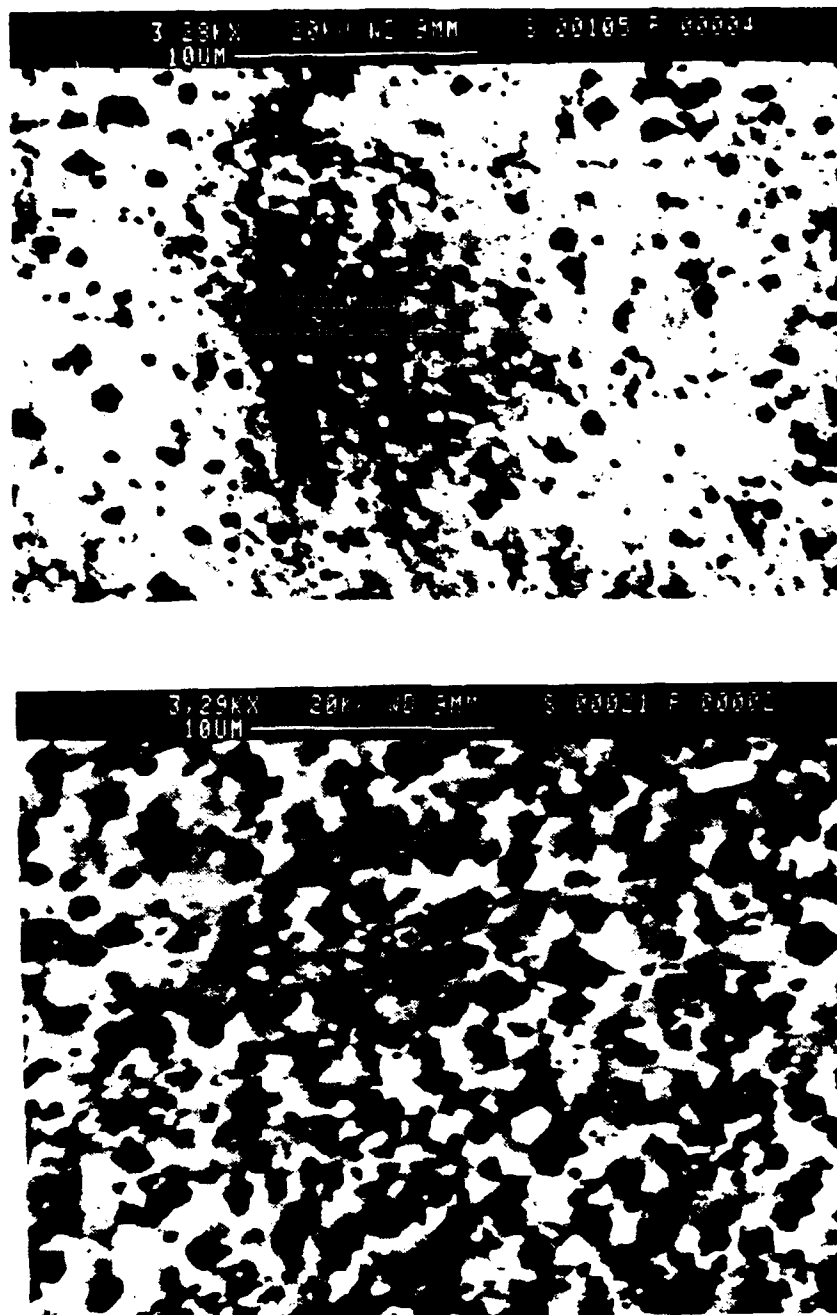
Figure 17. Electron Micrographs of TMP8 at \dot{\epsilon} = 6.11 \times 10^{-3} \text{sec}^{-1} : Interrupted tensile test specimen at a strain of \epsilon = 0.134 . Grip section shown above, gage section below.
