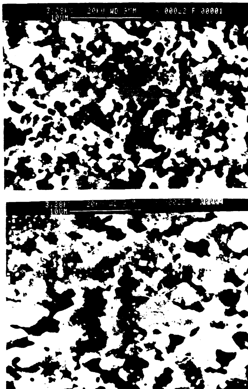
Figure 19. Electron Micrograph of TMP8 at \dot{\epsilon} = 6.11 \times 10^{-5} \text{sec}^{-1} : Tensile specimen pulled to failure. Notice large difference in grain size in the grip section (above) and the gage section (below).
