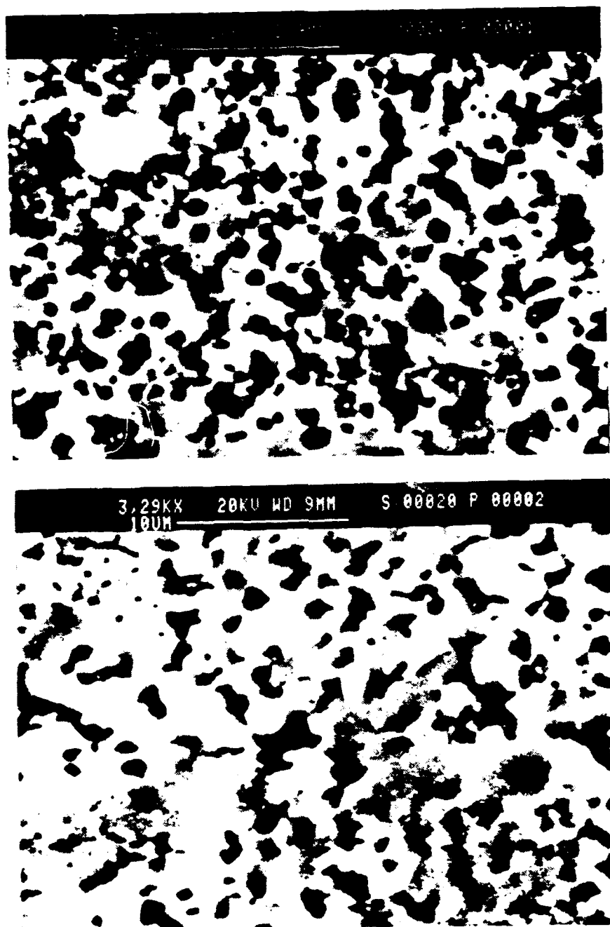
Figure 18. Electron Micrograph of TMP8 at \dot{\epsilon} = 6.11 \times 10^{-5} \text{sec}^{-1} : Interrupted tensile test specimen at \epsilon = 0.379 . Grip section shown (above), gage section shown (below).
