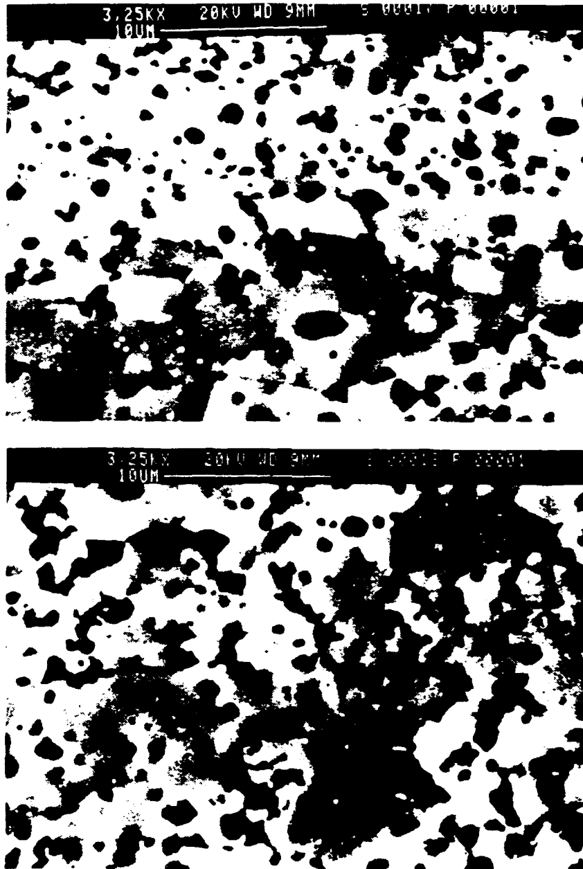
Figure 29. Micrographs of Statically Annealed TMP8: Material annealed for 5 hours (above) and 20 hours (below).
