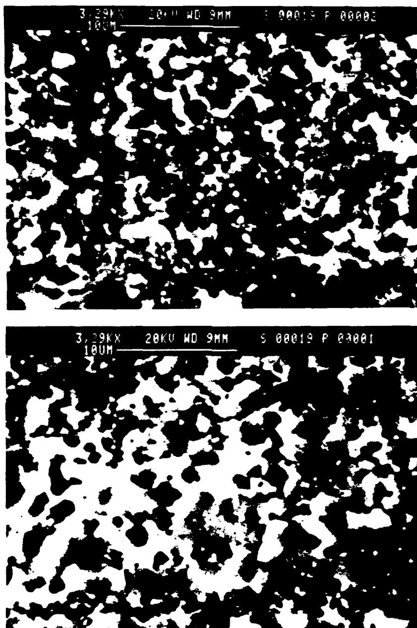
Figure 20. Electron Micrographs of TMP8 at \dot{\epsilon} = 1.99 \times 10^{-3} \text{sec}^{-1} : Interrupted tensile specimen showing relative grain growth of the grip section above and the gage section below at a higher strain rate then previously shown.
