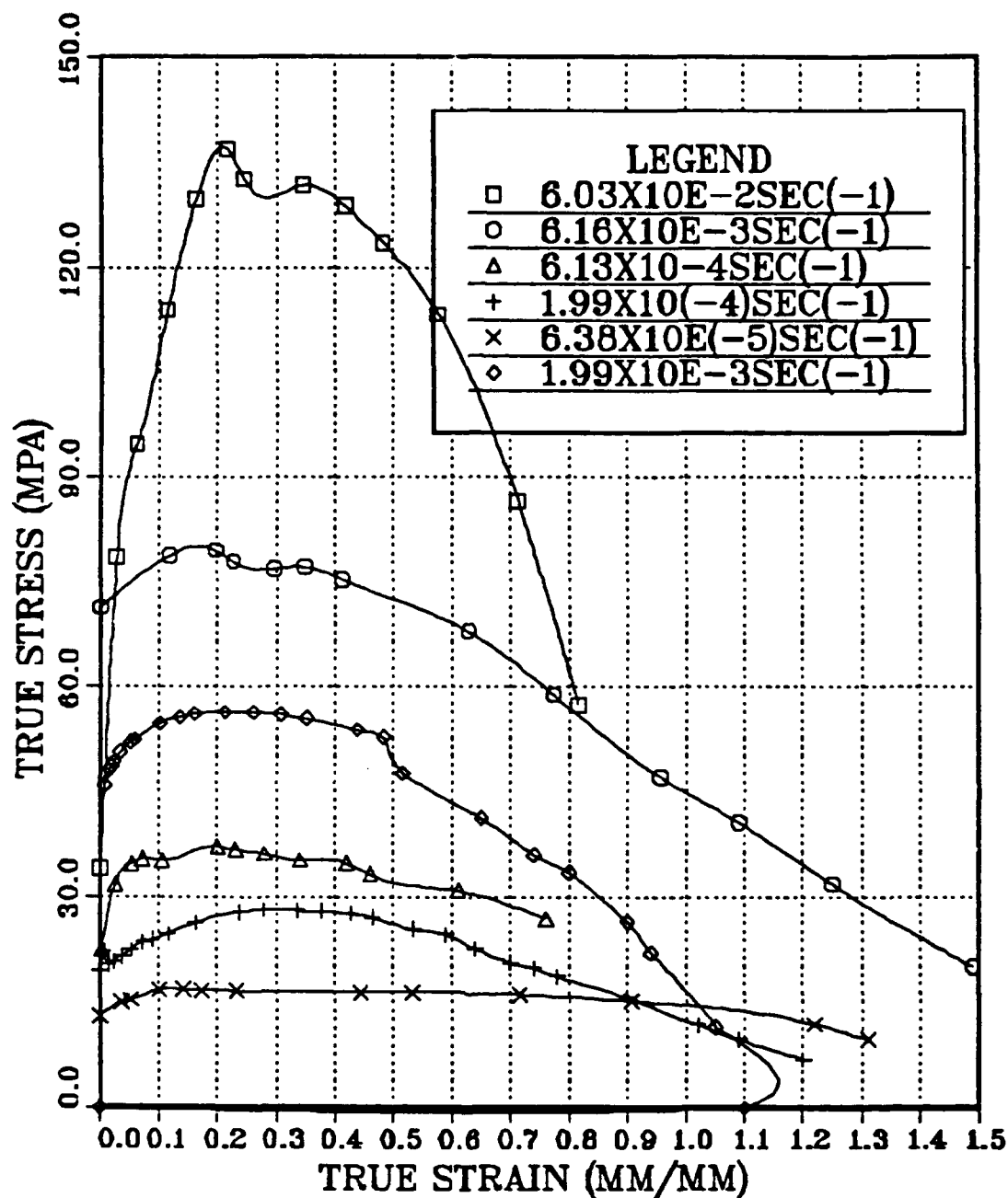
Figure 10. True Stress Strain Curve for TMP8
