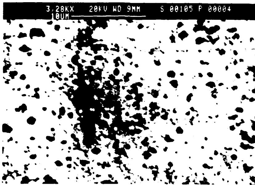
Figure 8. Electron Micrograph of TMP8 Material in as-rolled Condition
