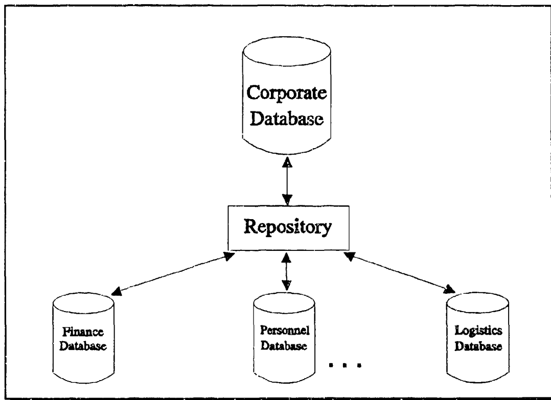
Figure 5. Repository and Database Relationship
