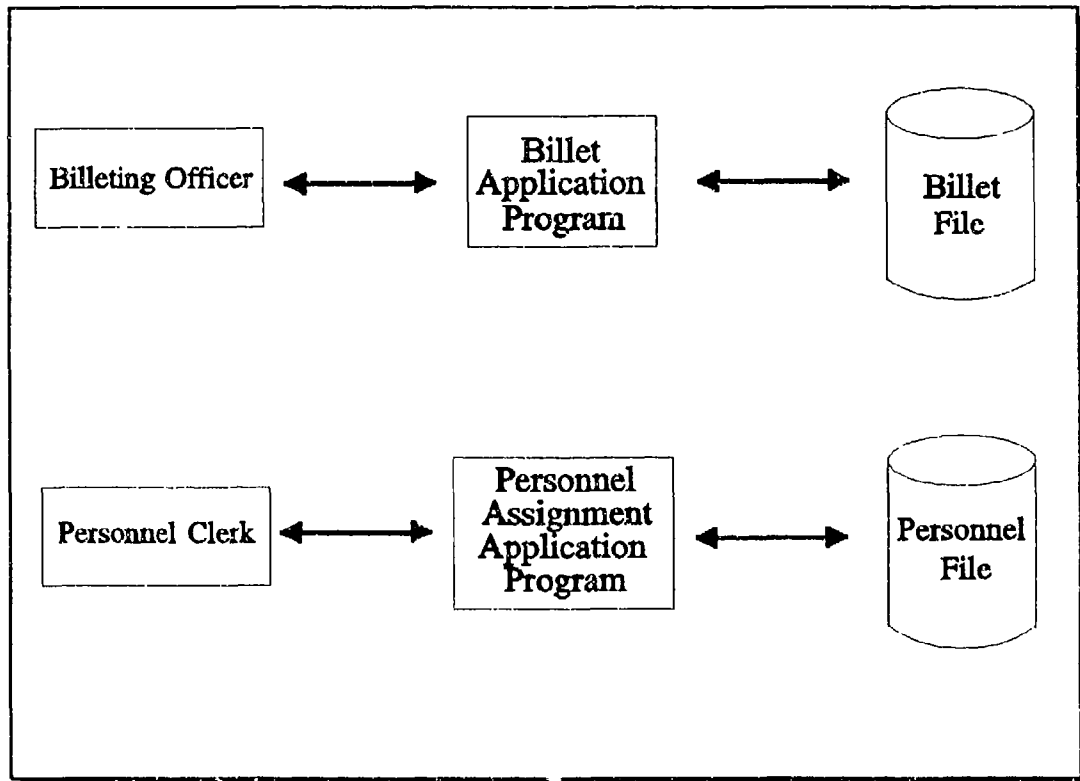
Figure 1. An Example of File Processing
