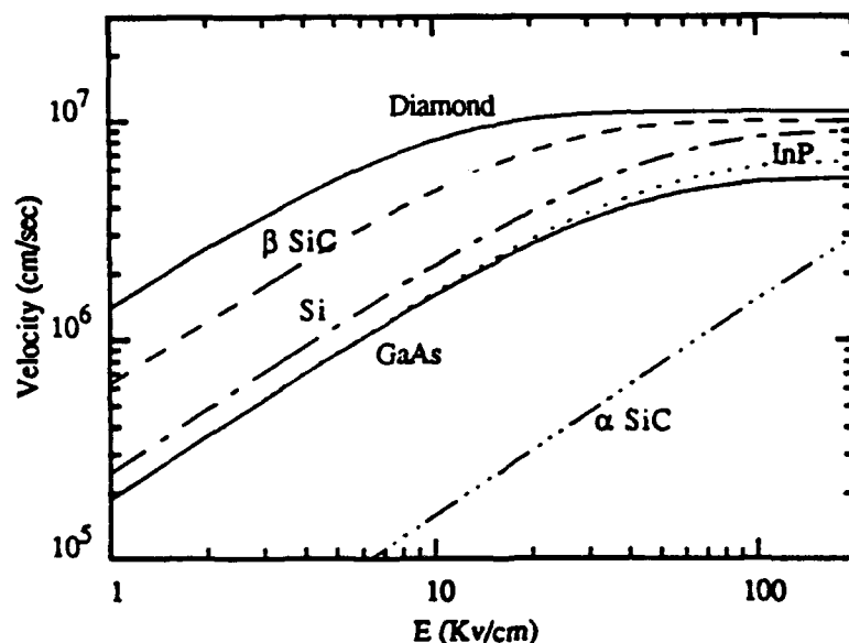
Figure 2. Hole velocity vs. electric field for several semiconductors at N_D = 10^{17} \text{ cm}^{-3} .
