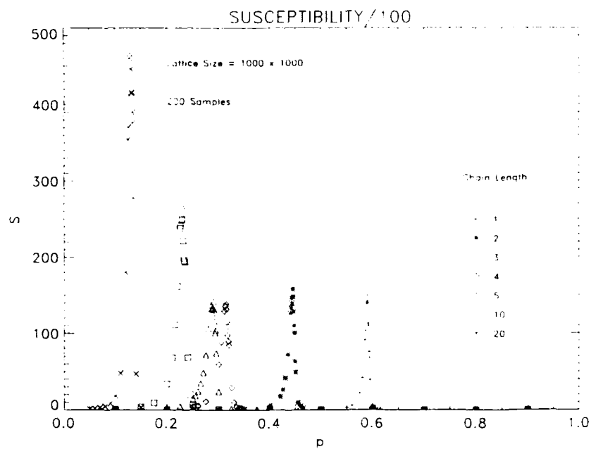
Fig. 3. Variation of the second moment S and p . Different chain-lengths are overlaid using different symbols.
