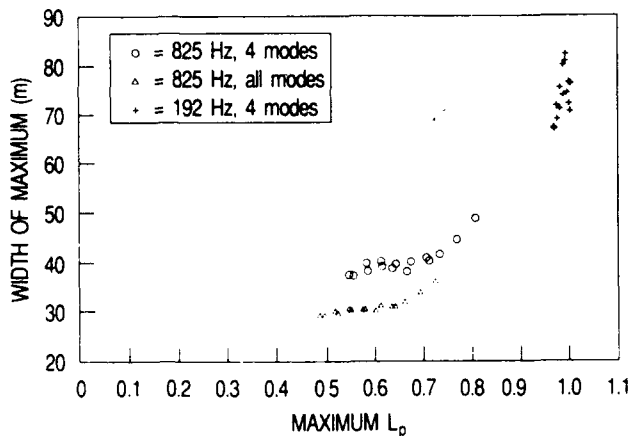
FIG. 10. Locator performance for an array of receivers. Examples are shown for two frequency bandwidths, 192 and 825 Hz. Examples are also shown for 825 Hz with 4 modes and 12 modes. Each of the series of points starts with 1 receiver at the upper left and moves downward and left as the number of receivers in the array increases.
