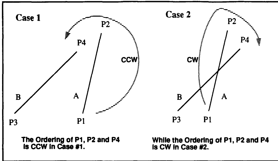
Figure 19: Illustration of Line Segment Intersections
