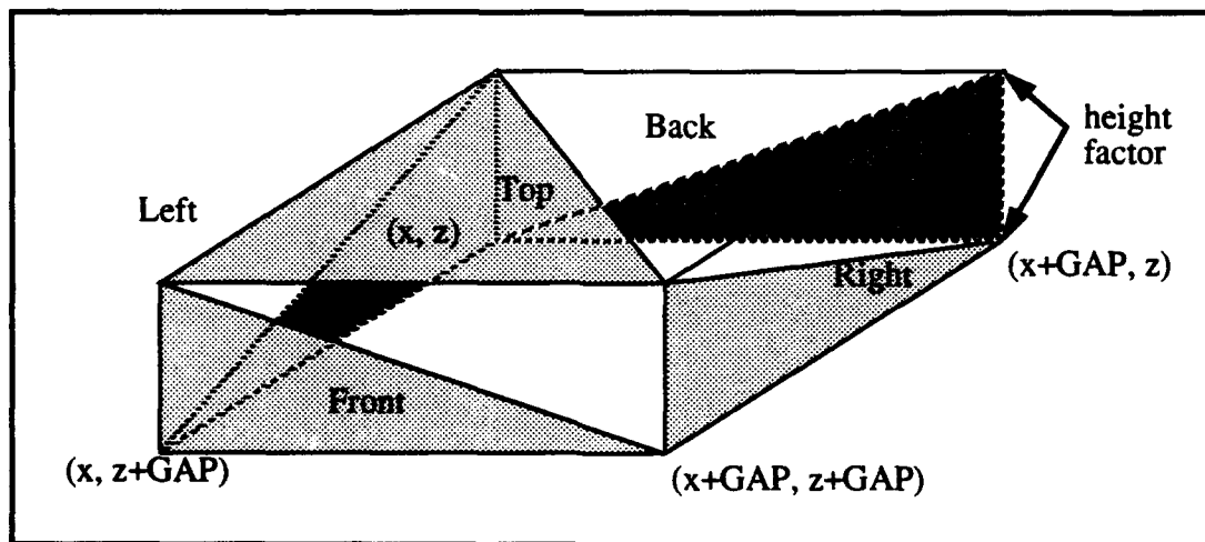
Figure 13: Drawing of a Tri-Mesh Canopy
