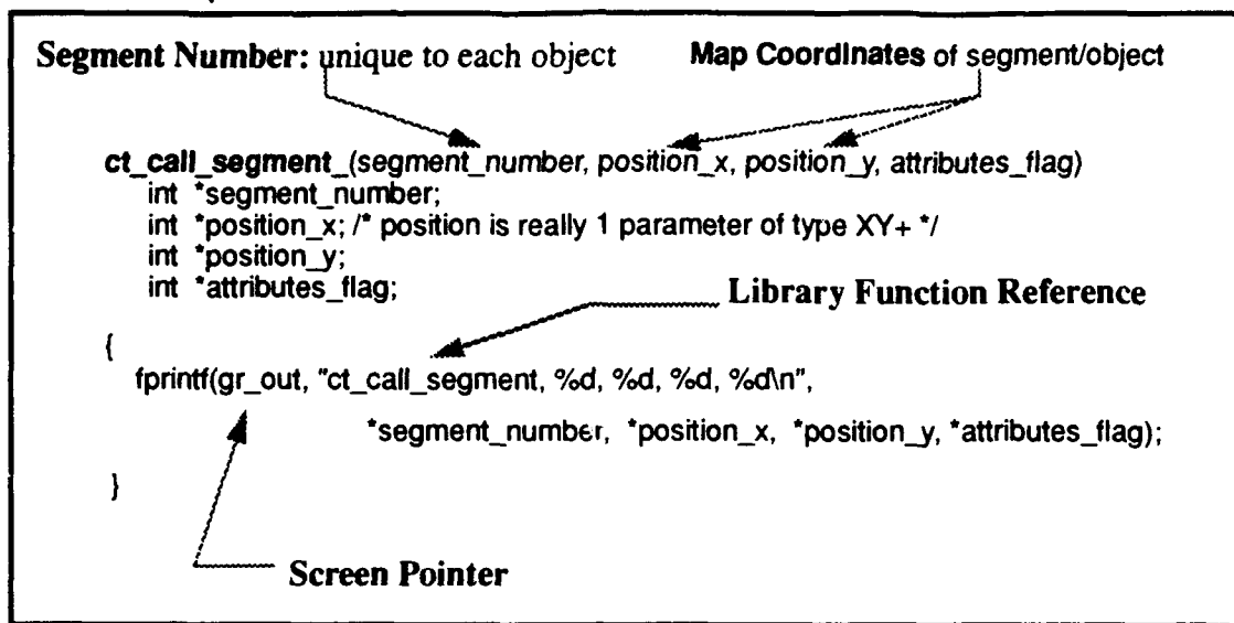
Figure 22: JANUS(X) Network Message Example
