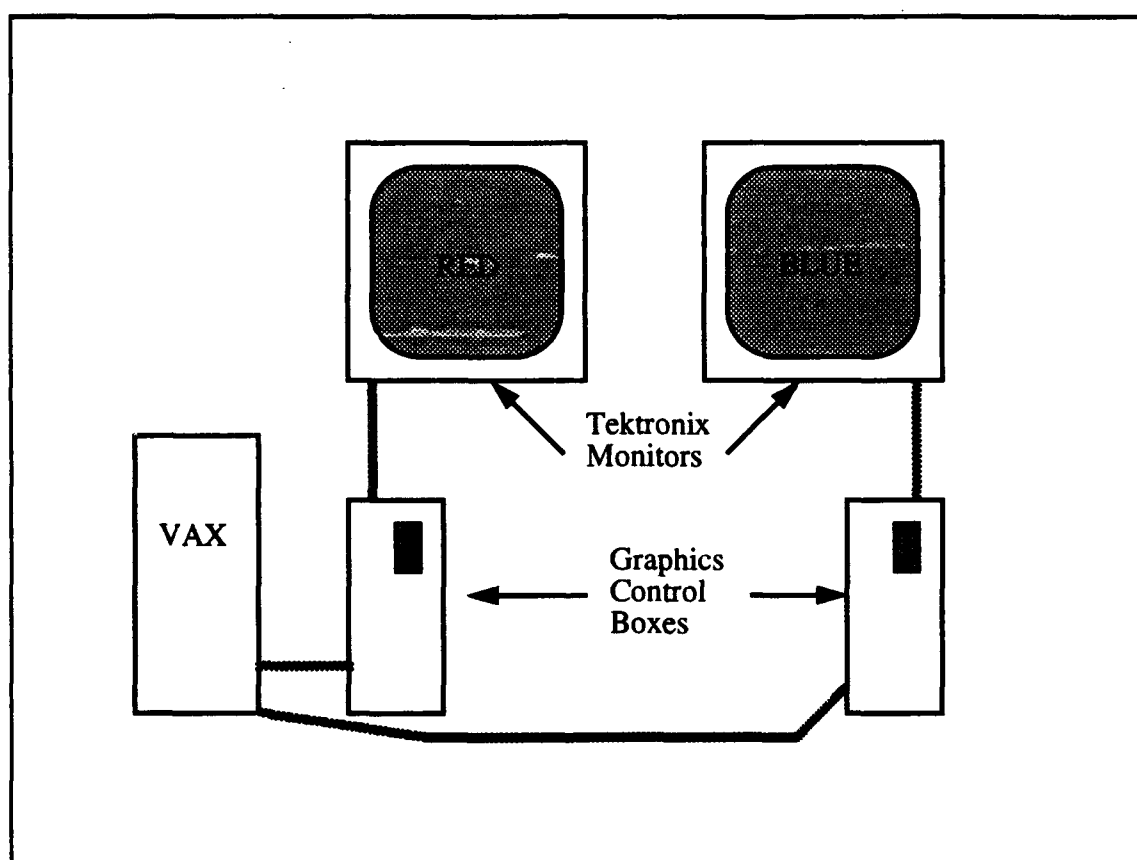
Figure 20: The Traditional JANUS(A) Hardware Setup.
