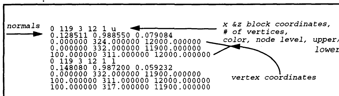
Figure 12: Quadnode File Representation
