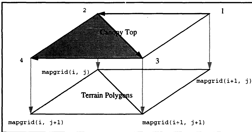
Figure 14: Order of Points for T-Mesh Canopy Top
