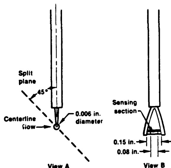
Figure 3-5. Schematic of Split Film Probe
