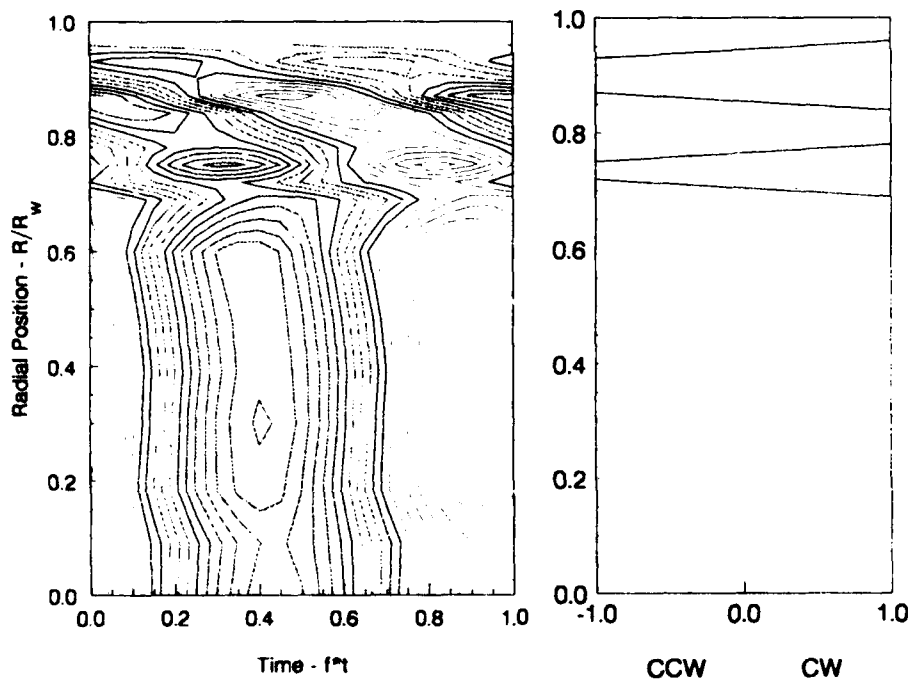
Figure 3-30. Axial Oscillatory Velocity at L/D = 4.22 (90 psia, M_s = 0.00197 )
