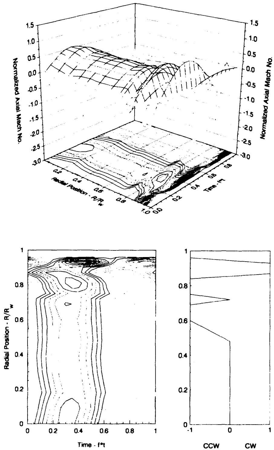
Figure 3-20. Axial Oscillatory Velocity at L/D = 1.8 (90 psia, M_s = 0.00197 )
