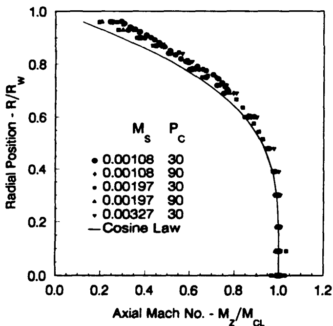
Figure 3-10. Axial Mean Velocity at L/D = 4.22
