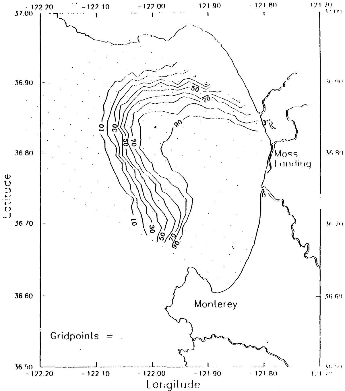
Figure 14. CODAR Coverage April, 1992: Contours indicate percentage of time the CODAR system produced total current vectors for each gridpoint. Coverage was calculated at each gridpoint by dividing the number of actual measurements derived by the possible number of measurements (240 in this case).
