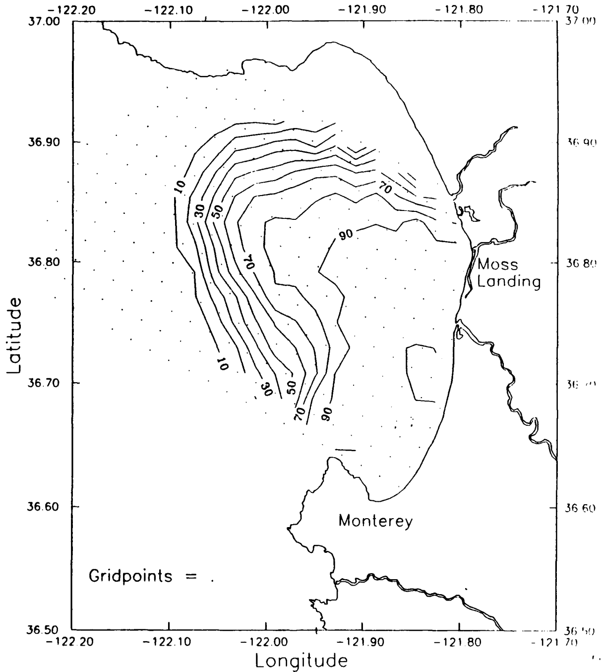
Figure 8. CODAR Coverage March to May, 1992: Contours indicate percentage of time the CODAR system produced total current vectors for each gridpoint. Coverage was calculated at each gridpoint by dividing the number of actual measurements derived by the possible number of measurements (762 in this case).
