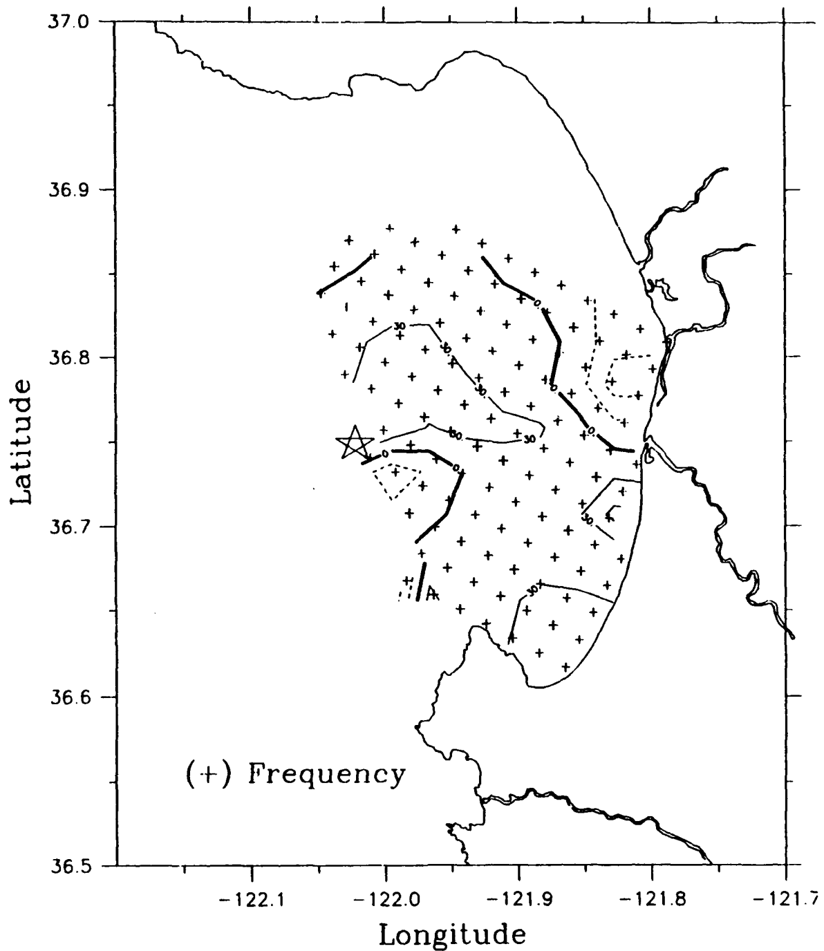
Figure 59. ADCP-CODAR Phase at 24 Hour Periods for Positive Frequencies: The majority of the area is less than 30^\circ in phase at 12 hour periods.
