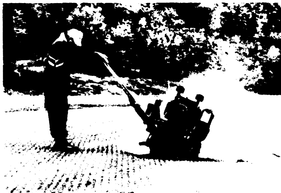
Figure 7. Routing a pavement crack prior to sealing.
