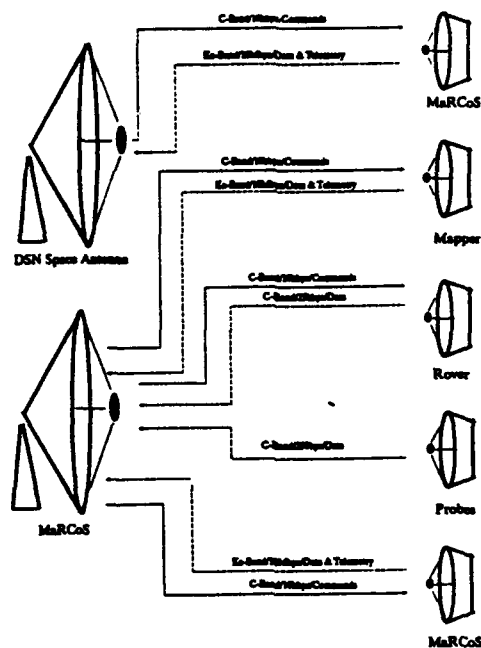
Figure 7. Communication Links.
