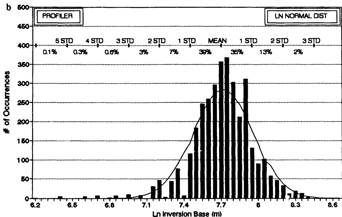
Figure 24. (a) Inversion base distribution (■) versus normal distribution (—) for profiler. (b) Natural log of inversion base distribution (■) versus normal distribution (—) for profiler. STD = Standard deviation.
