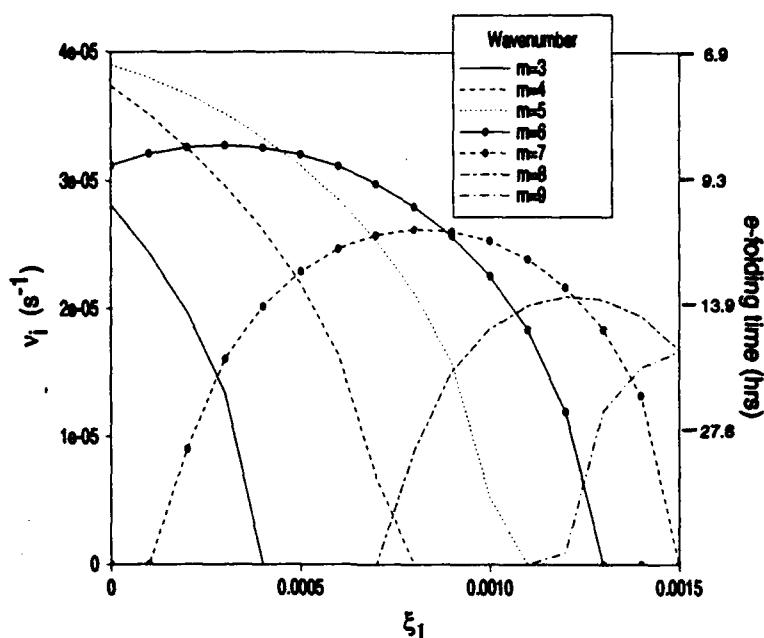
Figure 5.16: The growth rates ( \nu ) of the most unstable modes for wavenumbers m=3-9 as a function of \xi_1 . Constant values include r_1 = 50 km, r_2 = 200 km, r_3 = 250 km, and \xi_2 = -\xi_3 = 2.5 \times 10^{-4} .
