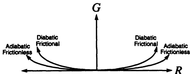
Figure 3.23: A schematic diagram of Leith's slow manifold. See text for explanation.
