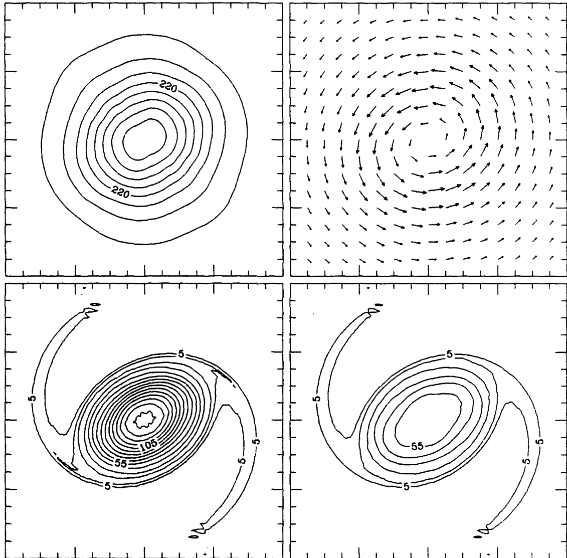
Figure 3.15: Same as Fig. 3.13 but at 12 hours.
