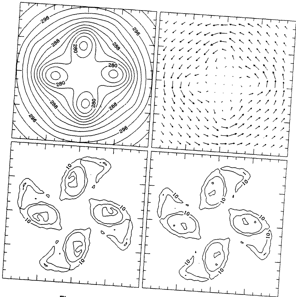
Figure 5.8: The same as Fig. 5.5 but for 48 hours.
