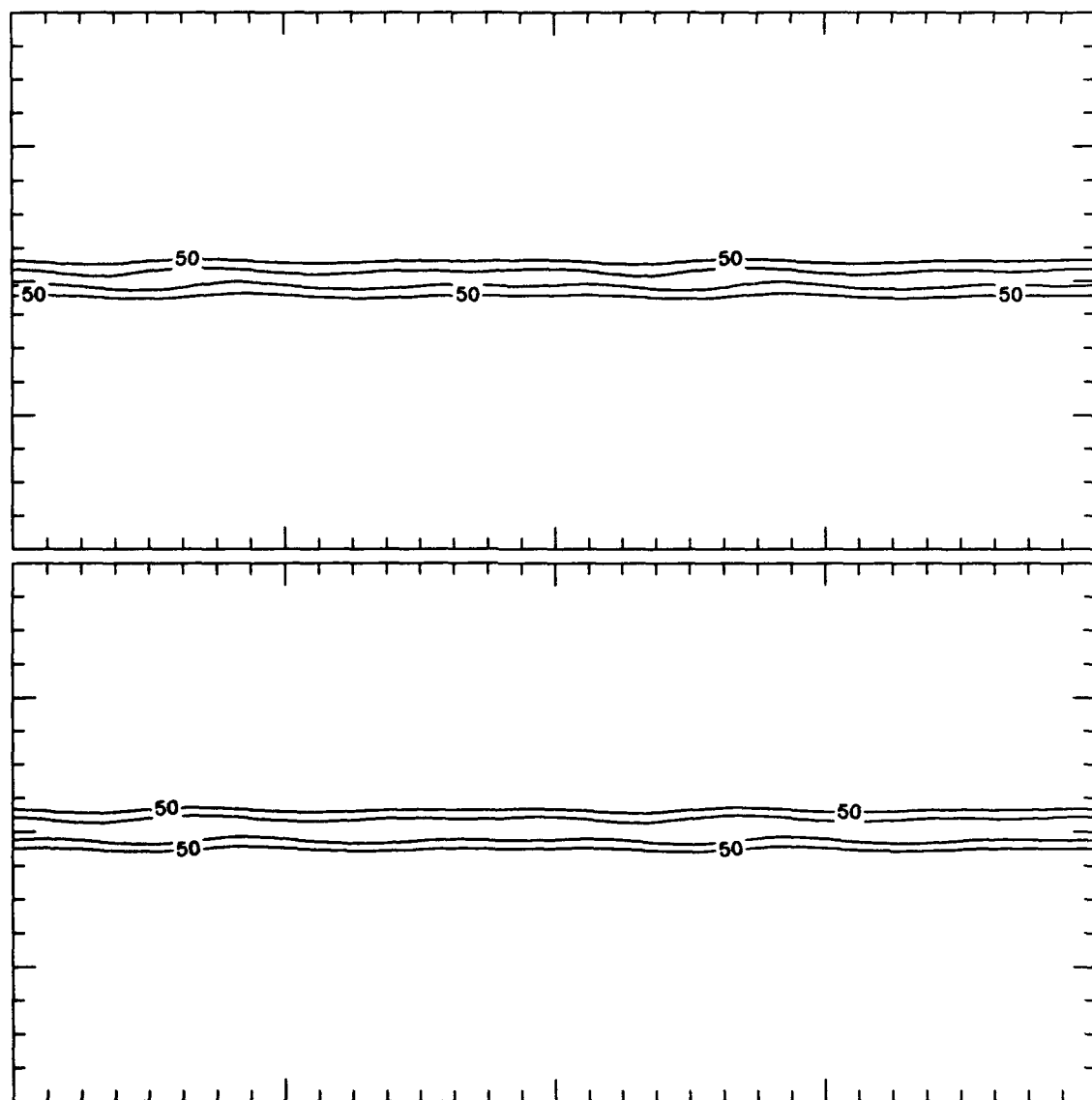
Figure 4.5: Vorticity (top) and FV (bottom) at day eight for experiment one. Two domain periods are shown. Units are 10^{-6} \text{ s}^{-1} and contour intervals are 25 \times 10^{-6} .
