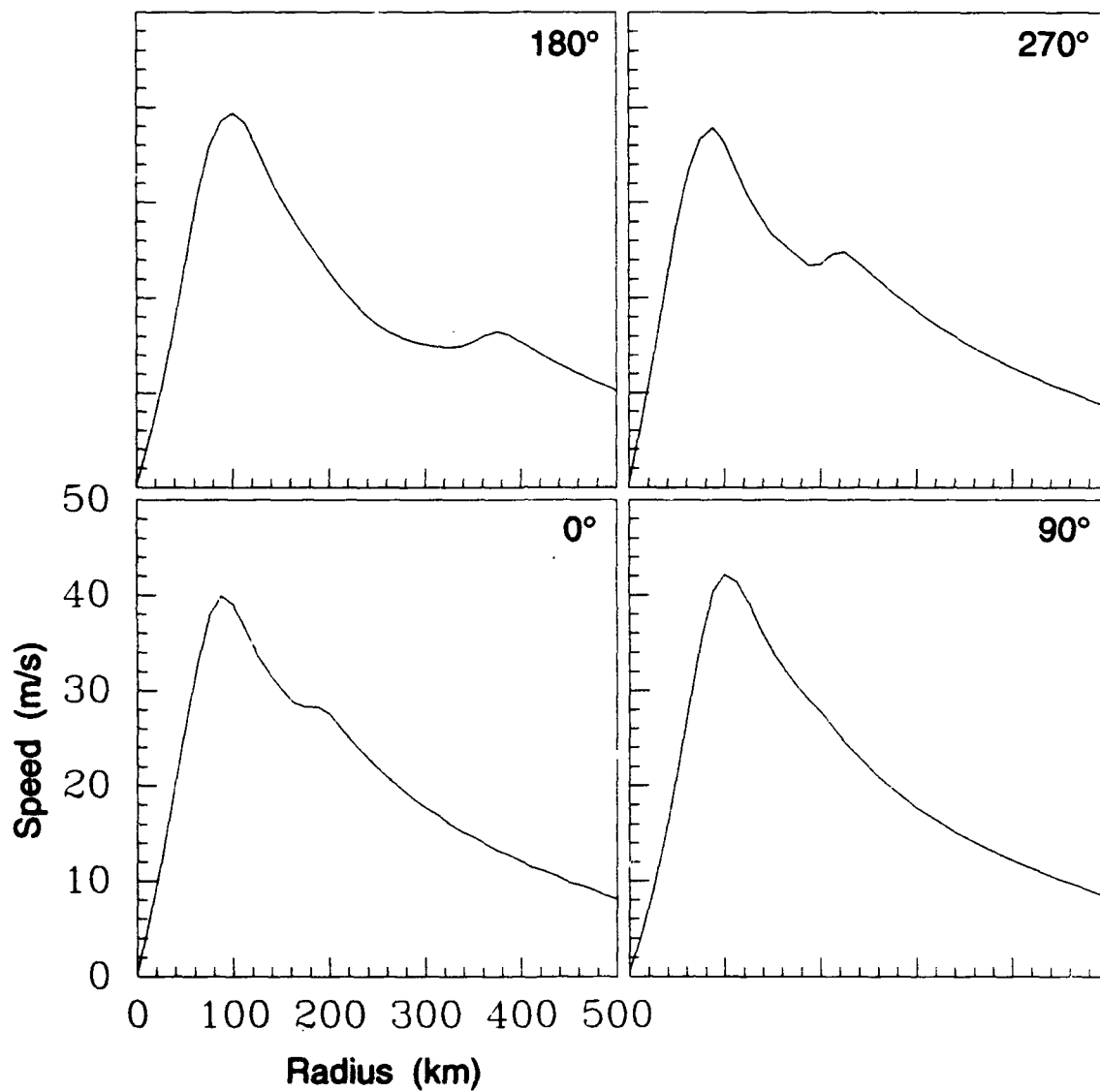
Figure 3.33: The tangential wind speed along four radial arms extending from the center of the vortex at 48 hrs (see Fig. 3.32). The radial arms are at 0° (lower left), 90° (lower right), 180° (upper left), and 270° (upper right) as measured from the positive x axis.
