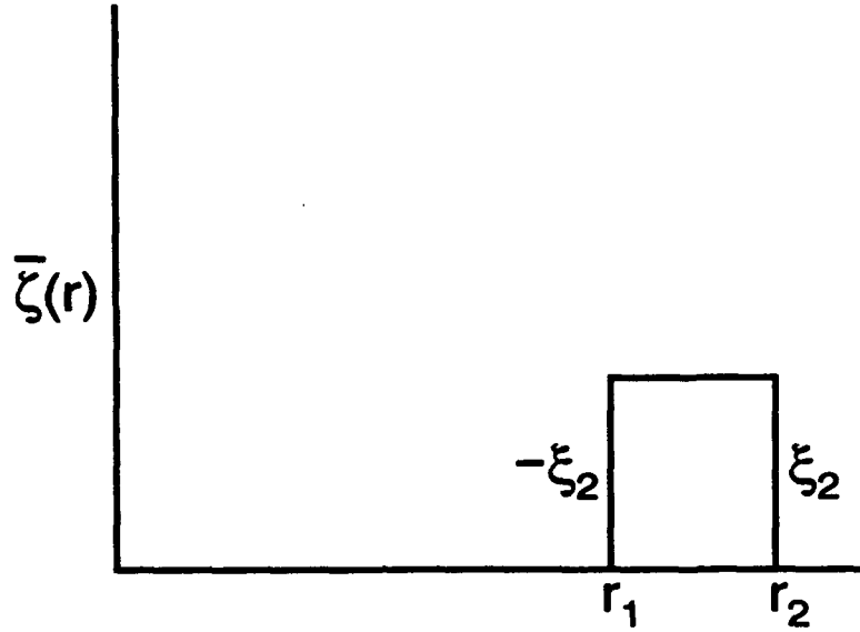
Figure 5.2: The assumed vorticity profile for J = 2 .
