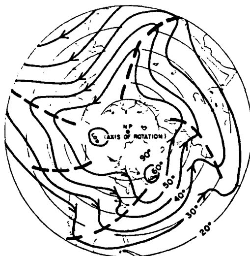
Figure 1.4: An artist's conception of how clouds associated with tilted troughs in the troposphere might appear from an extra terrestrial viewpoint. (From MacDonald, 1968.)
