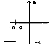
Fig. 1: The 2 layer single-step game of life template. The initial state has to be fed on the input of layer 1, and the new state will appear on the output of layer 2.
