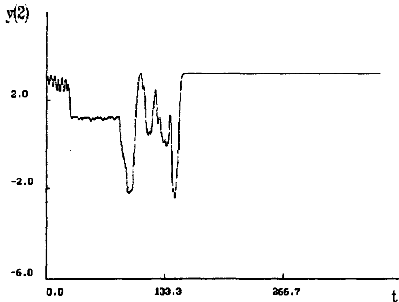
Fig.4. Pattern recognition: k = 0.02 , e = 0.002 . Z is an arbitrary external pattern for 0 < t < 140 and Z = V1 for t > 140 .
