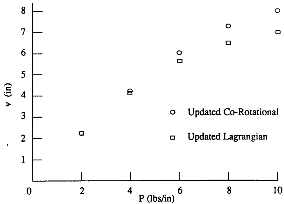
Figure 4.13 Problem 4.4 tip deflection versus load for updated lagrangian and updated co-rotational formulations
