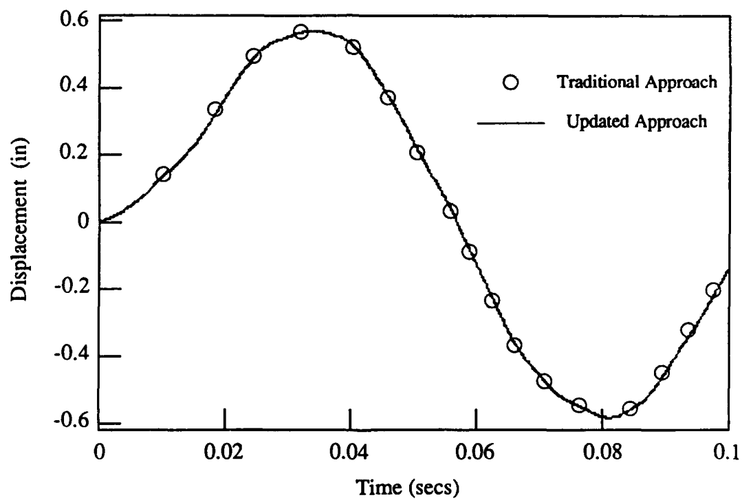
Figure 4.7 Problem 4.1 mid-span displacement history
