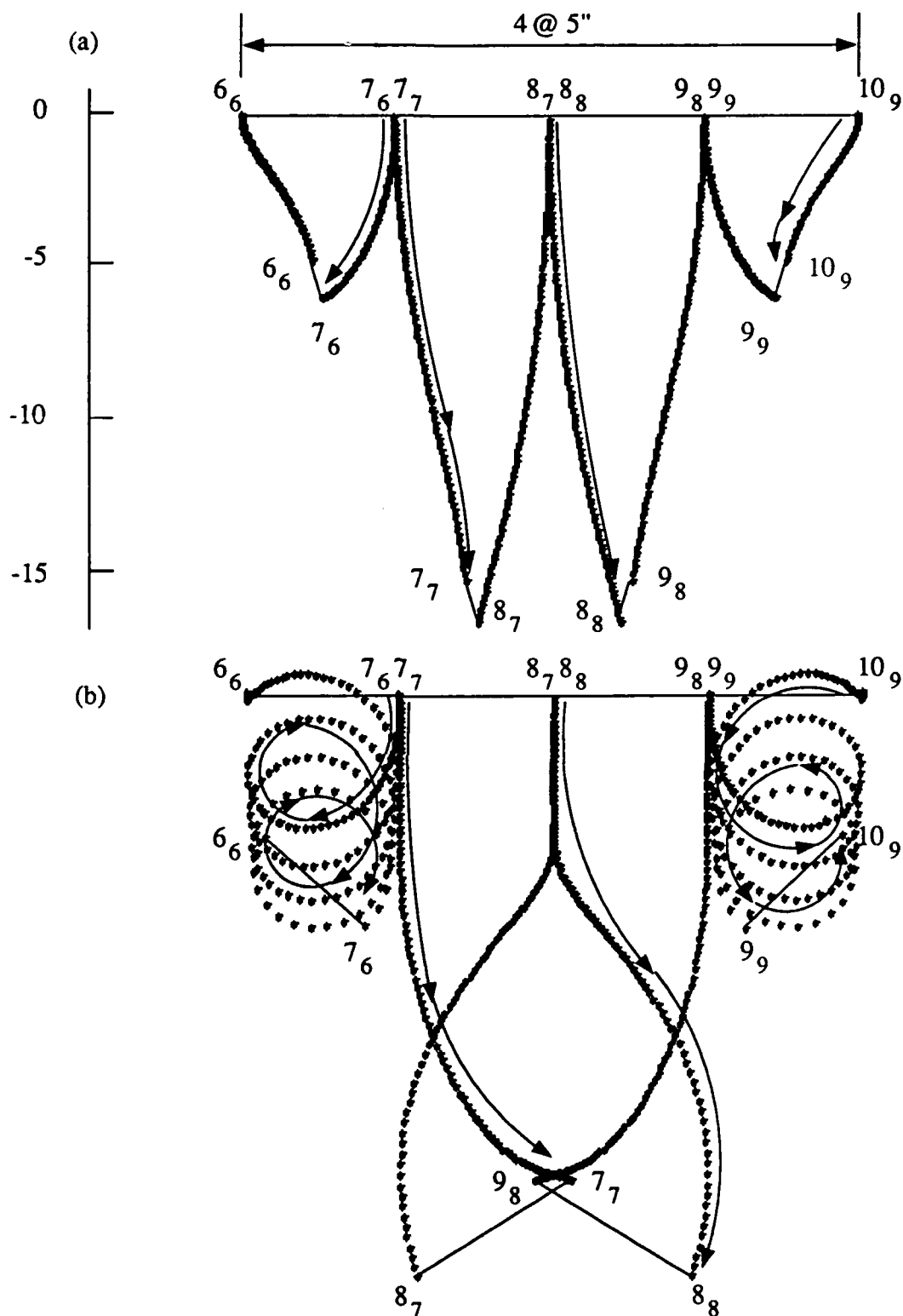
Figure 4.18 Displacement trace of fragments from Problem 3.2 for (a) traditional co-rotational and (b) updated formulations
