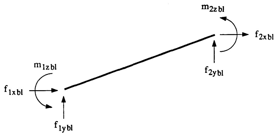
Figure 4.4 Element base-line forces
