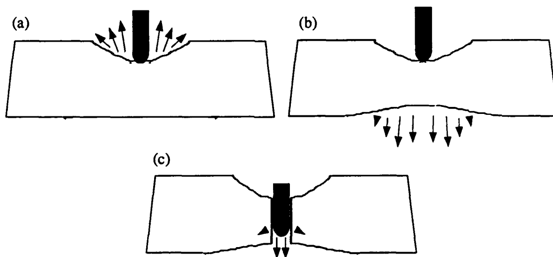
Figure 1.7 Concrete failure modes of (a) cratering, (b) spalling or scabbing, and (c) tunneling
