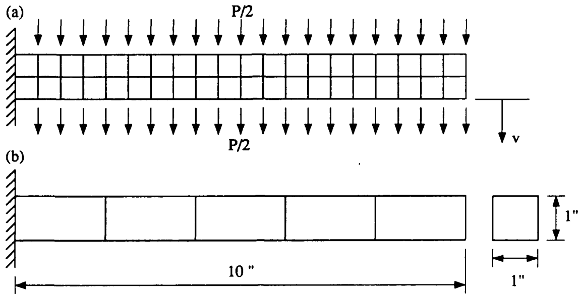
Figure 4.12 Problem 4.4 (a) 4-node element mesh showing loading and (b) 8-node element mesh showing geometry
