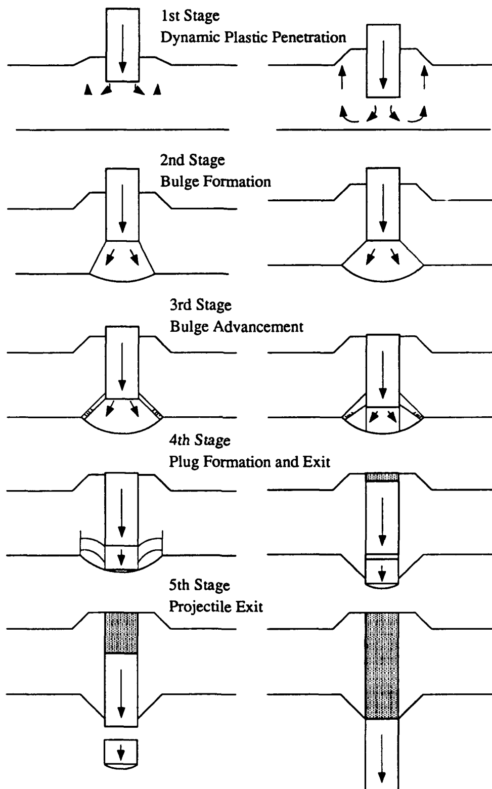
Figure 1.10 5-stage failure process from Ravid and Bodner (1983)
