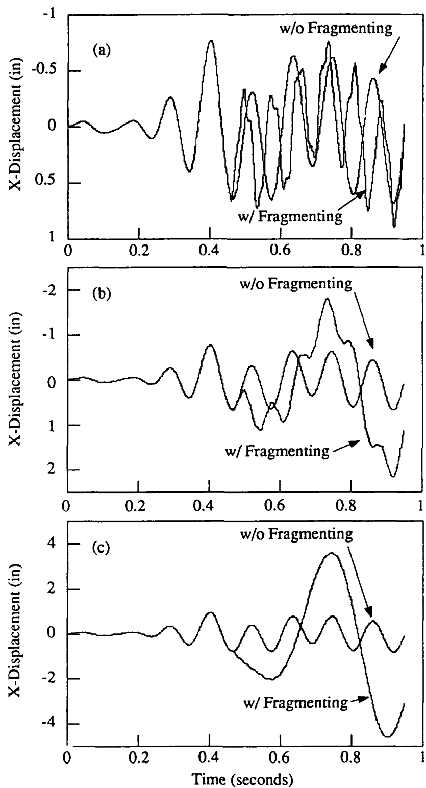
Figure 3.9 Problem 3.1 x-displacement history of (a) node 14a, (b) node 14b, and (c) node 34 without and with fragmenting permitted
