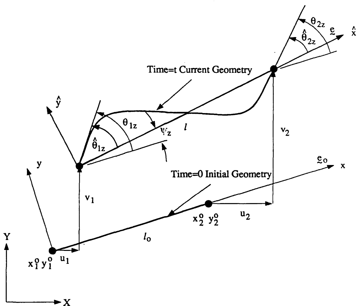
Figure 2.3 Initial and current geometries used for planar frame element in co-rotational approach
