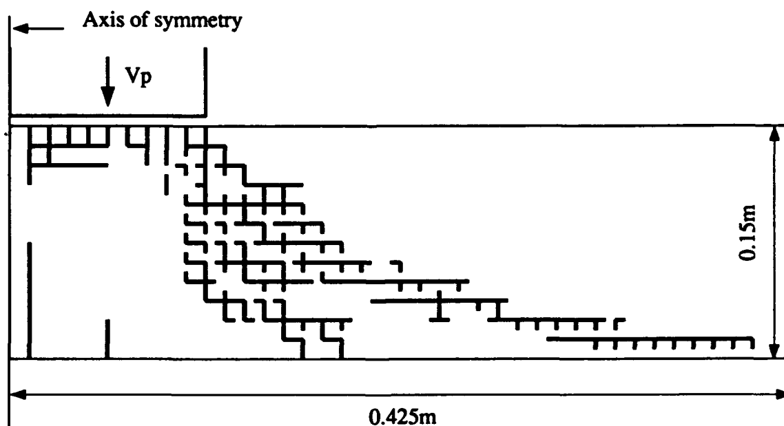
Figure 5.10 Problem 5.1 failure pattern after 0.0012 seconds
