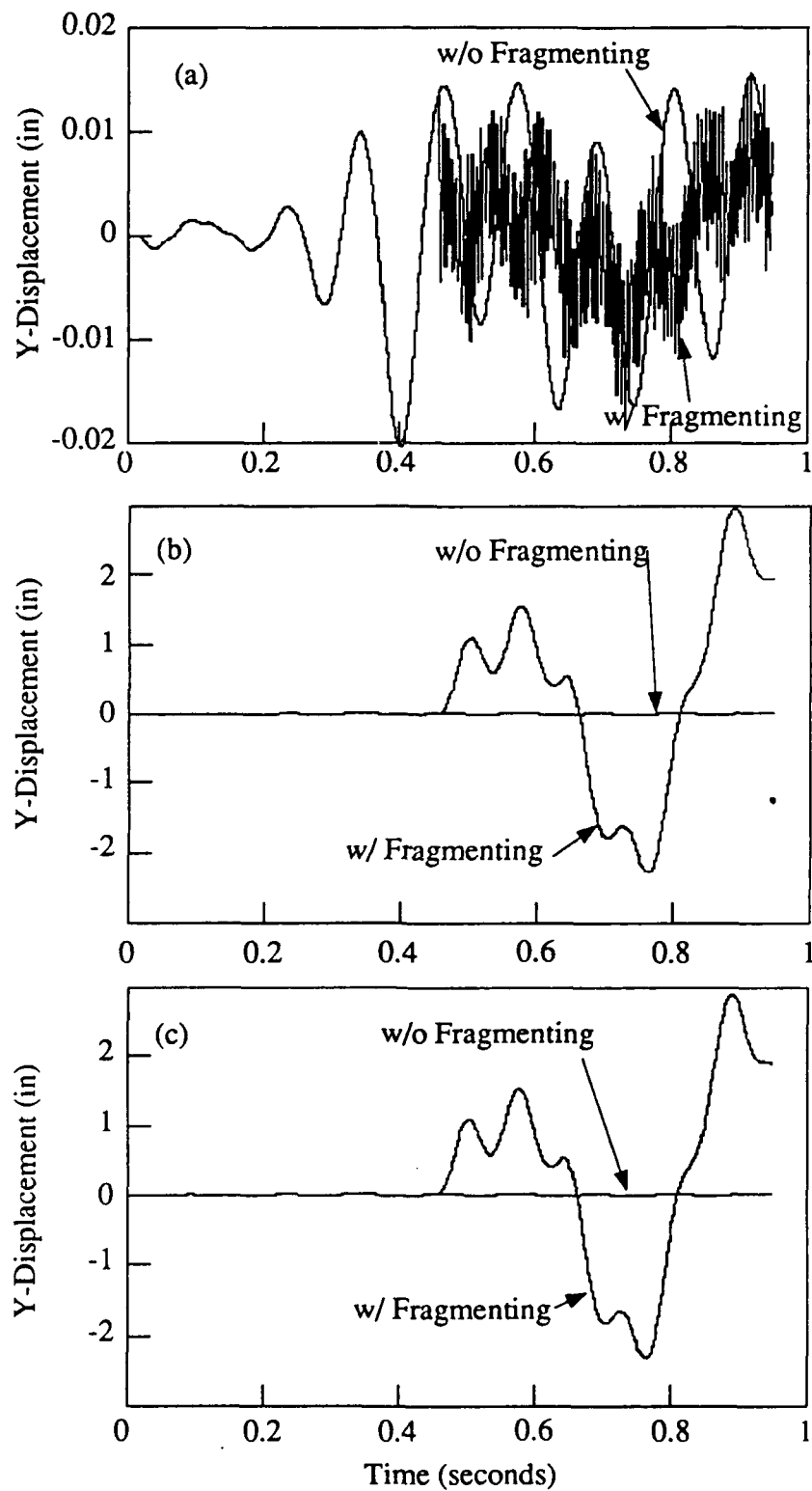
Figure 3.10 Problem 3.1 y-displacement history of (a) node 14a, (b) node 14b, and (c) node 34 without and with fragmenting permitted
