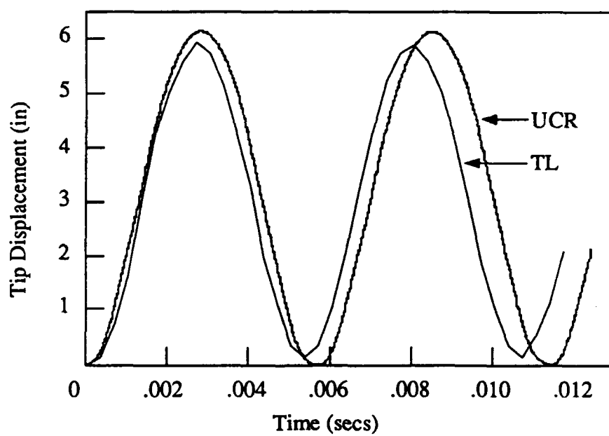
Figure 4.15 Problem 4.5 tip displacement history for updated lagrangian and updated co-rotational formulations
