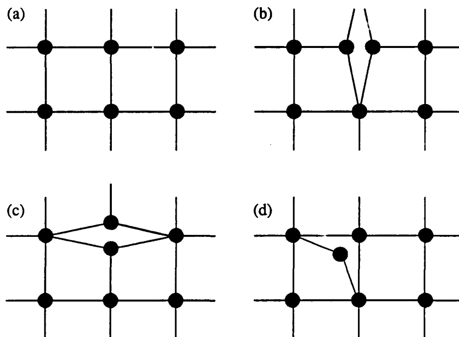
Figure 3.4 2-dimensional release showing (a) initial mesh, (b) vertical crack, (c) horizontal crack, and (d) diagonal crack
