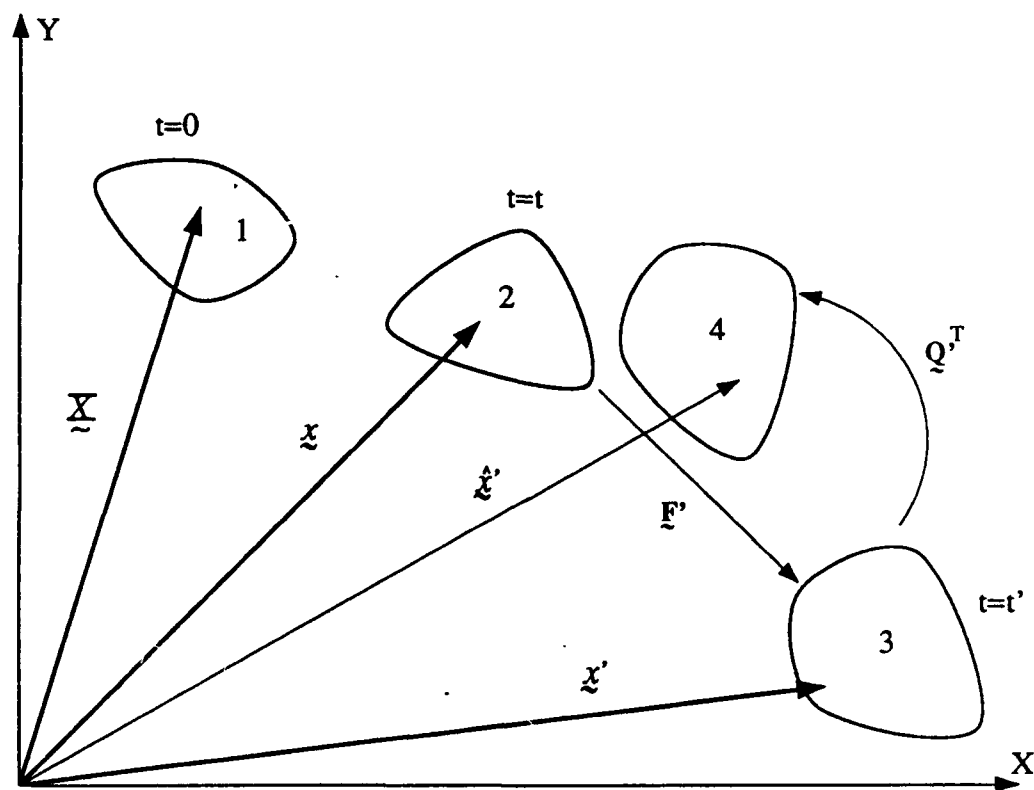
Figure 4.1 Stages of deformation in updated geometry formulation
