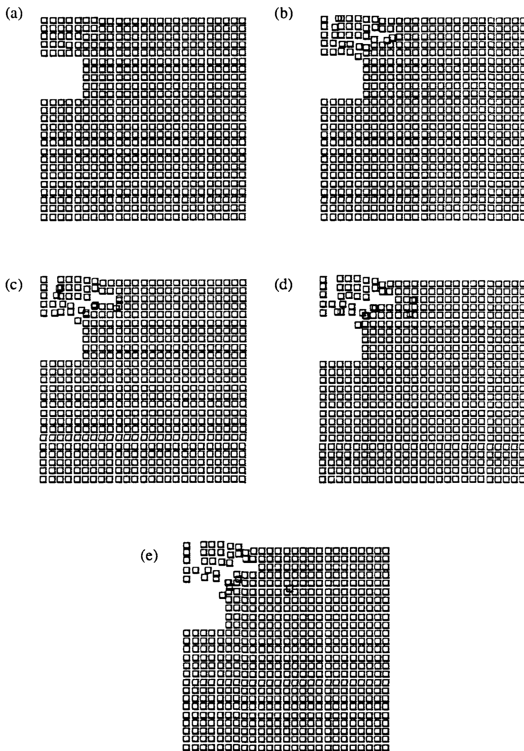
Figure 3.18 Problem 3.4 mesh at (a) .0004, (b) .0008, (c) .0012, (d) .0016, and (e) .002 seconds for elastic-fragment material model
