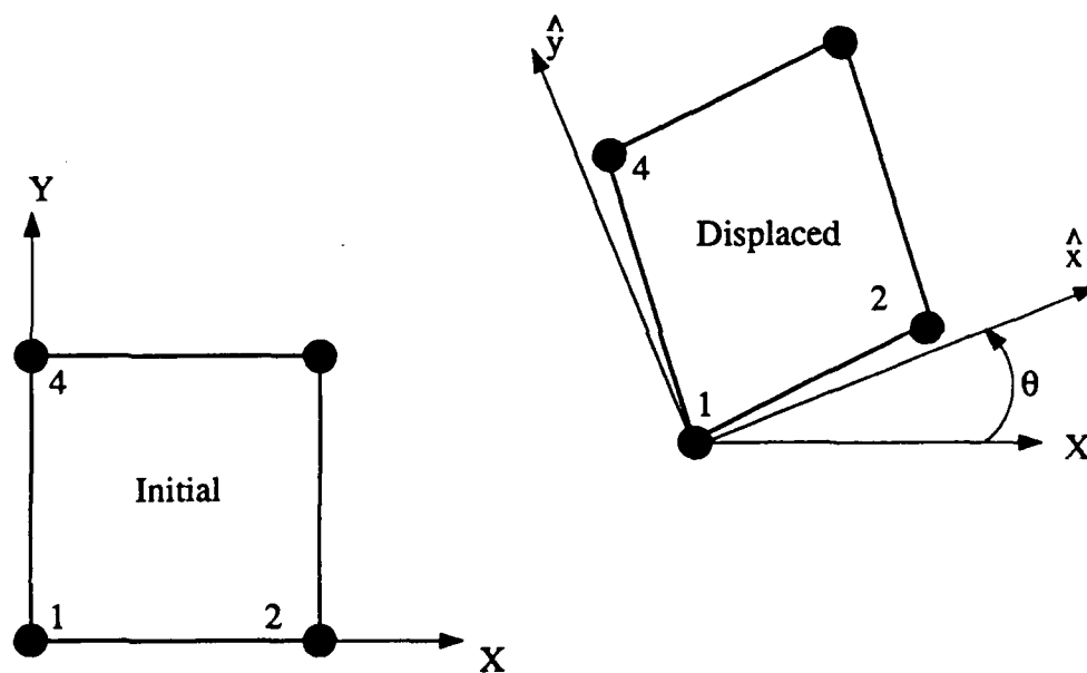
Figure 2.7 Initial configuration of 4-node isoparametric planar element and displaced configuration showing co-rotational coordinate system
