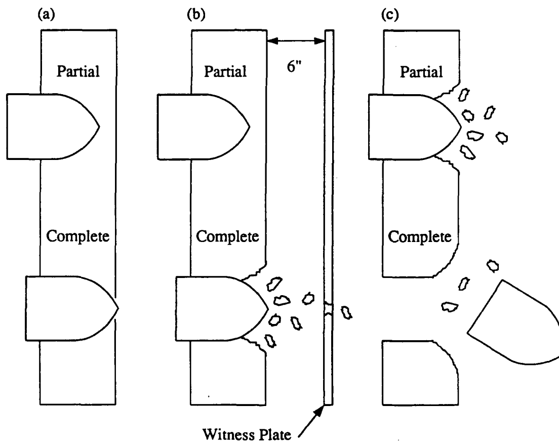
Figure 1.1 Definitions of partial and complete penetration for (a) Army Ballistic Limit, (b) Protection Ballistic Limit, and (c) Navy Ballistic Limit from Backman and Goldsmith (1978)
