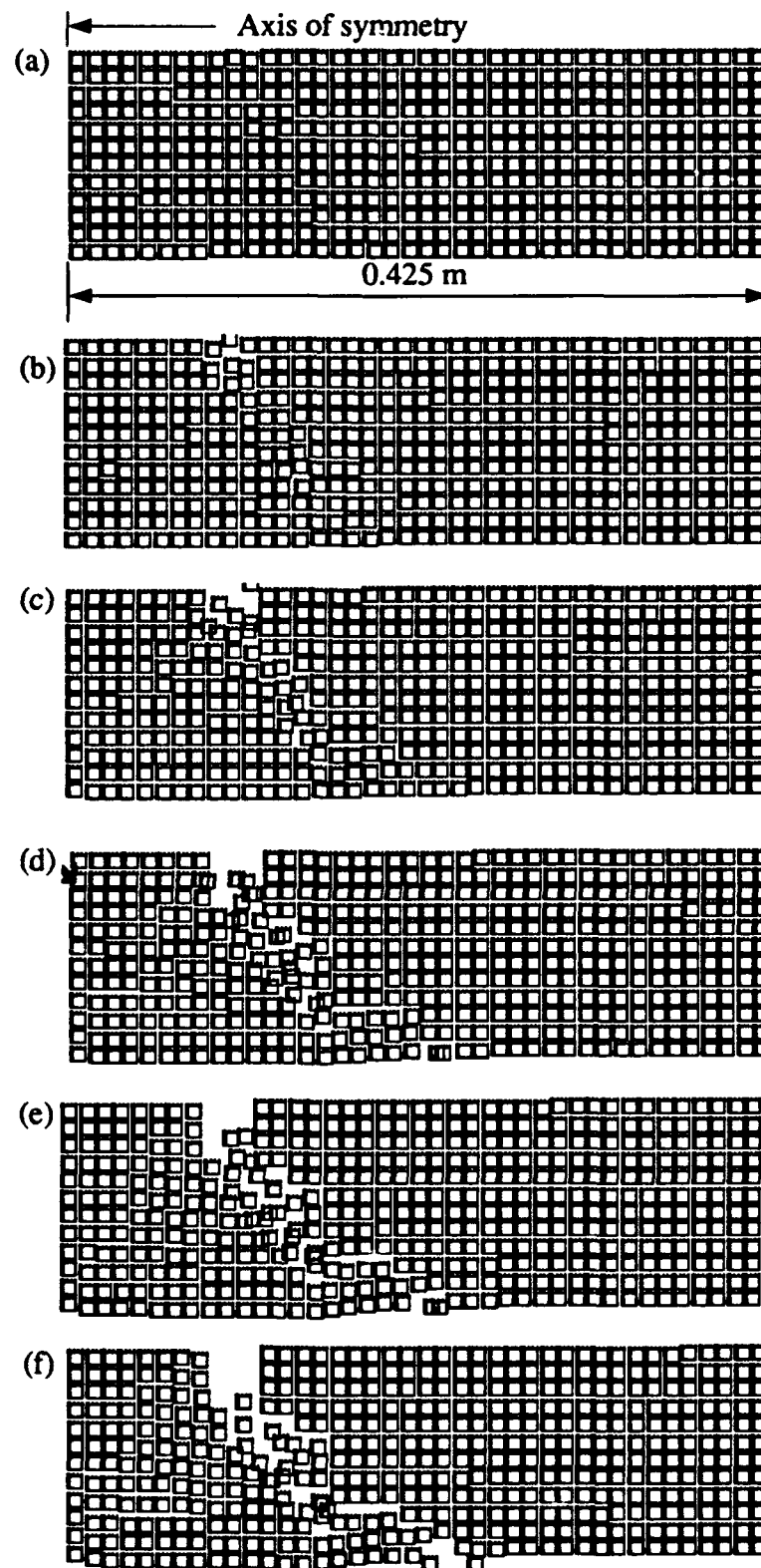
Figure 5.11 Problem 5.1 low-velocity impact of concrete plate at (a) 0.0002, (b) 0.0004, (c) 0.0006, (d) 0.0008, (e) 0.0010, and (f) 0.0012 seconds
