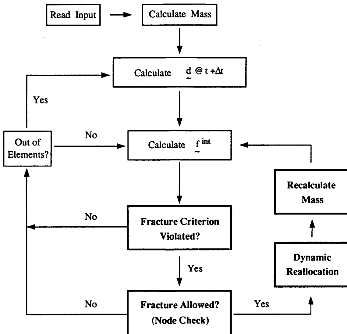
Figure 3.2 Flowchart of fragmentation algorithm
