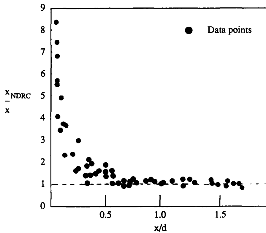
Figure 1.9 NDRC empirical formula compared to experimental data at various x/d ratios from Kennedy (1976)
