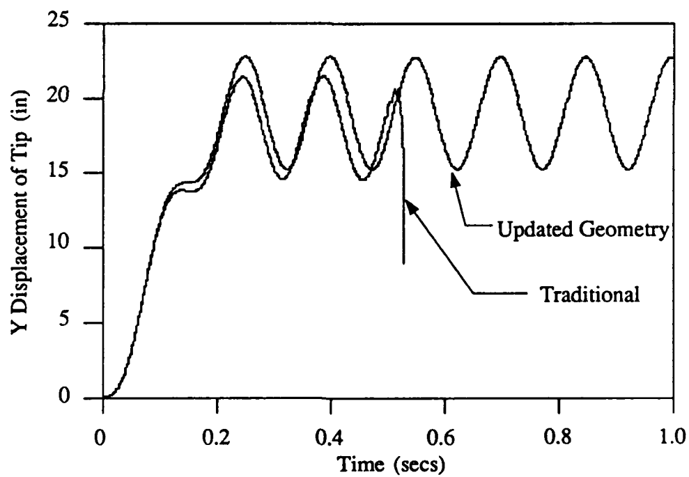
Figure 4.9 Problem 4.2 tip deflection showing comparison of traditional and updated approaches
