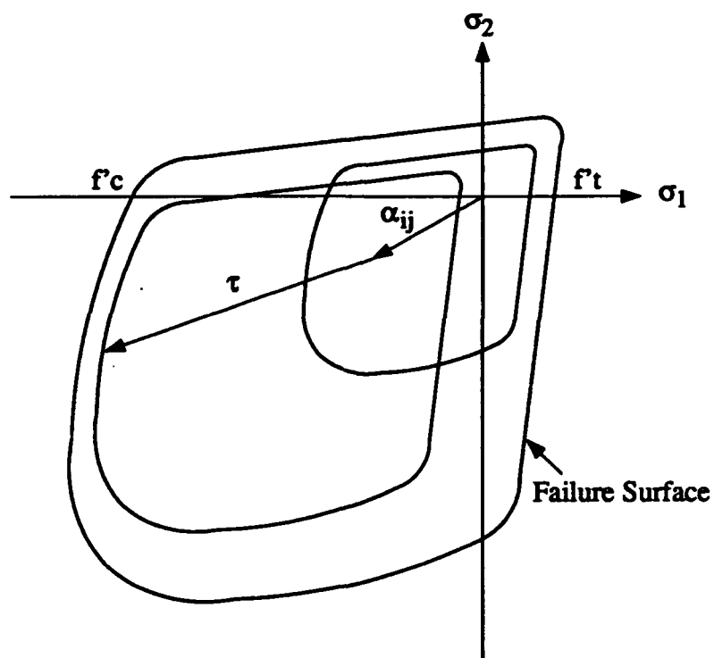
Figure 5.1 Schematic representation of H-T-C 4-parameter concrete material model in the biaxial stress plane from Labbane (1991)
