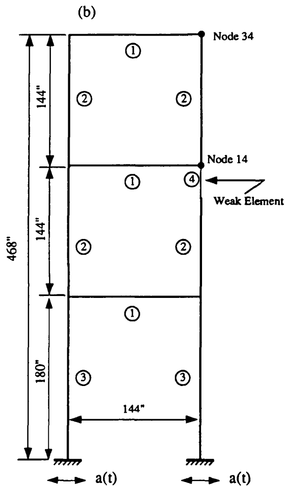
Figure 3.7 Problem 3.1 (a) ground acceleration history and (b) frame geometry, section properties, and material properties
