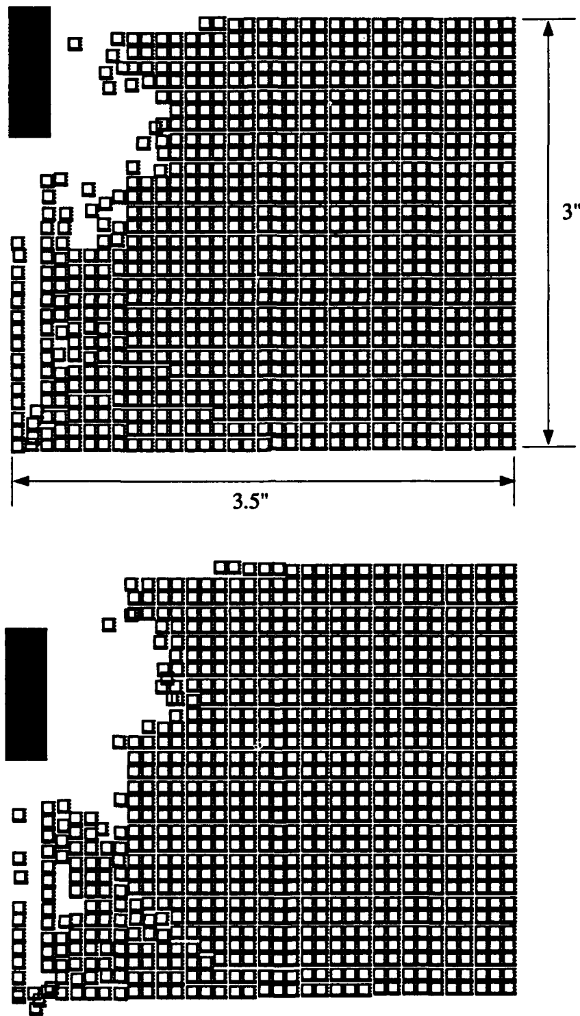
Figure 5.29 Deformed mesh for Problem 5.12 at 1 \times 10^{-4} , 2 \times 10^{-4} , 3 \times 10^{-4} , and 3.9 \times 10^{-4} seconds
