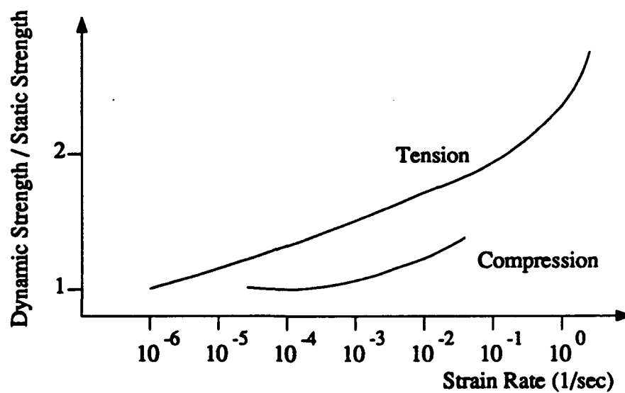
Figure 5.2 Comparison of strain-rate sensitivity in tension and compression from Suaris and Shah (1983)
