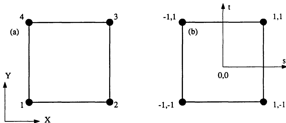
Figure 2.5 4-node isoparametric plane-stress/strain element in (a) global and (b) natural coordinates
