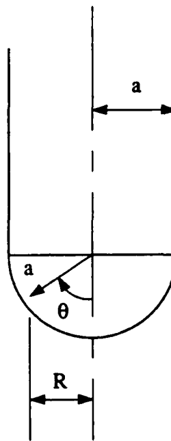
Figure 1.11 Projectile parameters from Luk and Forrestal (1987) for analytical solution of concrete impact
