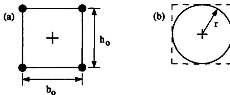
Figure 5.6 (a) Element geometry used to calculate size of pseudo-element and (b) resulting pseudo-element
