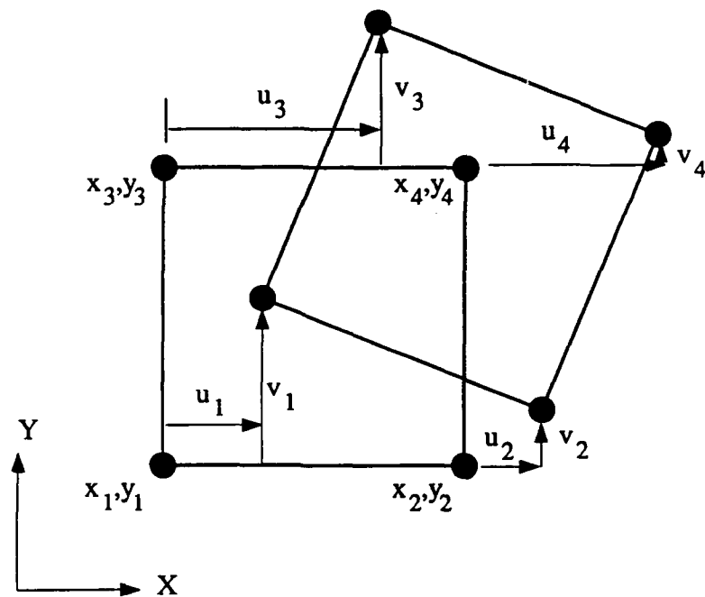
Figure 2.6 Element nodal coordinates and displacements
