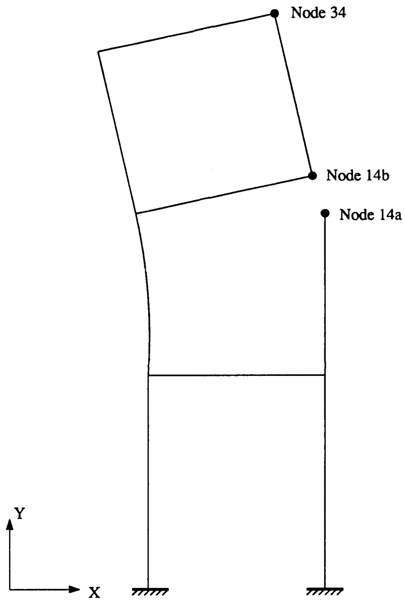
Figure 3.8 Problem 3.1 fragmented structure configuration
