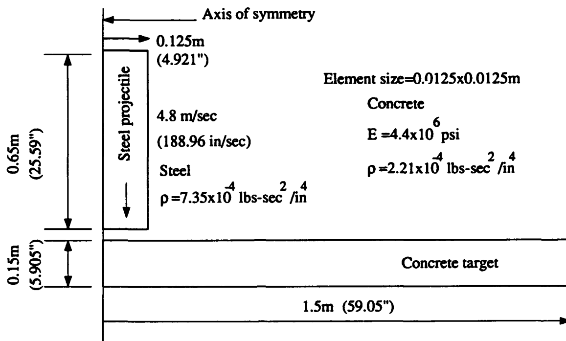
Figure 5.9 Problem 5.1 low-velocity impact geometry, material properties and initial conditions
