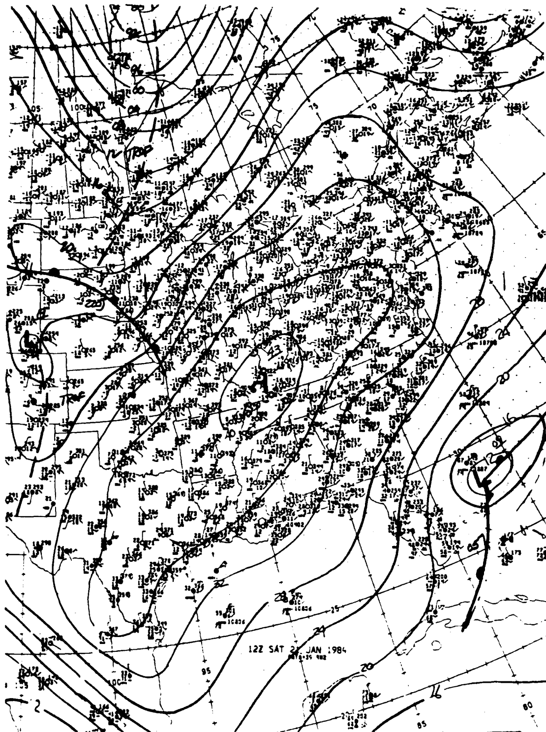
Fig. 6.1. NMC surface analysis valid at 1200 UTC, 21 January 1984.
