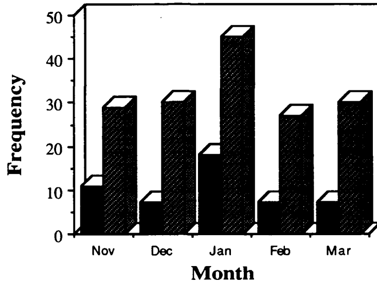
Fig. 5.1. Monthly frequency of coastal front occurrences. Current study's values (solid) based on 51 cases, while Anderson's values (hatched) are based upon 161 cases.
