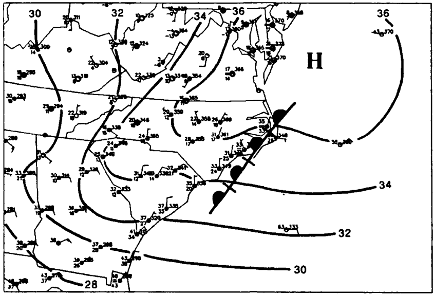
Fig. 6.4. Surface analysis valid at 1200 UTC 23 January 1984.
