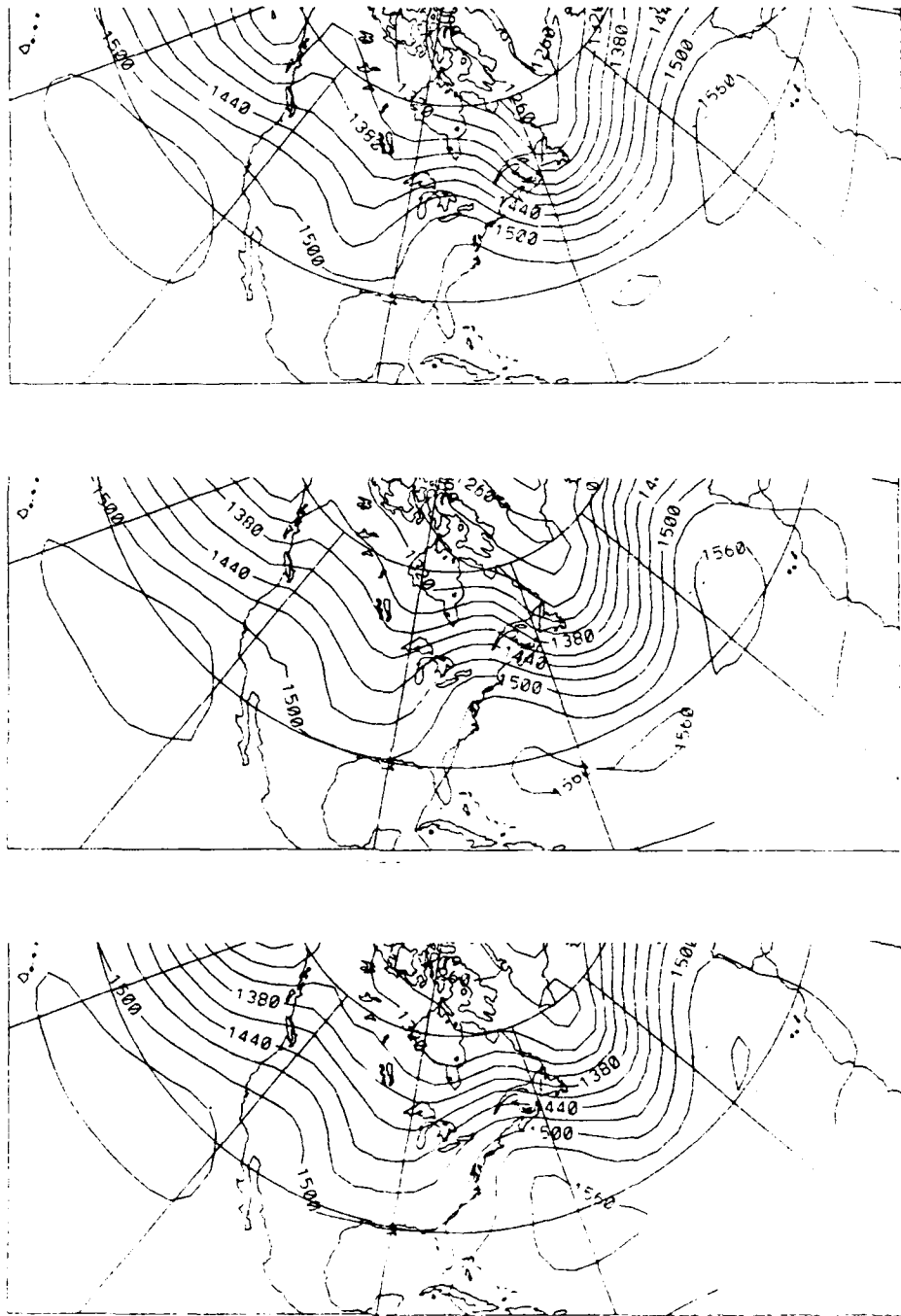
Fig. 5.14. Composite 850 mb height pattern for offshore events. Time sequence is the same as given in figure 5.13.
