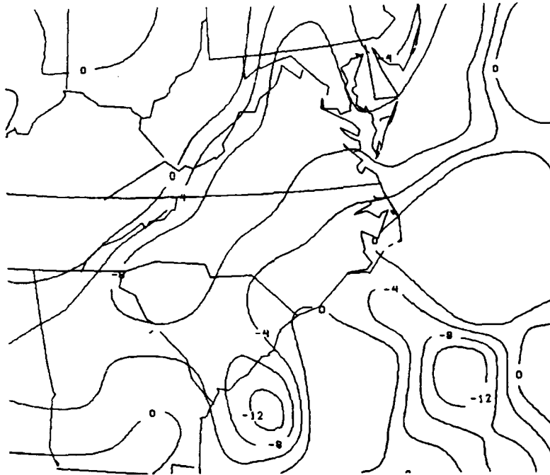
Fig. 12.11. Analysis of the Laplacian of sea level pressure valid at 1800 UTC 24 January 1986. Values given are \times 10^{11} mb m^{-2} , and the contour interval is four units.
