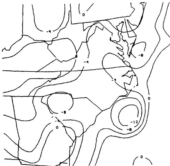
Fig. 12.10. Analysis of the Laplacian of sea level pressure valid at 1200 UTC 24 January 1986. Values given are \times 10^{-11} \text{ mb m}^{-2} , and the contour interval is four units.
