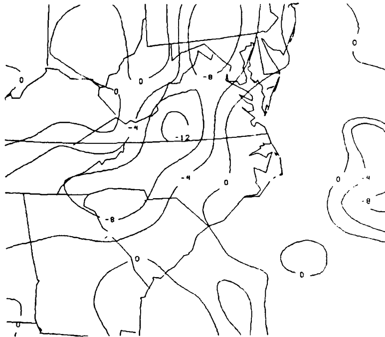
Fig. 12.14. Analysis of the Laplacian of sea level pressure valid at 1200 UTC 25 January 1986. Values given are \times 10^{-11} \text{mb m}^{-2} , and the contour interval is four units.
