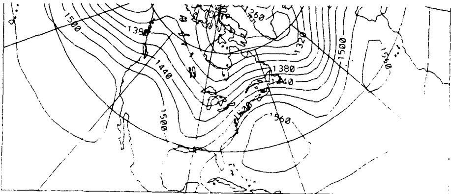
Fig. 5.13. Composite 850 mb height pattern for onshore events at 12 hours prior to HAT frontal passage, at frontal passage, and 12 hours subsequent to frontal passage.
