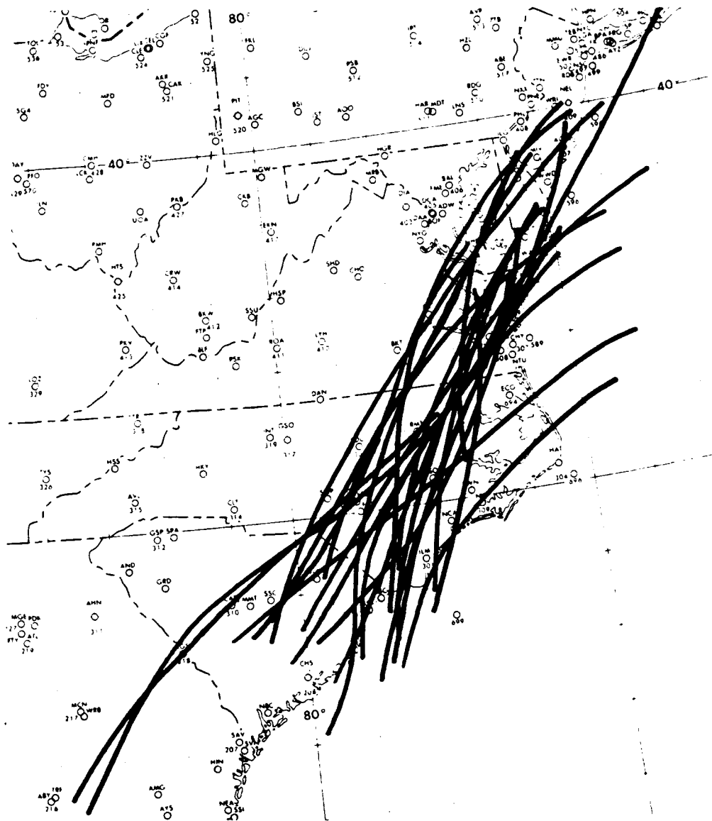
Fig. 5.4. Terminal positions of Carolina coastal fronts for 24 events not involving a cyclone.
