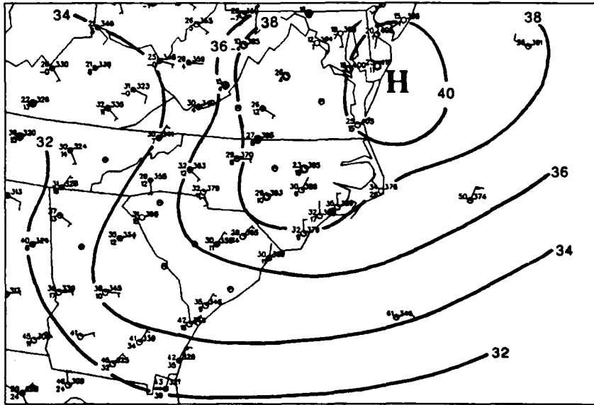
Fig. 6.2. Surface pressure analysis valid at 0000 UTC, 23 January 1984.
