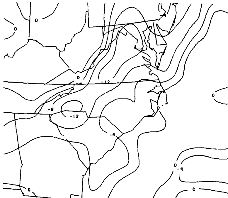
Fig. 12.12. Analysis of the Laplacian of sea level pressure valid at 0000 UTC 25 January 1986. Values given are \times 10^{11} mb m^{-2} , and the contour interval is four units.
