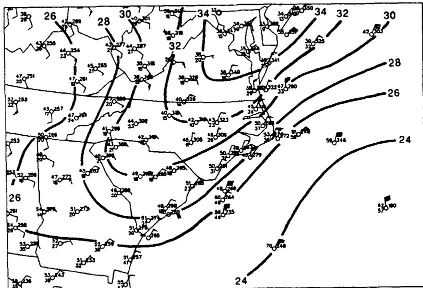
Fig. 6.10. Surface pressure analysis valid at 1800 UTC 24 January 1986.
