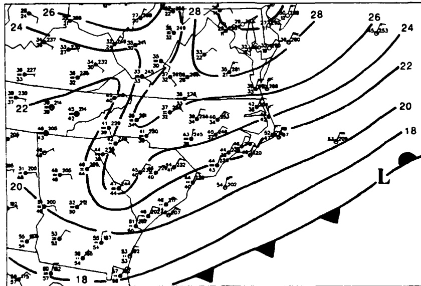
Fig. 6.17. Surface pressure analysis valid at 1500 UTC 17 January 1986.
