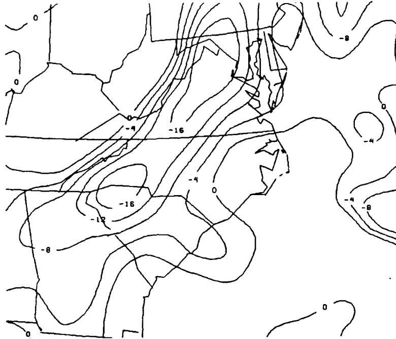
Fig. 12.13. Analysis of the Laplacian of sea level pressure valid at 0600 UTC 25 January 1986. Values given are \times 10^{-11} \text{mb m}^{-2} , and the contour interval is four units.
