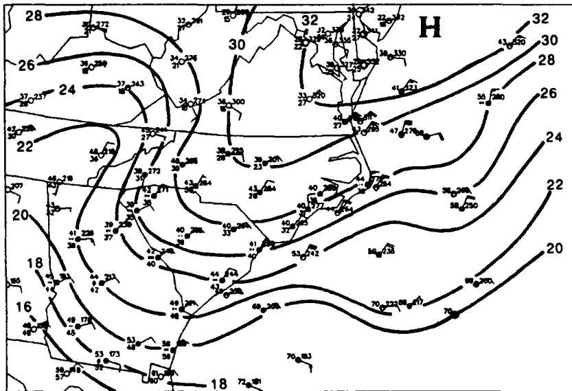
Fig. 6.24. Surface pressure analysis valid at 0600 UTC 23 March 1989.
