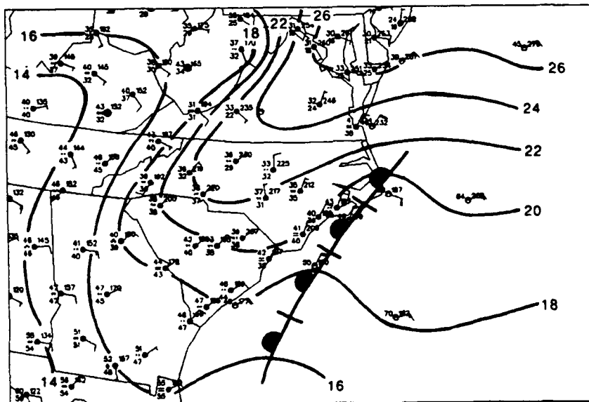
Fig. 6.19. Surface pressure analysis valid at 0600 UTC 18 January 1987.
