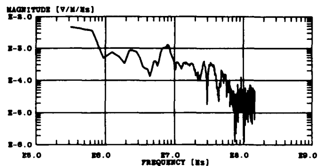
Figure B-3. Measured electric field components, magnitude and amplitude, at location (0, 0, 5): (a) radial (x-components), (b) horizontal (y-components), and (c) vertical (z-components).
