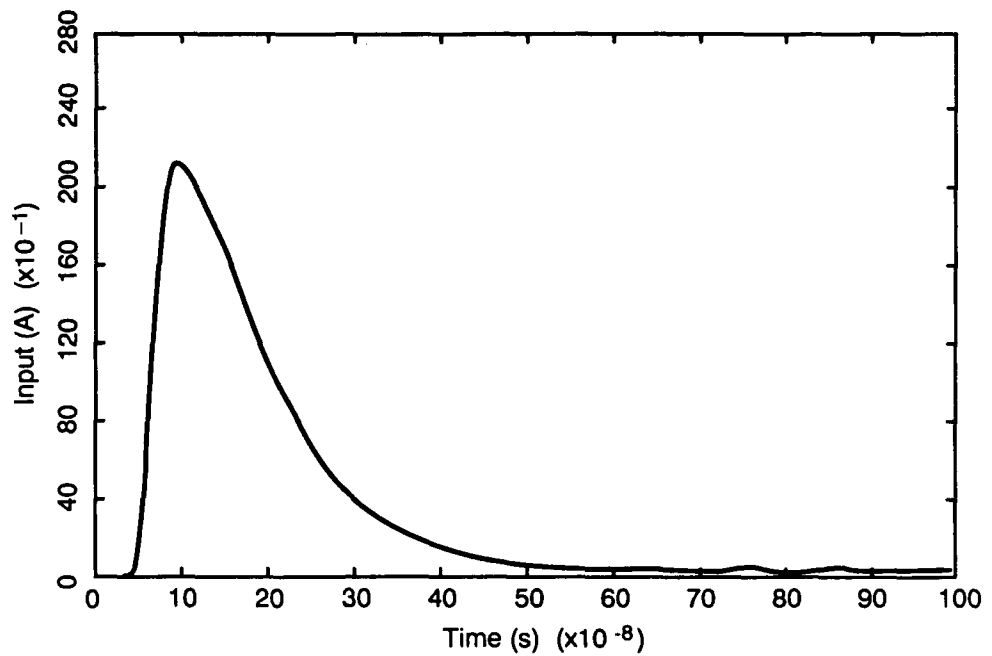
Figure 20. Measured TPD input current for a 50- \Omega line.
