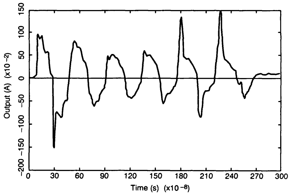
Figure 21. Measured residual current for a 50- \Omega load.
