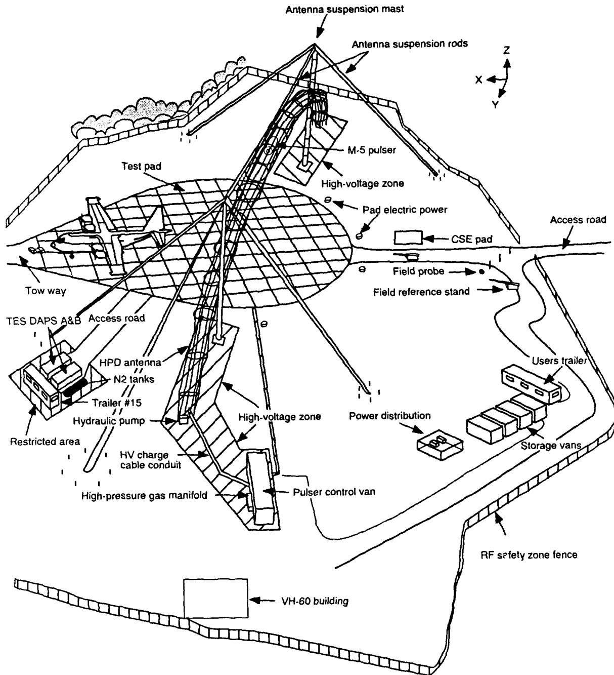
Figure 11. TACAMO EMP simulator.
