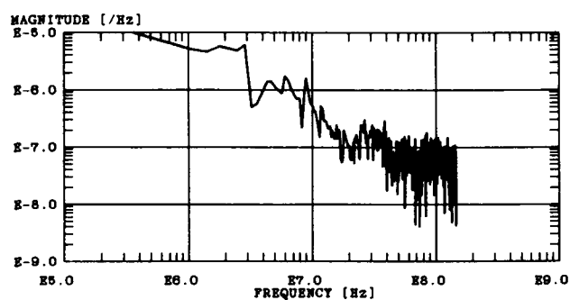
Figure A-10. Measured currents at location (-60, 0, 5): (a) antenna current and (b) coupler ground cable current.
