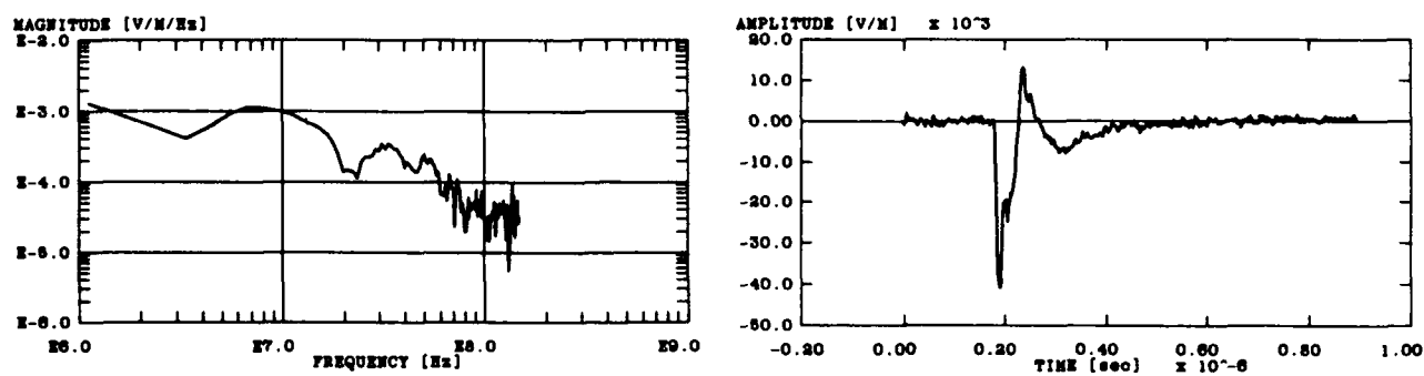
Figure B-4. Measured horizontal electric field (y-component) at location (6, 0, 9).
