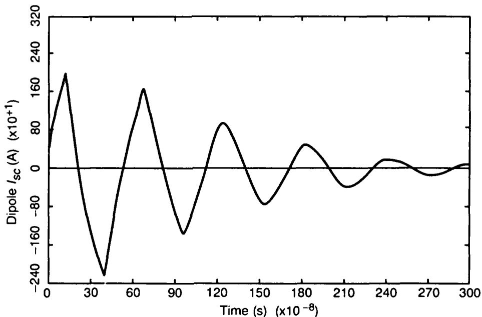
Figure 5. HEMP response of a 46-m free-space dipole.
