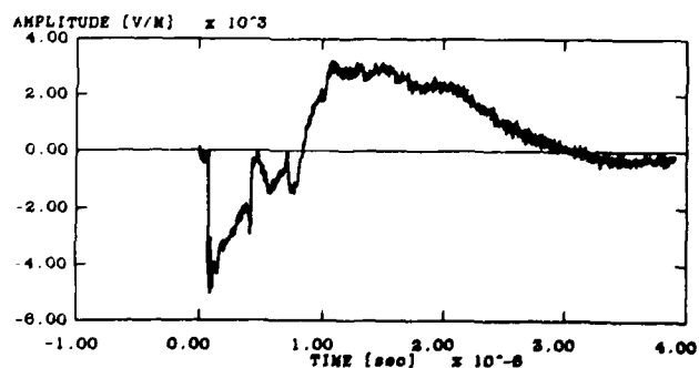
Figure A-6. Measured horizontal electric field (y-component) at locations: (a) (80, 20, 1) and (b) (80, 0, 0).
