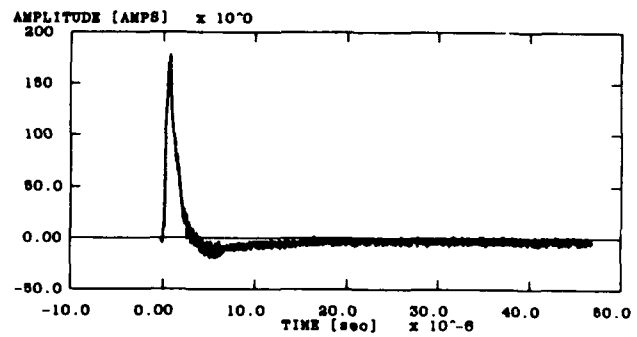
Figure B-9. Measured ac power bulk cable current in test configuration IB: (a) before power line protector and (b) after power line protector.
