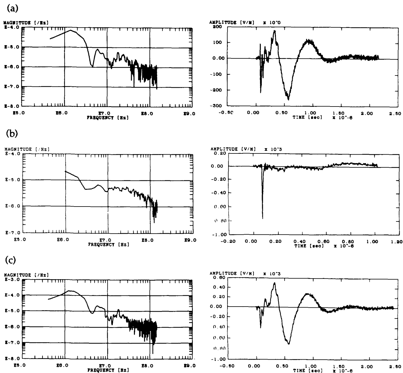
Figure A-1. Measured electric field components, magnitude and amplitude, at location (200, 30, 1): (a) radial (x-component), (b) horizontal (y-component), and (c) vertical (z-component).
