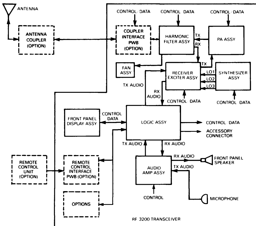
Figure 2. RF-3200 interconnect diagram.
