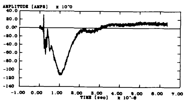
Figure B-14. Measured ground strap current: (a) at the coupler and (b) at the transceiver.
