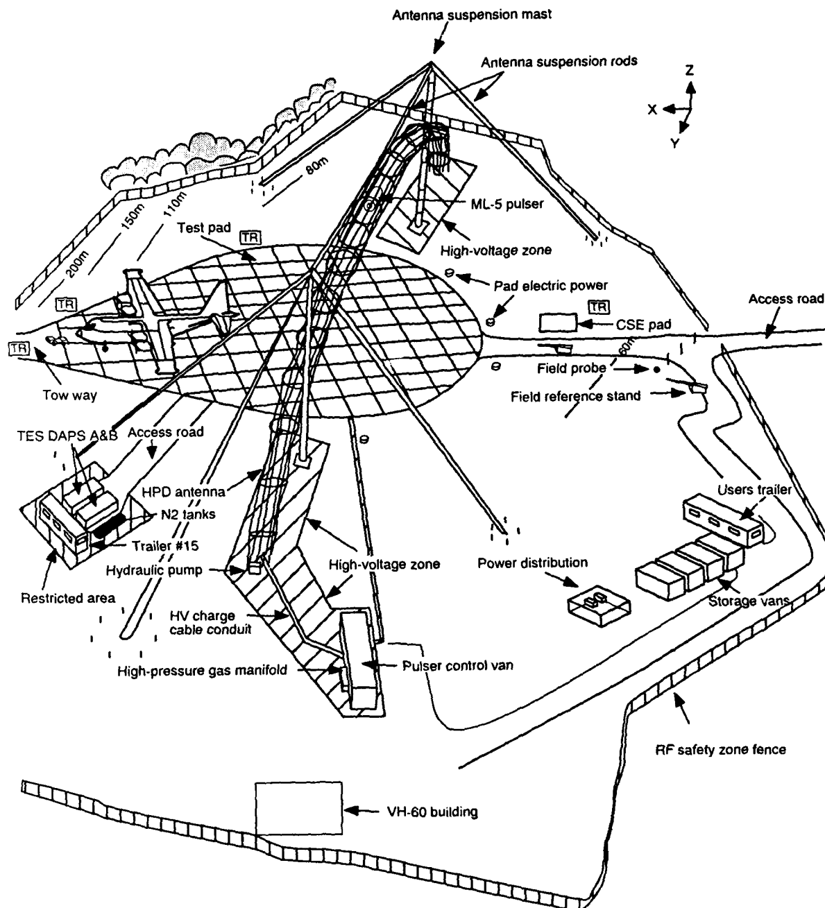
Figure 12. Test configuration for the unhardened RF-3200 system.
