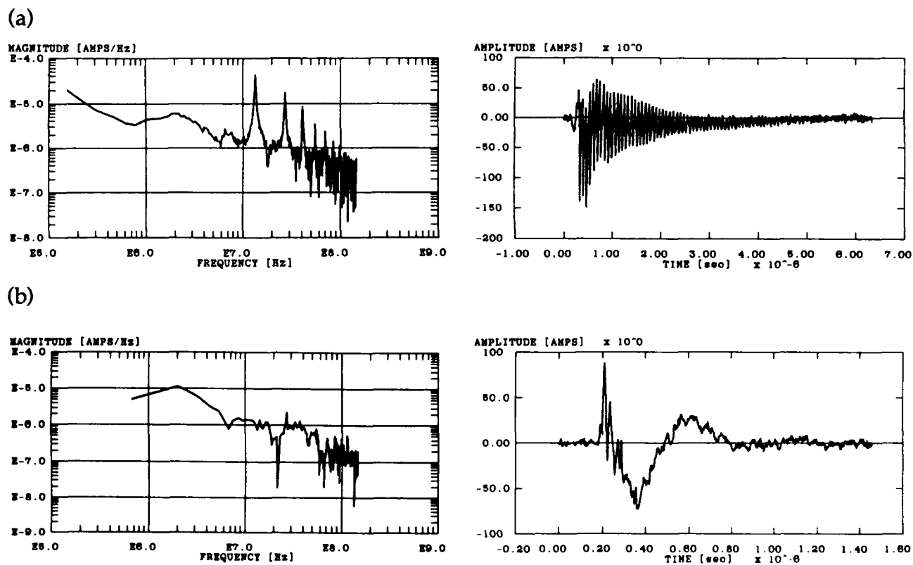
Figure B-5. Measured RF-1912 antenna current: (a) both leads shorted, one lead measured, and (b) both leads shorted, both leads measured.
