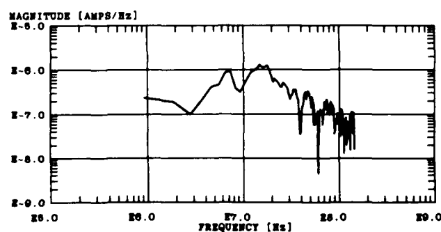
Figure B-12. Measured microphone bulk cable current: (a) dynamic microphone and (b) electret microphone.
