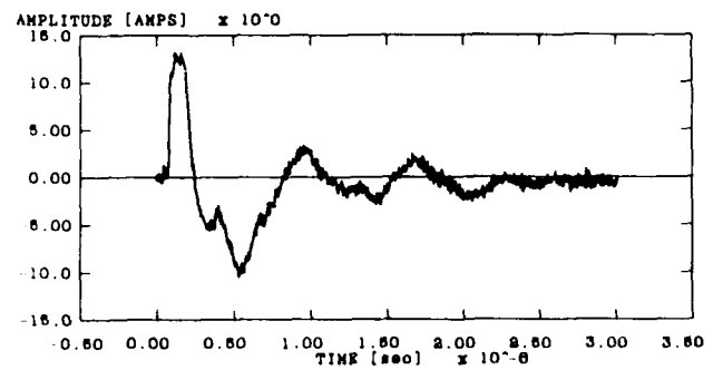
Figure A-5. Measured antenna current at locations: (a) (150, 10, 0), and (b) (110, 10, 0).
