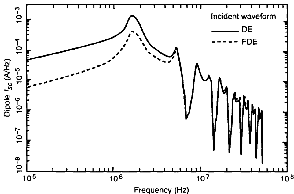
Figure 9. Free-space dipole spectral response comparison for DE and FDE incident pulses.
