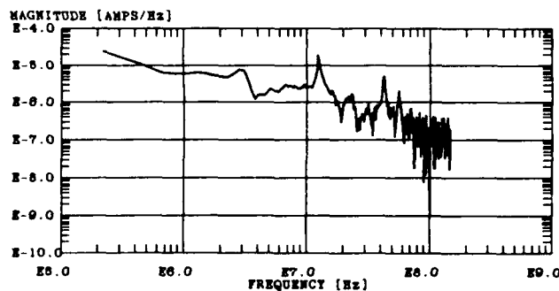
Figure B-5 (cont'd). Measured RF-1912 antenna current: (c) coupler terminated into 50 \Omega (shot #16839), (d) coupler terminated into 50 \Omega (shot #16840), and (e) coupler terminated into transceiver.
