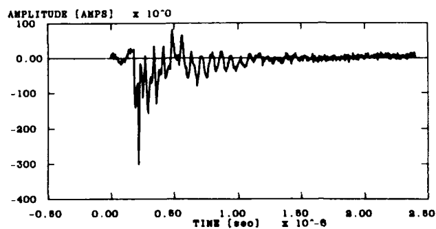
Figure B-7. Measured RF-1940 and RF-1912 combined antenna current: (a) magnitude and (b) amplitude.
