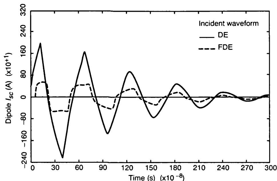
Figure 10. Free-space dipole transient response comparison for DE and FDE incident pulses.
