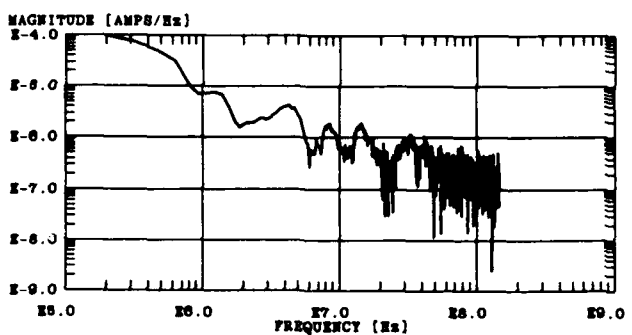
Figure B-14. Measured ground strap current: (a) at the coupler and (b) at the transceiver.
