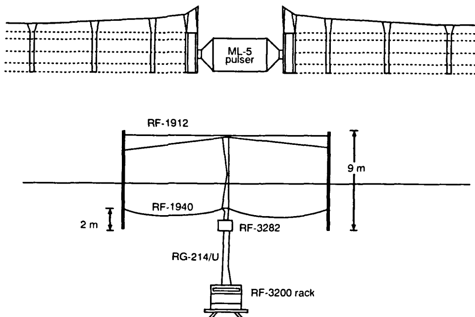
Figure 17. Test configuration IB with the transceiver.
