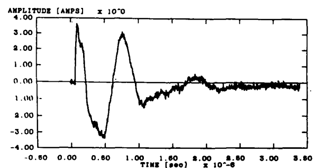
Figure A-3. Measured antenna current at location (200, 10, 0): (a) with the antenna coupler and (b) without the antenna coupler.
