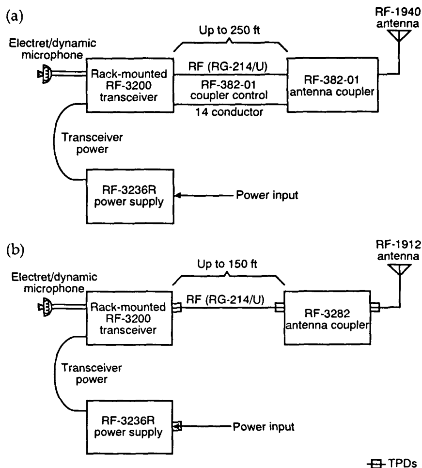
Figure 1. Typical configuration for the (a) unhardened RF-3200 system and (b) hardened RF-3200 system.
