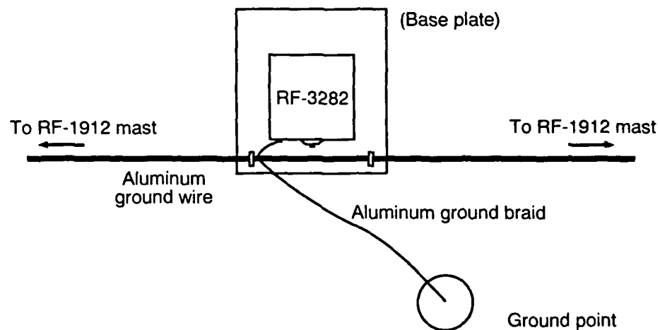
Figure 15. RF-1912 antenna and RF-3282 coupler ground connections.
