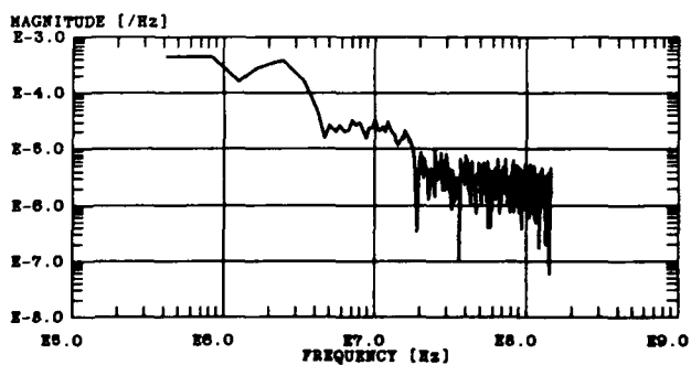
Figure A-2. Measured electric field components, magnitude and amplitude, at location (200, 10, 0): (a) radial (x-component), (b) horizontal (y-component), and (c) vertical (z-component).
