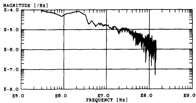
Figure A-4. Measured horizontal (y-component) electric field at locations: (a) (150, 30, 1), (b) (150, 10, 0), and (c) (110, 10, 0).
