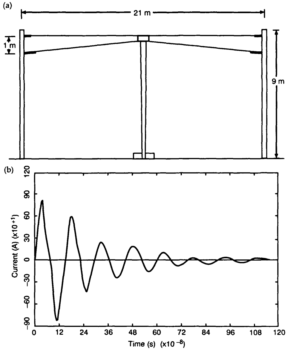
Figure 6. RF-1912 free-space antenna: (a) typical configuration and (b) HEMP induced response.
