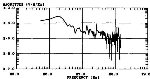
Figure B-2. Measured electric field components, magnitude and amplitude, at location (6, 0, 1): (a) radial (x-components), (b) horizontal (y-components), and (c) vertical (z-components).
