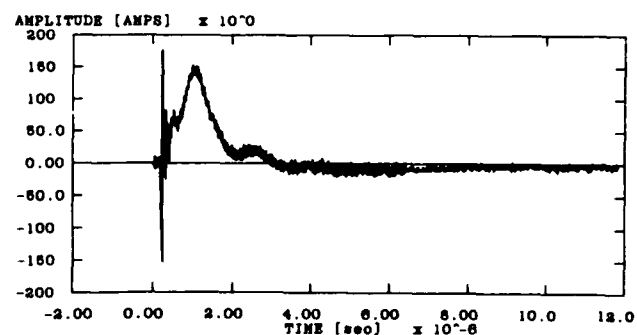
Figure B-10. Measured ac power bulk cable current in test configuration II: (a) before power line protector and (b) after power line protector.
