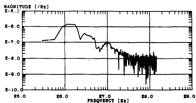
Figure A-3. Measured antenna current at location (200, 10, 0): (a) with the antenna coupler and (b) without the antenna coupler.
