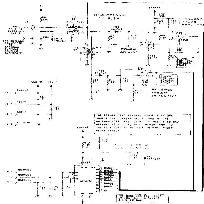
Figure 13. Harmonic filter PWB A4 schematic diagram.
