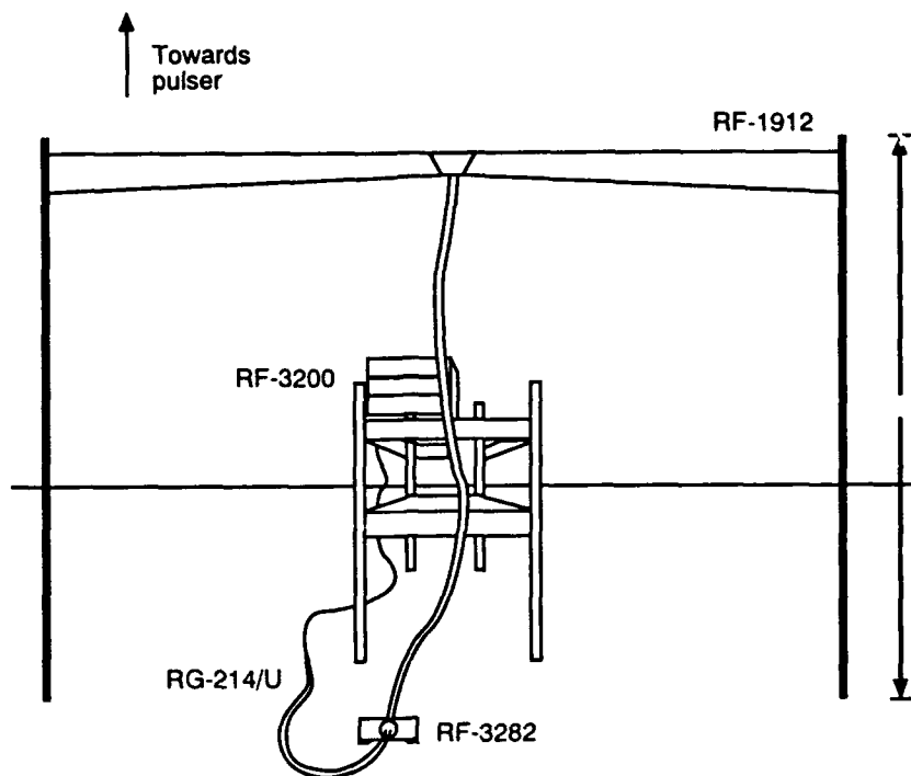
Figure 18. Test configuration II for the hardened system.
