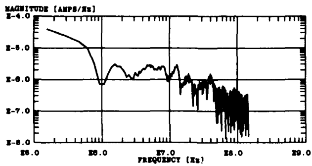
Figure B-13. Measured RG-214/U coaxial cable shield current in test configuration II: (a) at the coupler and (b) at the transceiver.
