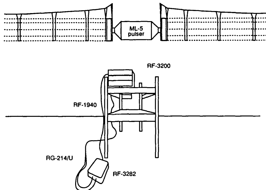
Figure 19. Test configuration III for the hardened system.
