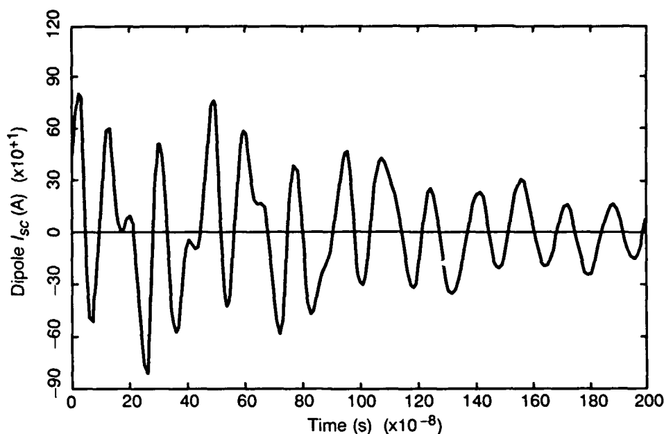
Figure 8. HEMP response of a 46-m dipole at a height of 2 m.
