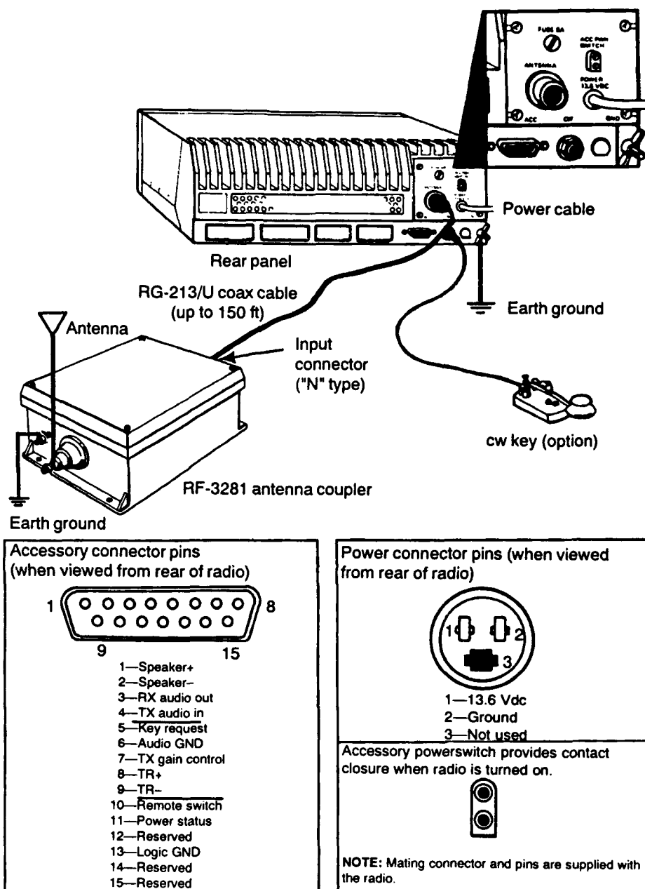
Figure 4. RF-3200 rear panel connections.
