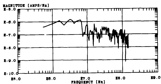
Figure B-8. Measured RG-214/U coaxial cable current in test configuration IB: (a) shield current and (b) center conductor current.
