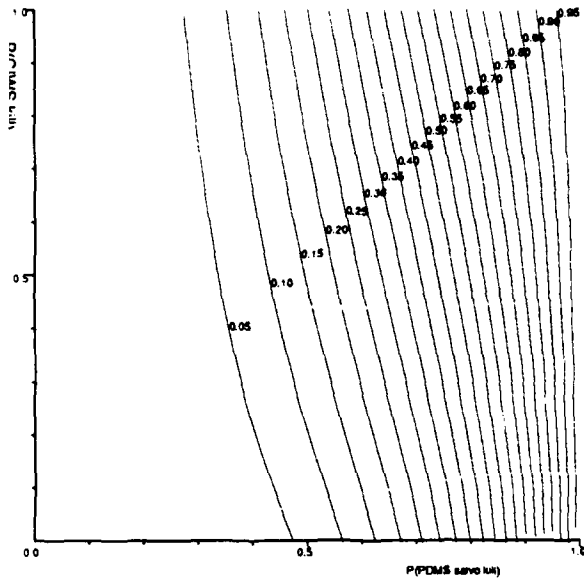
FIGURE 4(a) PROBABILITY CONTOURS OF ALL FOUR ASCMs BEING KILLED FOR SHIP DEFENDED BY PDMS AND SINGLE CIWS
