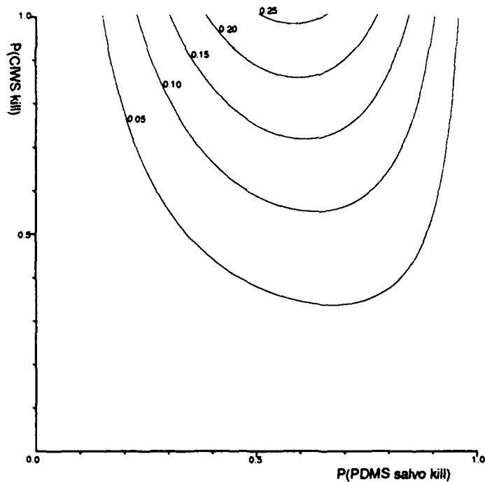
FIGURE 4(c) CONTOURS OF IMPROVEMENT IN PROBABILITY OF KILLING ALL FOUR ASCMs WHEN SECOND CIWS IS ADDED TO SHIP WEAPONS SYSTEMS
