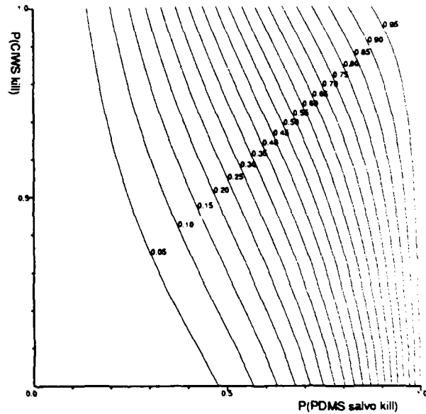
FIGURE 4(b) PROBABILITY CONTOURS OF ALL FOUR ASCMs BEING KILLED FOR SHIP DEFENDED BY PDMS AND TWO CIWS
