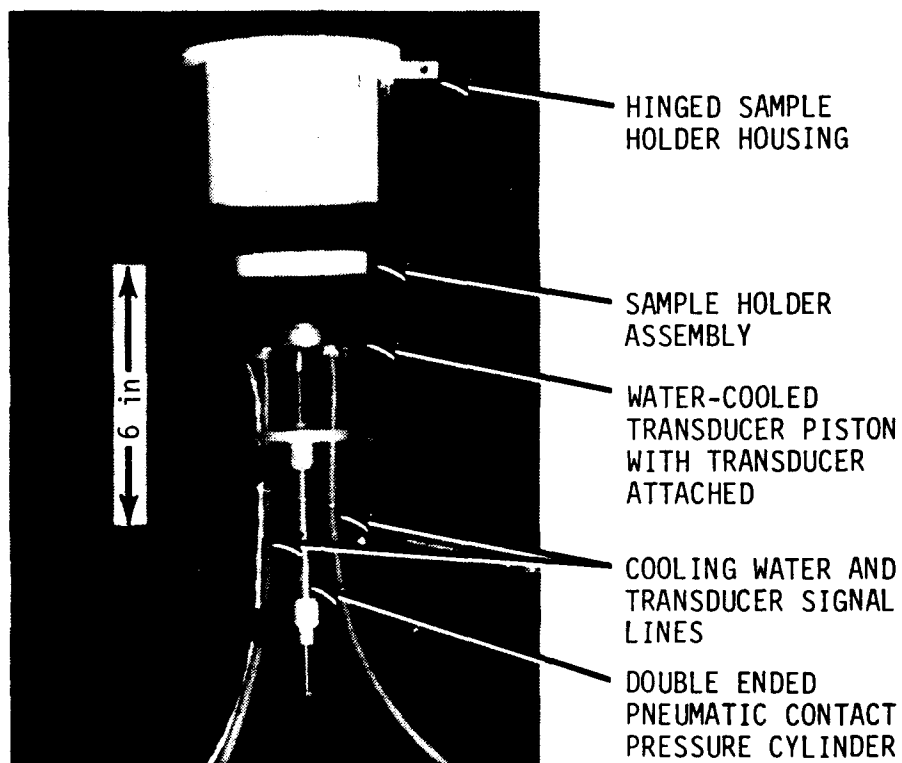
Figure 10. Disassembled Sample Holder Housing
