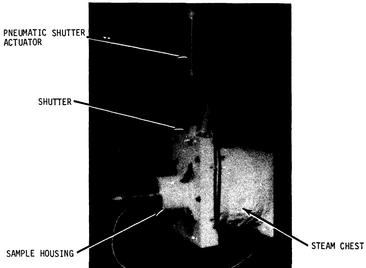
Figure 4. Steam Chest
