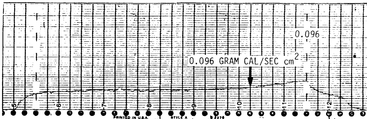
Figure 20. Heat Flux through Aluminized Fabric, Aluminum Side Exposed to the Steam
