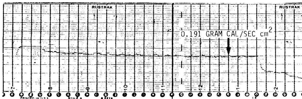
Figure 22. Heat Flux into Transducer without Sample
