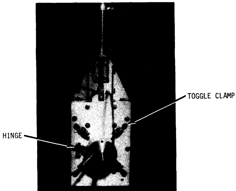
Figure 9. Sample Holder Housing Clamped to Steam Chest
