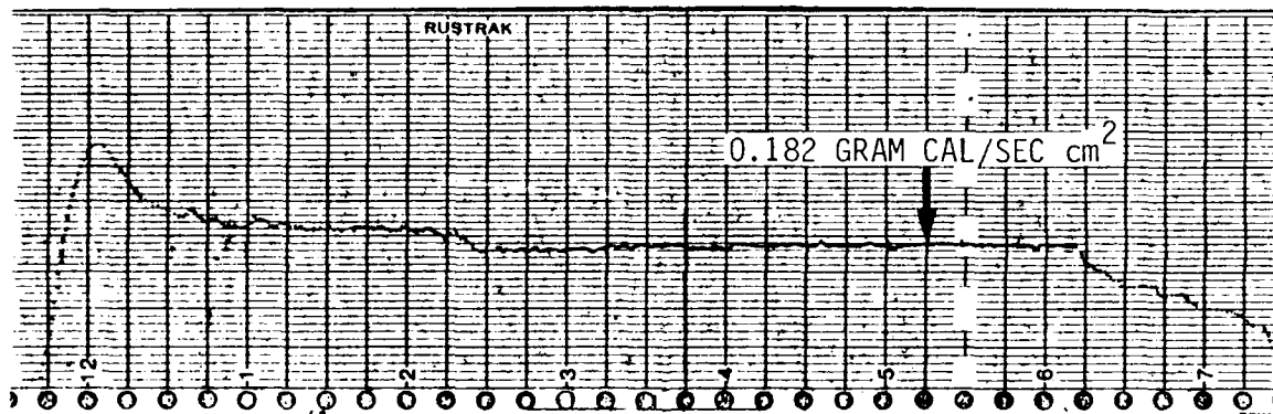
Figure 21. Heat Flux through Denim
