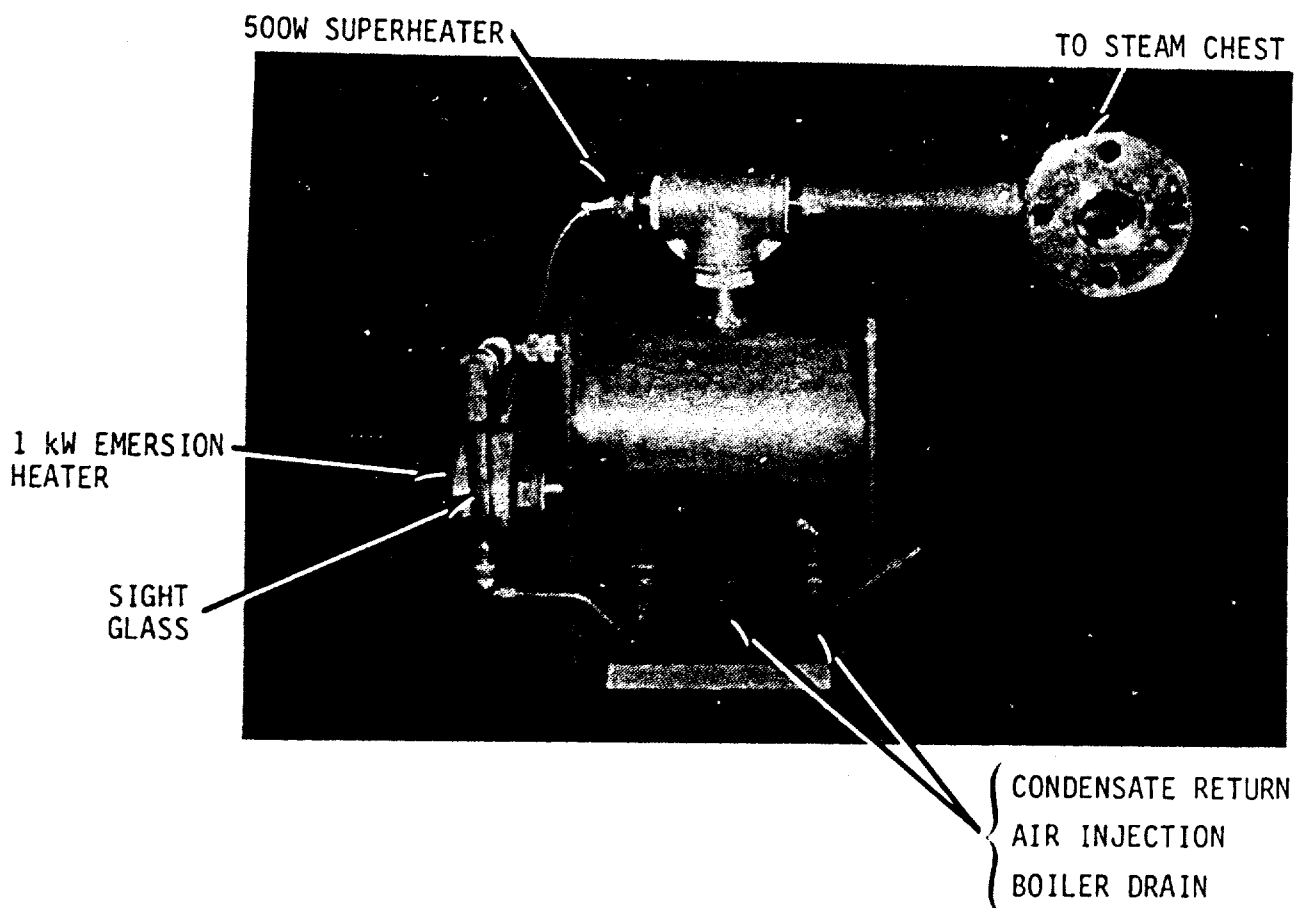
Figure 3. Boiler with Superheater
