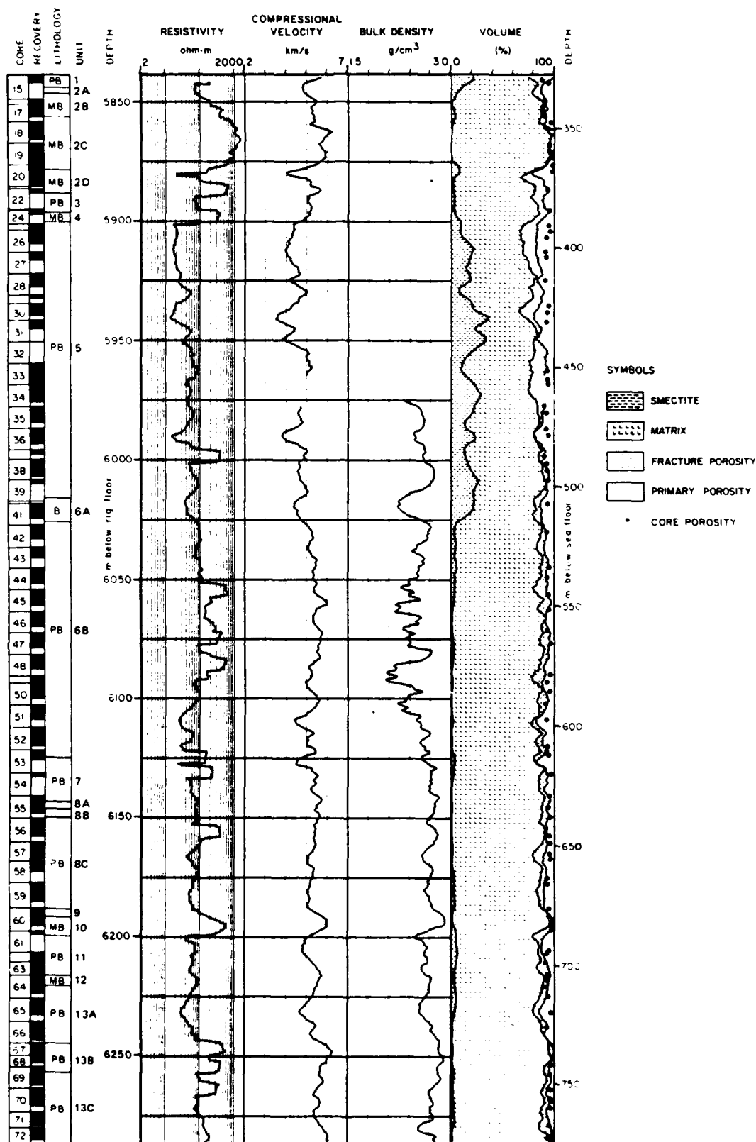
Figure 32. Computed smectite volume, total porosity, and primary porosity in Hole 418A from Broglia and Moos (1988).
