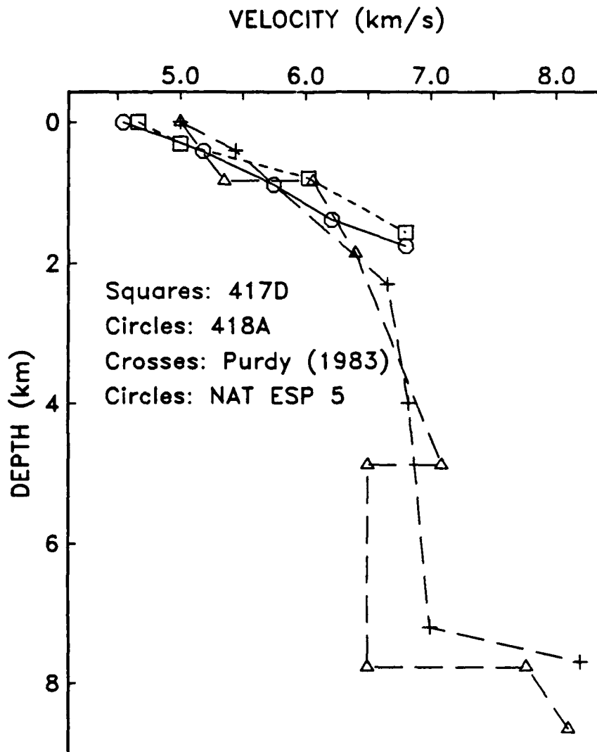
Figure 4. Compressional velocities from tau-zeta in version of oblique seismic experiment travel times for Holes 417D (Stephen and Harding, 1983) and 418A (Swift and Stephen, in press). Also shown are full crustal velocity profiles from ESP 5 of the NAT (Mithal, 1986) and from Purdy's (1983) study of 140 Ma crust.
