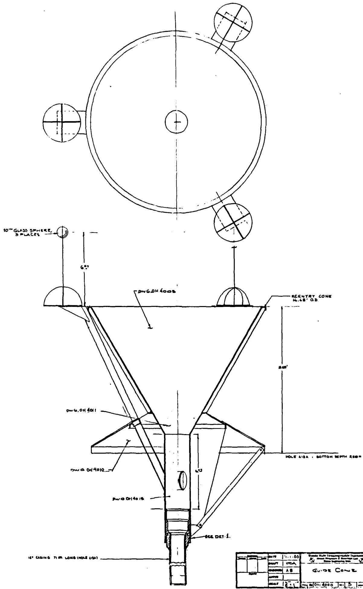
Figure 45. The dimensions of the re-entry cone at Hole 418A are given as interpreted by A. Boconcelli and R. Stephen at WHOI in 1988.
