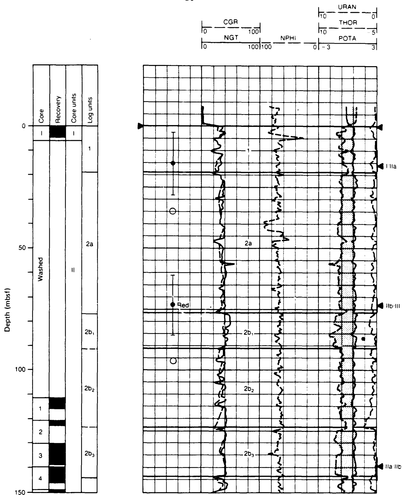
Figure 29. Gamma ray logs in sediment section of Hole 418A from Carlson et al. (1988b).
