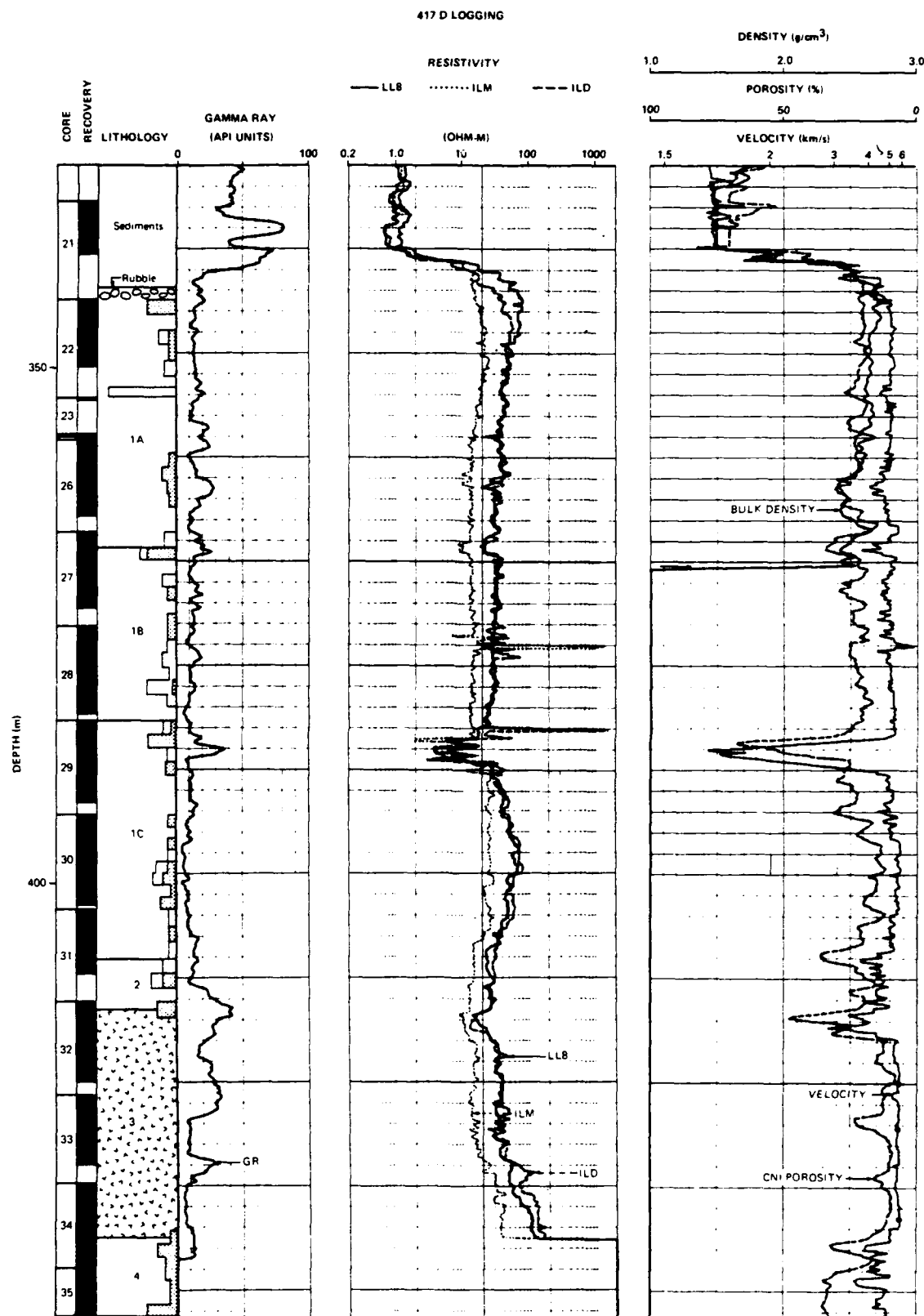
Figure 26. Corrected logs for basement section in Hole 417D. From Salisbury et al (1980b).
