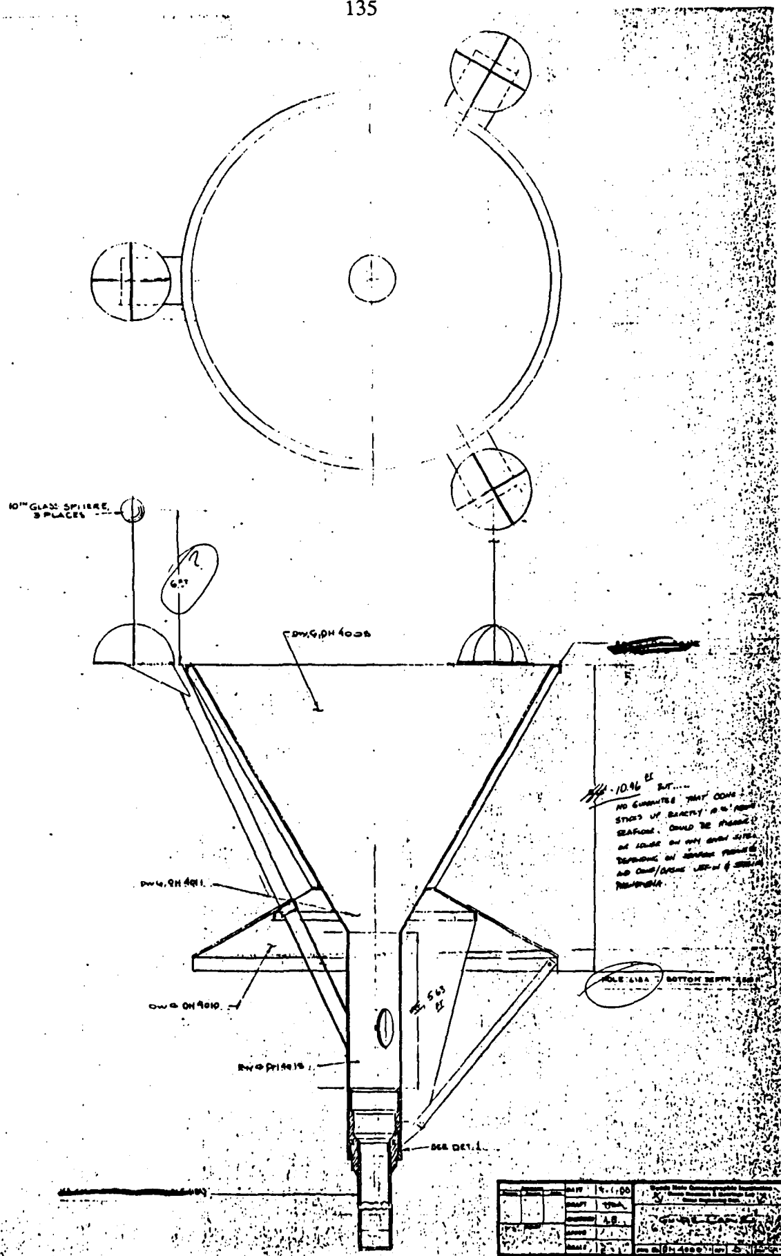
Figure 47. This is the same as Figure 45 but with annotations by Dave Huey of ODP in 1988. The changes reflect the uncertainty at this time in the cone dimensions.
