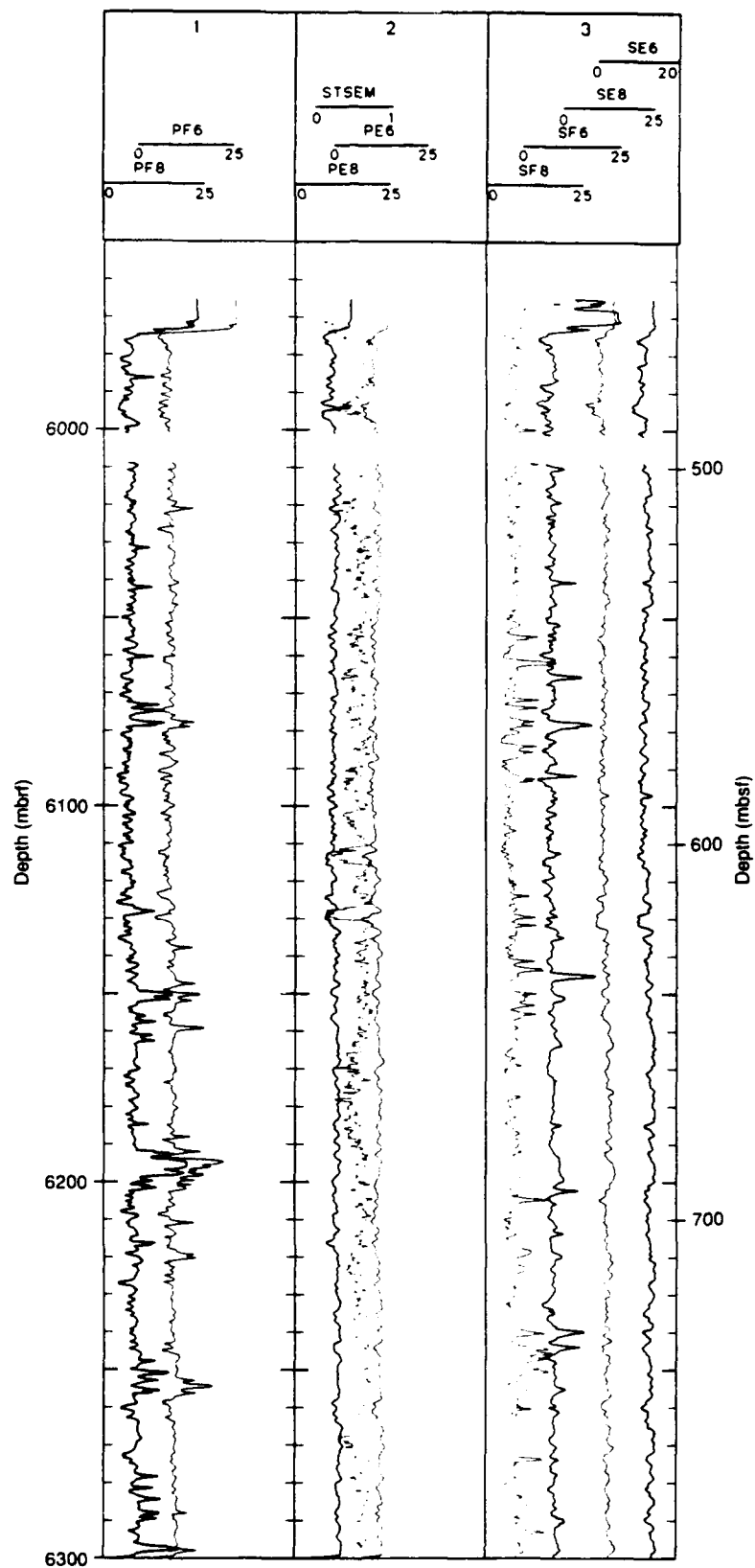
Figure 35. Peak frequency and energy in P and S waves in Hole 418A from Moos (1988).
