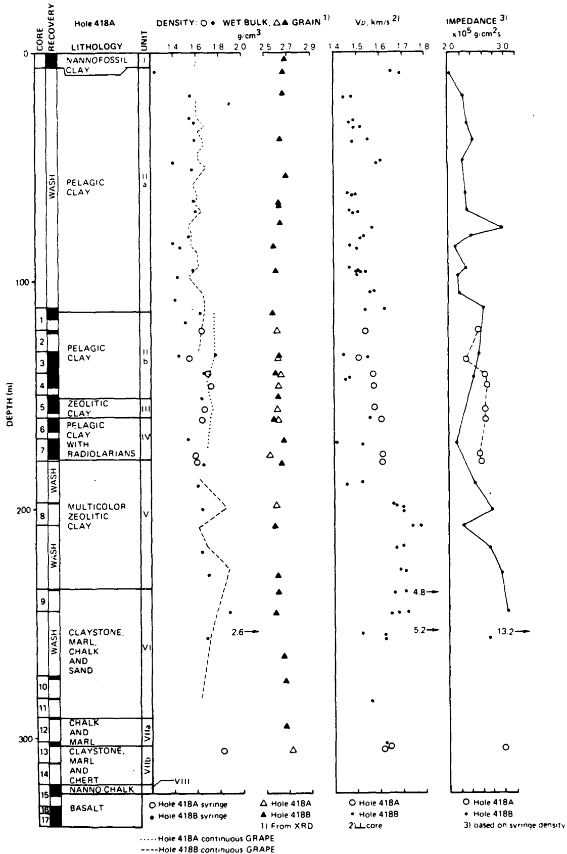
Holes 418A and 418B: Physical properties of sediment.
