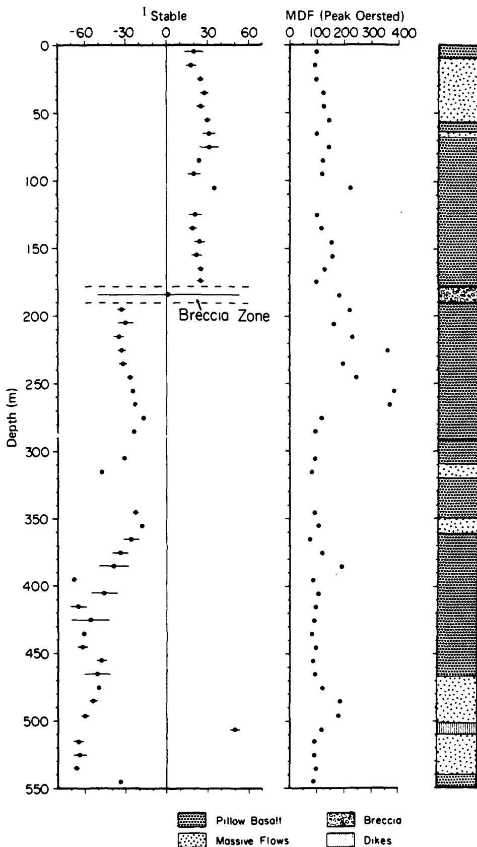
Downhole variation of I_{\text{Stable}} and MDF for Hole 418A. All else is as in Figure 3.
