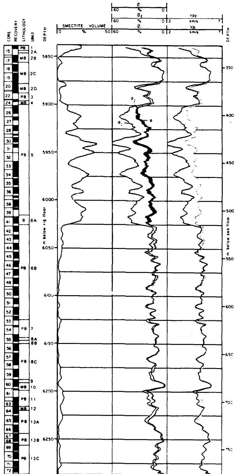
Figure 33. Upper and lower limits on the original basalt porosity and velocity computed from log data in Broglia and Moos (1988).
