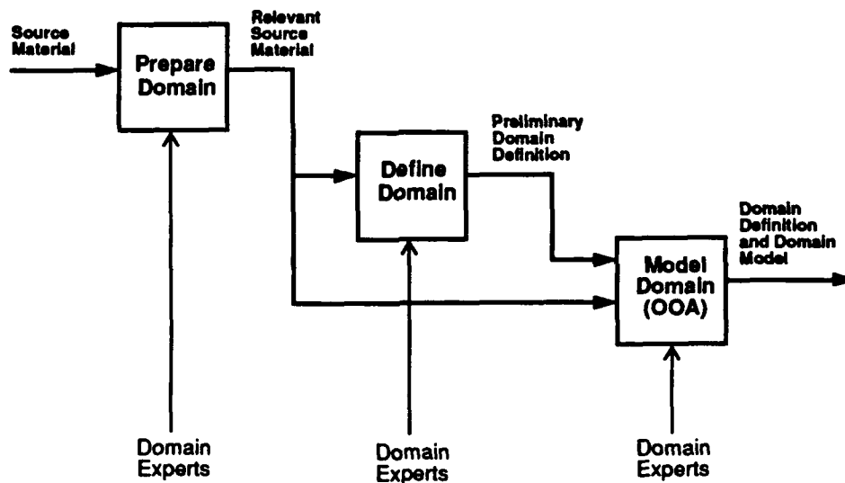
Figure 3-1 Domain Analysis Process
