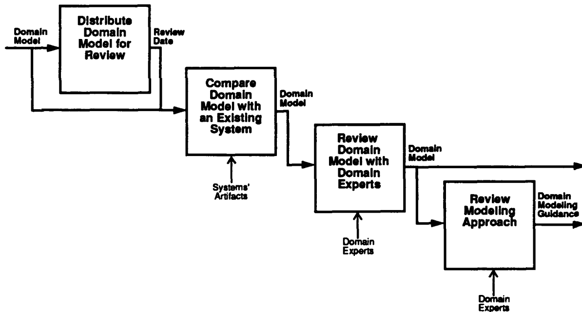
Figure 7-2 Domain Model Review Process
