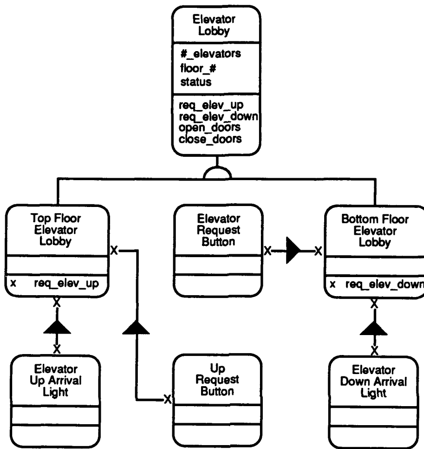
Figure A-10 Elevator Lobby Classification Structures
