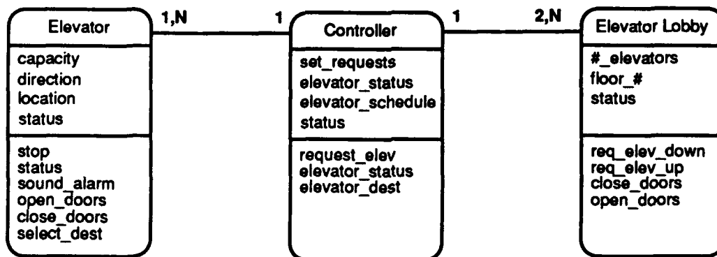
Figure A-13 Controller for the Office Building Elevator System
