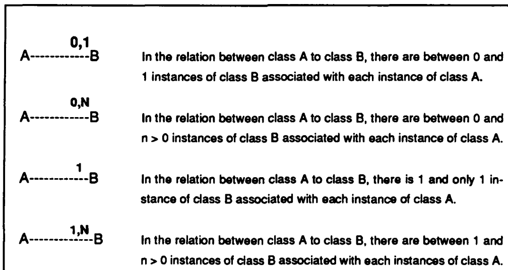
Figure C-3 Instance Connection Constraint Notion
