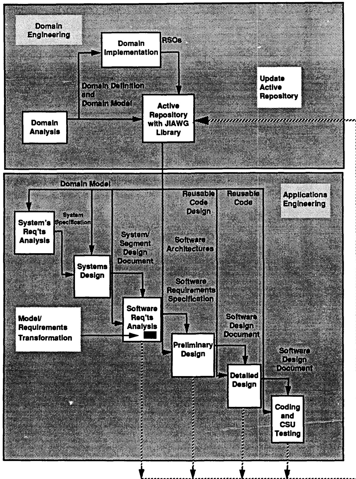
Figure 2-2 Applications Engineering Based on Domain Engineering
