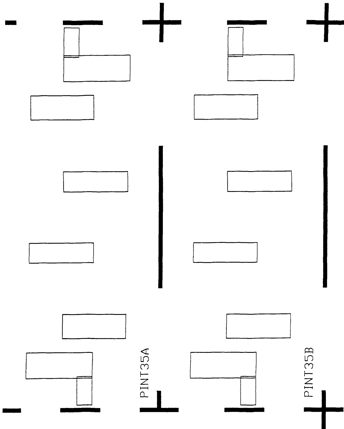
Fig. 14. Interdigitated 35 GHz Filter
