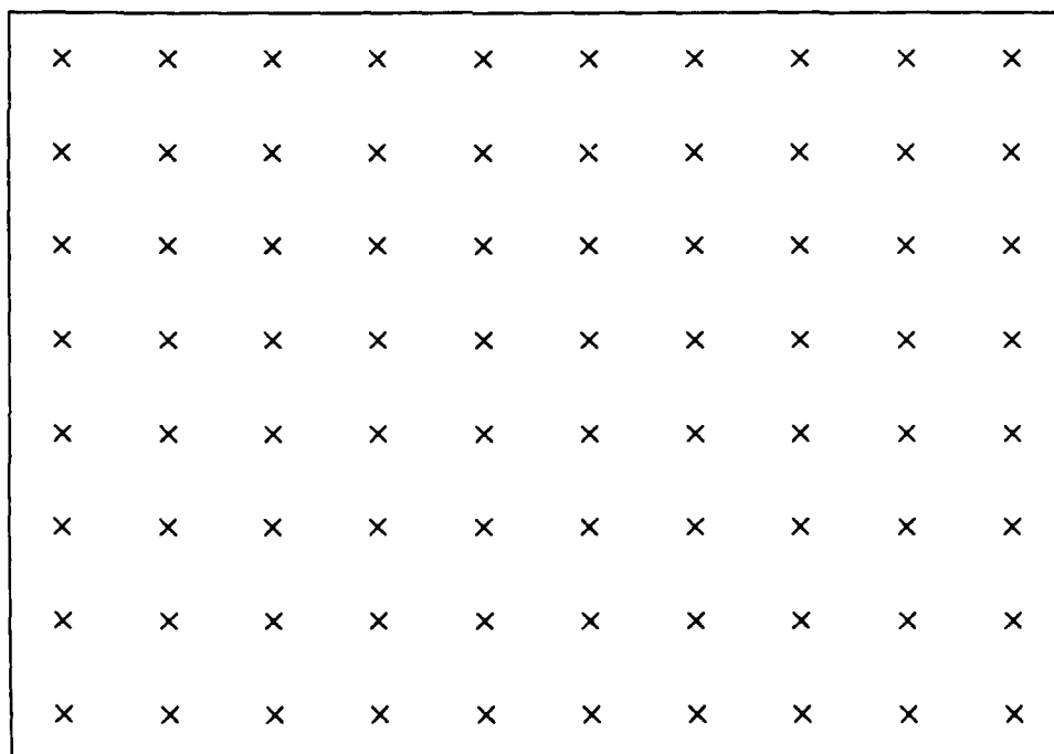
Figure B-1. Centers of pixels on hexagonal (top) and rectangular (bottom) 8 \times 10 grids with identical row and column separation.
