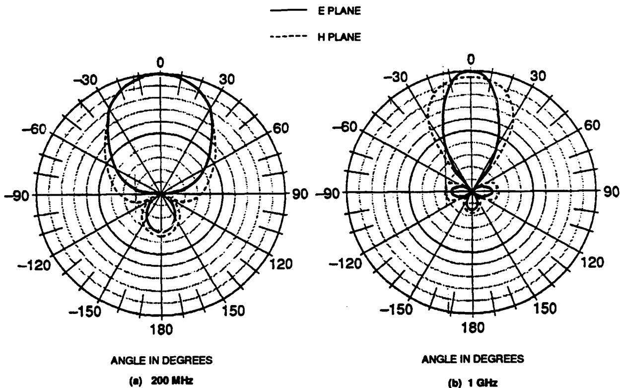
FIGURE 1 E- AND H- PATTERNS OF BROADBAND HORN AT 200 MHz AND 1 GHz
