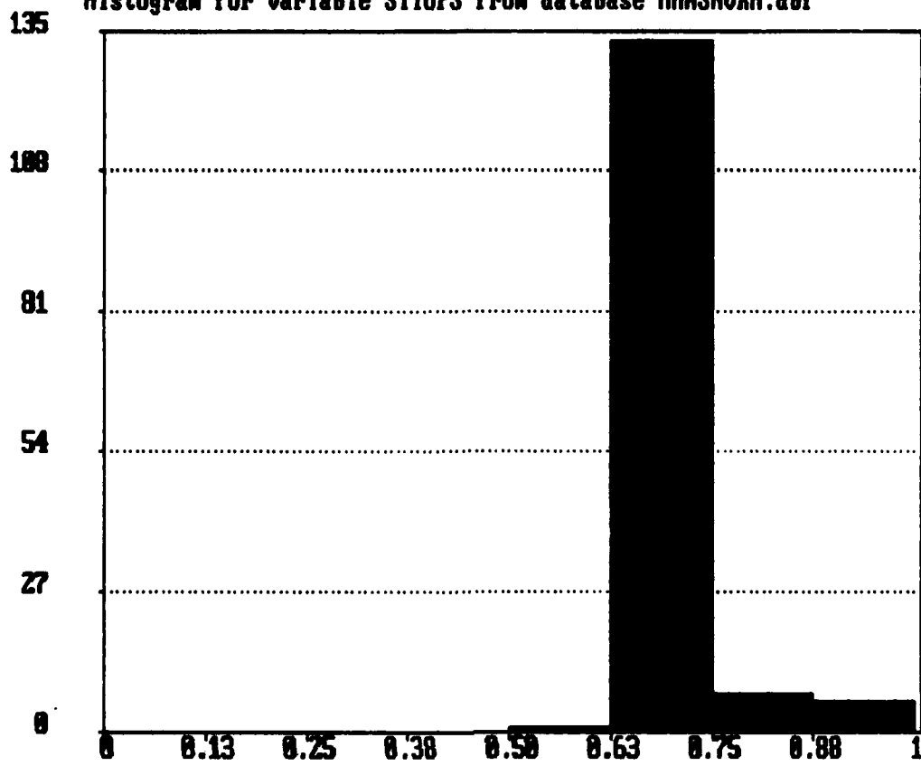
Histogram for variable SITUPS from database MMASNORM.dbf
