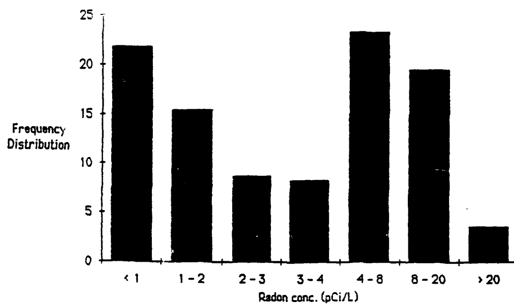
Figure 13 Andersen AFB Radon Distribution
