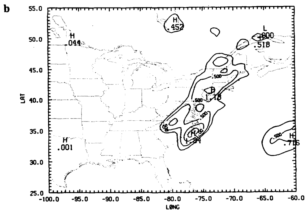
Figure 5.2. Forecasts of accumulated total precipitation in cm (26/00Z - 26/06Z) originating from (a) DVMI and (b) AVMI. (c) Observed precipitation in cm for the same period. Contours at 0.25 cm and every 0.5 cm for 0.5 and above.
