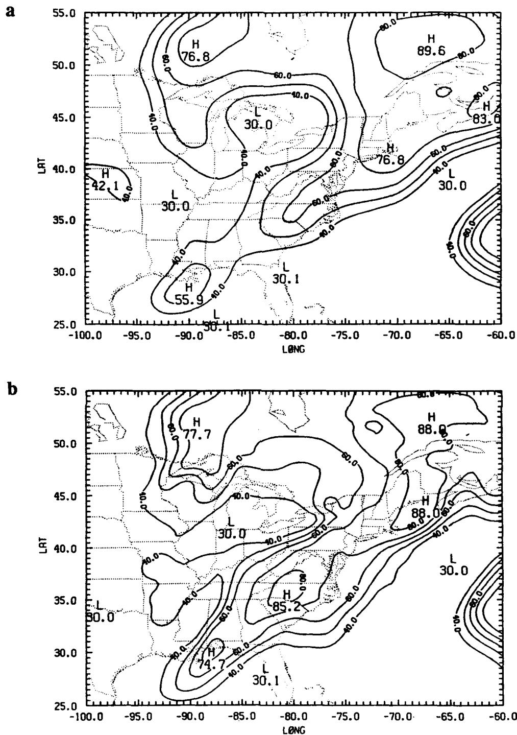
Figure 6.12. 500-mb relative humidity (%) analyses at 26/00Z from (a) experiment 1 (no assimilation), (b) experiment 2 (12DI), (c) experiment 3 (05DI), and (d) experiment 5 (06AI). Contours are every 10%.
