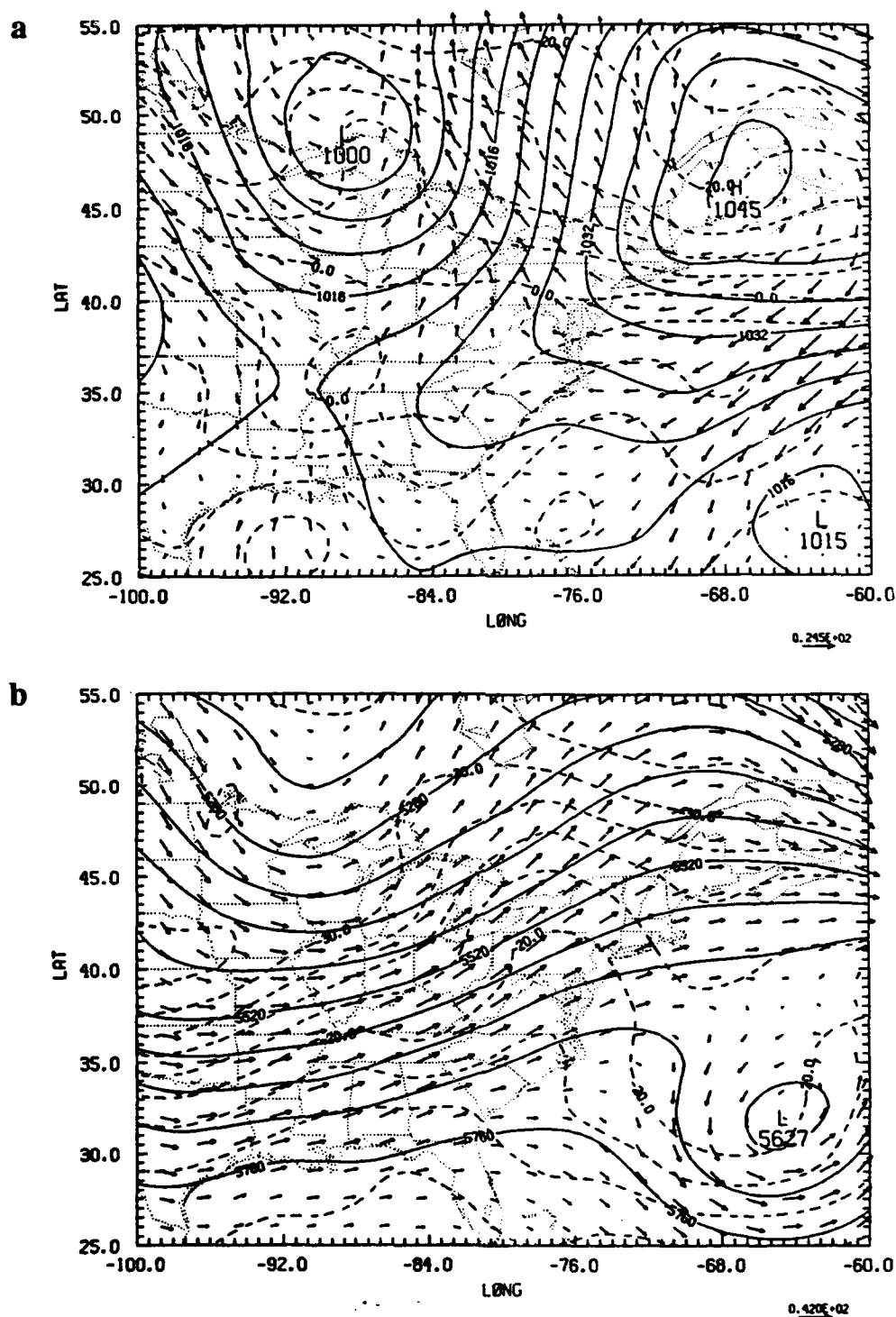
Figure 4.3. (a) Sea-level pressure (mb) and temperature ( ^{\circ} C) and winds at 1000 mb, and (b) geopotential height (m), temperature ( ^{\circ} C) and winds at 500 mb for the NMC analysis on 25/12Z. (c) and (d) as in (a) except for 26/12Z and 27/12Z, respectively. Contours of sea-level pressure and temperature at 1000 mb are 4 mb and 5^{\circ} C, respectively. Maximum wind vector indicated by labelled arrow in m s -1 .
