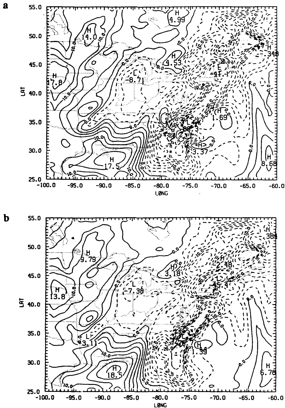
Figure 5.1. 500-mb vertical motion fields valid at 27/00Z: (a) from 12-h forecast of the control (case 5.1), (b) after DVM (case 5.2), and (c) after AVMI (case 5.3). Vertical motion of magnitude of -20 \text{ mb h}^{-1} or more are contoured every 2.5 \text{ mb h}^{-1} .
