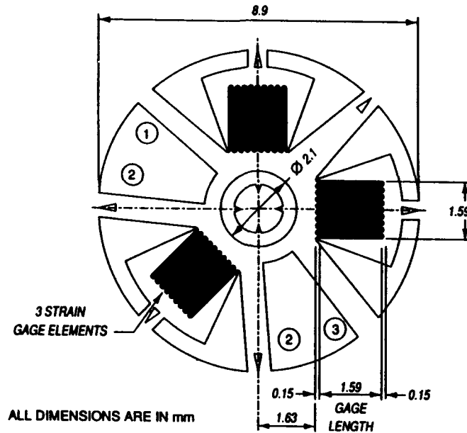
Figure 3. Rosette gage for residual stress measurements, Measurement Group, Inc. (type 062-RE) (all dimensions are in millimetres)
