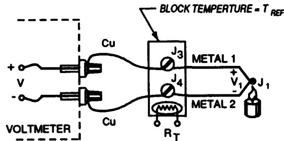
EXTERNAL REFERENCE JUNCTION-NO ICE BATH
