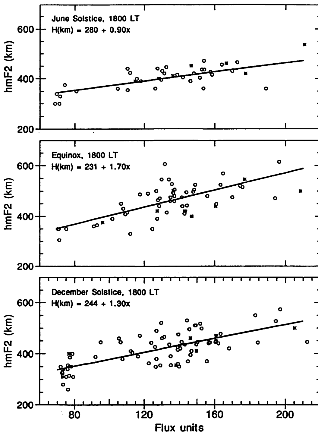
Fig. 37. Seasonal variation of the peak height (hmF2) with flux for 1800 LT. The heavy line is a least squares fit to the scattered quiet-time data (open circles). The formula in the upper left corner corresponds to the least squares fit. The stars denote data obtained under disturbed conditions.
