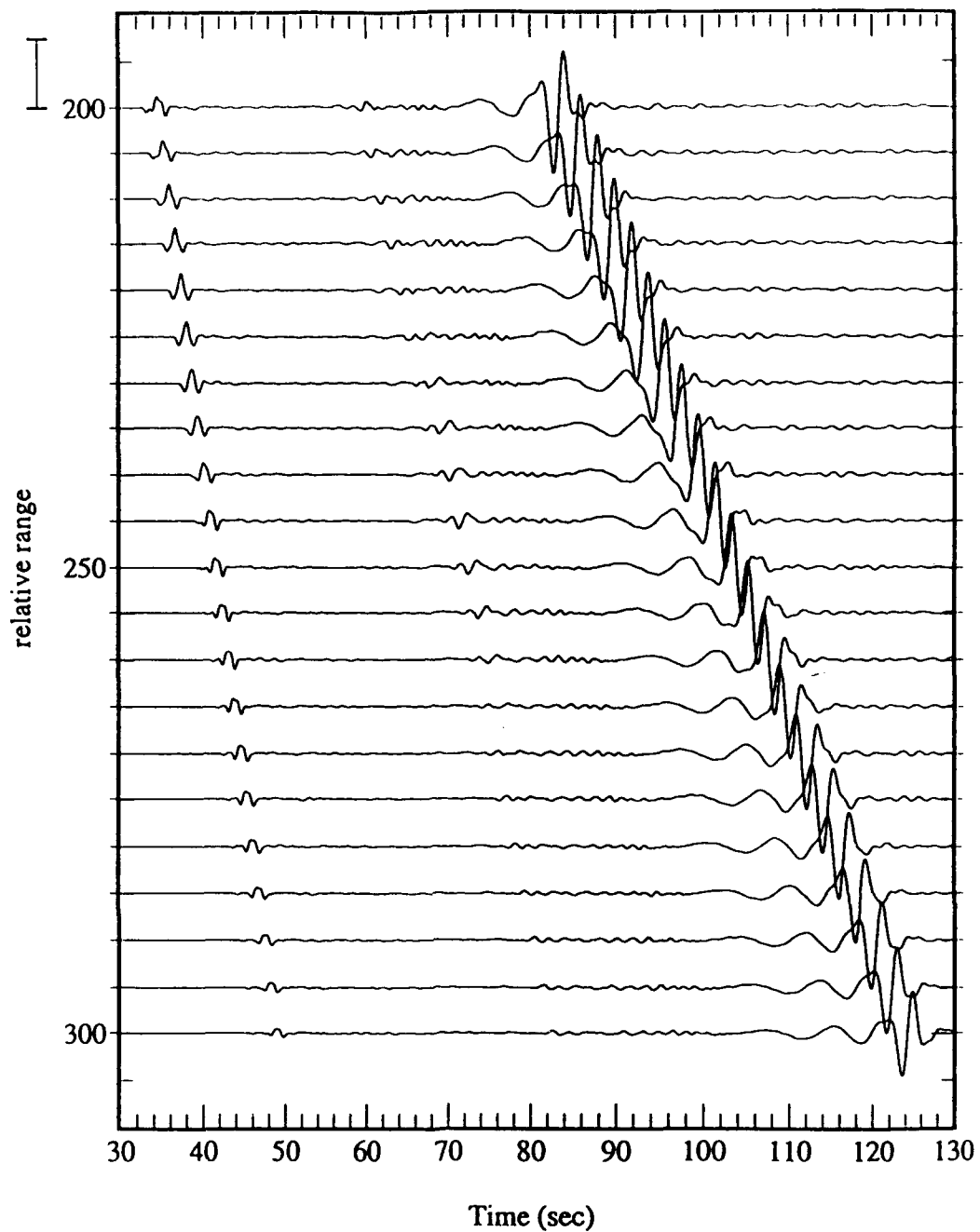
Figure 10-a: Synthetic seismograms for a layered earth with horizontal and vertical randomization of 1km. square segments of the earth structure. The fluctuations very smoothly from 20% at the surface to 3% at a depth of 3km.
