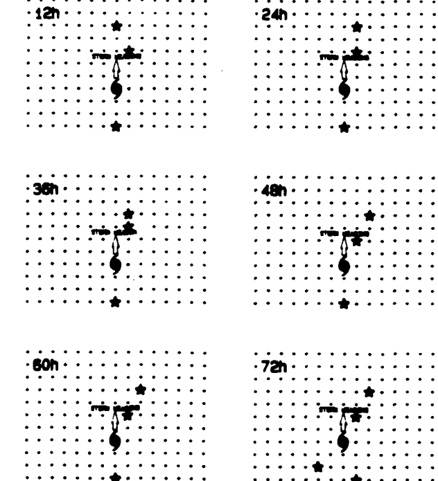
Fig. 11. 15 x 11 grid-layout and geopotential height predictor locations (starred grid-points) for the North-Zone. Perfect-Prog predictor values are averaged over forecast period (see Section 3.7).
