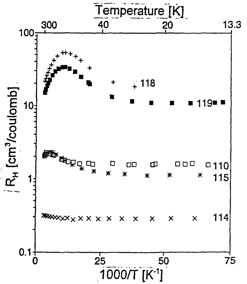
Figure 1 - Hall coefficient vs. 1/T.
