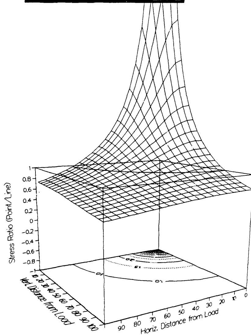
Figure A-3. Ratio of vertical stresses for vertical point and line loads for P/p = 100
