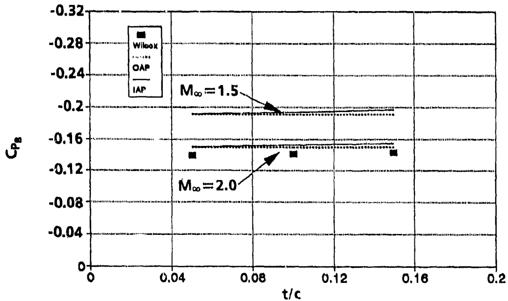
FIGURE 13h. COMPARISON OF BODY-TAIL BASE PRESSURE PREDICTED BY THE OAP AND IAP AS A FUNCTION OF FIN THICKNESS ( \alpha = \delta = 0 ; x/c = 2.0 ; M_\infty = 1.5, 2.0 )
