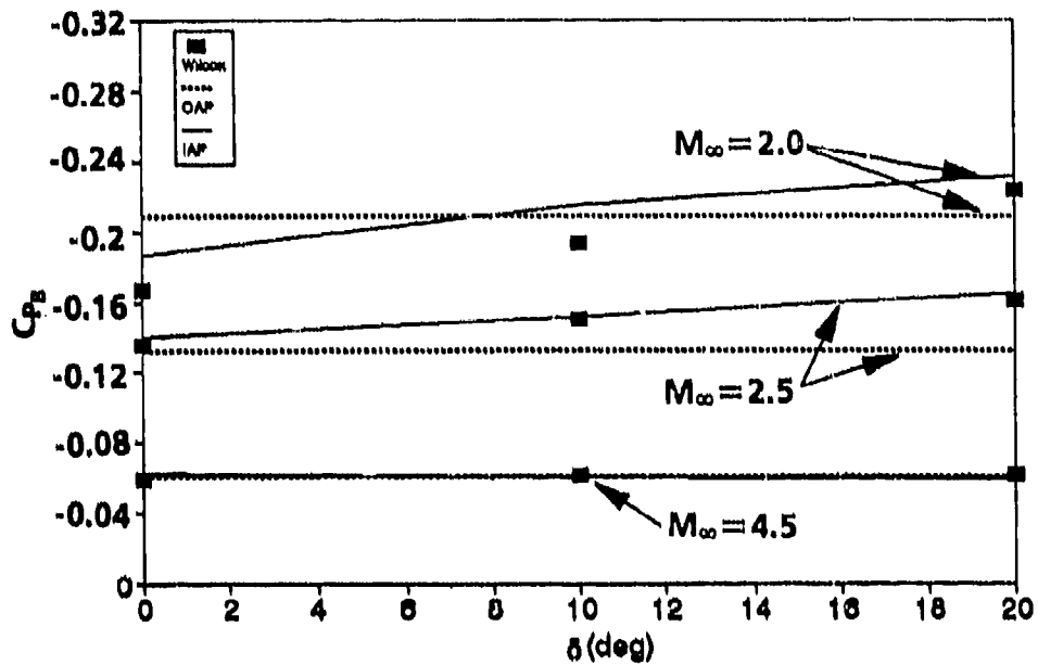
FIGURE 12b. COMPARISON OF BODY-TAIL BASE PRESSURE PREDICTED BY THE OAP AND IAP AS A FUNCTION OF CONTROL DEFLECTION ( t/c=0.15 ; M_\infty=2.0, 2.5, 4.5 ; x/c=0 )
