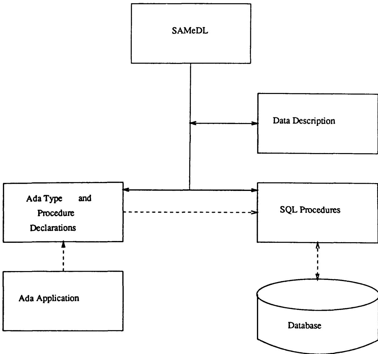
Figure 1-8: The Meaning of a SAMeDL Text
