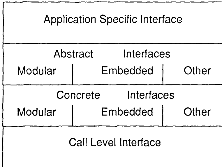
Figure 1-1: Ada SQL Interface Reference Model
