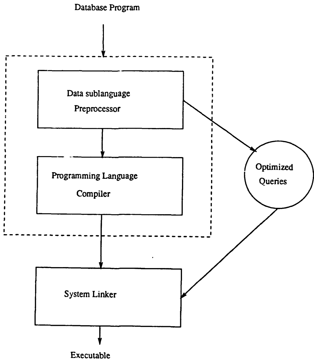
Figure 1-2: The Pre-Compilation Process
