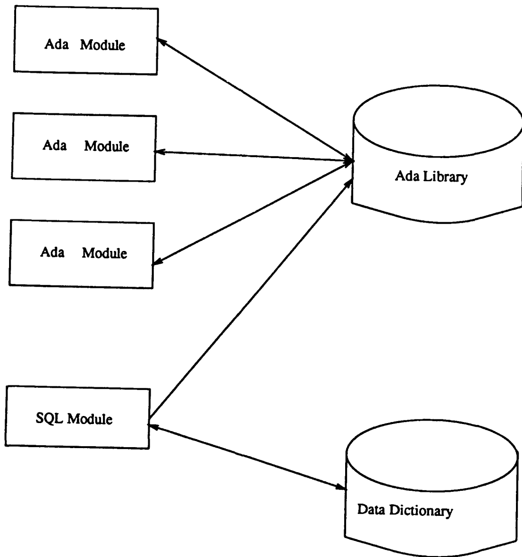
Figure 1-3: Modular Program Architectures
