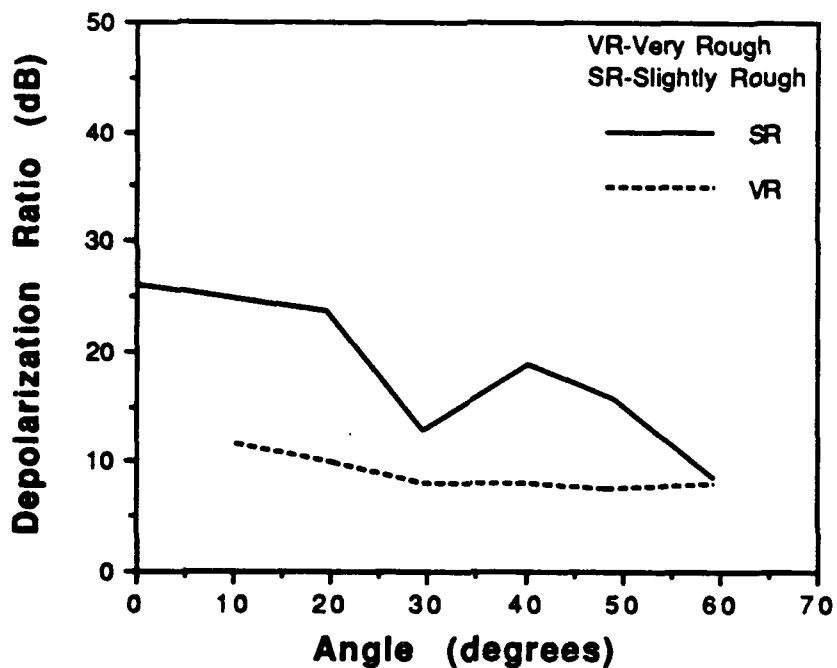
Figure 16: Depolarization response (VV + HH) / (VH + HV) for ice with a very rough surface (VR) and slightly rough surface (SR) for like and cross polarizations at 10.0 GHz.
