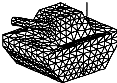
Figure 6. Tank meshed for antenna analysis at 300 MHz. 57
