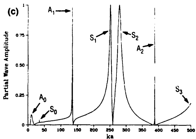
Figure 3. Partial wave for aluminum: (a) mode 1, (b) mode 2, and (c) mode 10.
