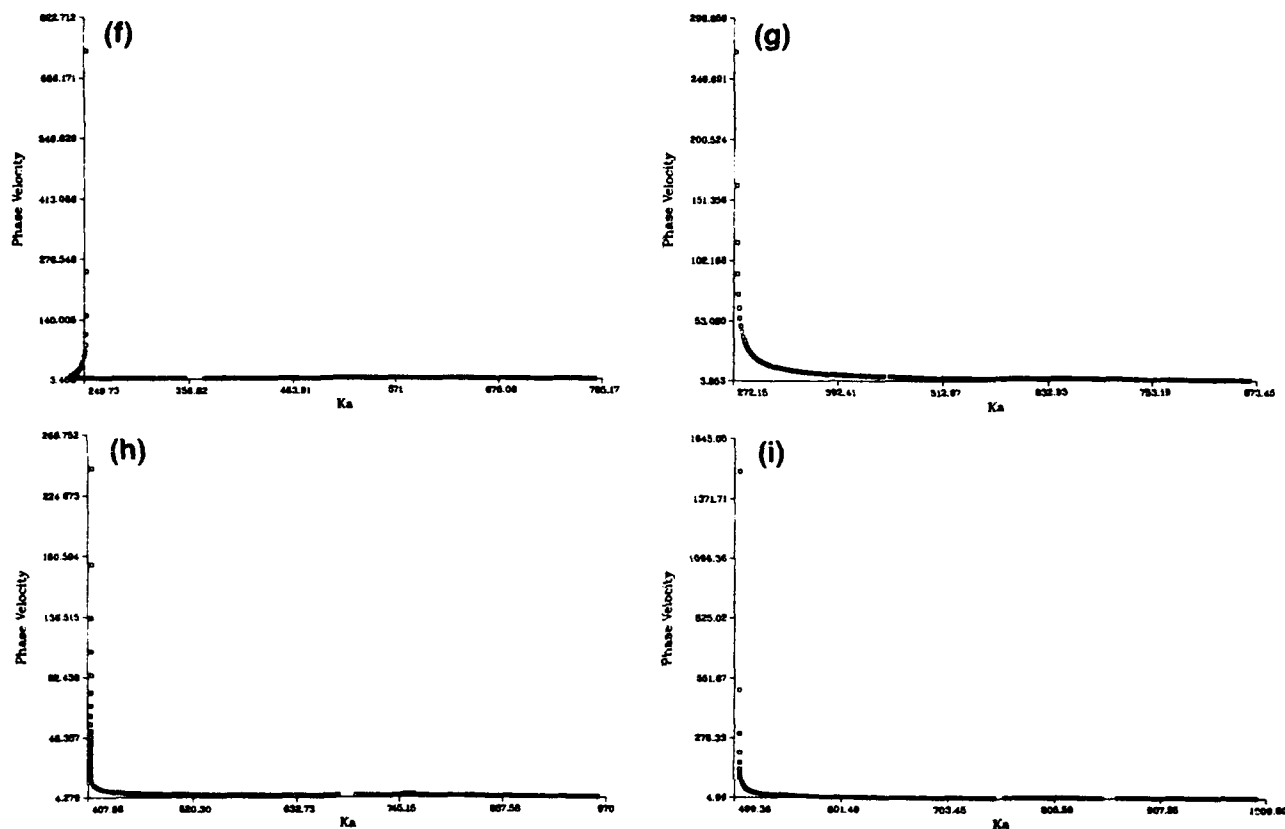
Figure 5. Phase velocity for steel (cont.) (f) S_1 resonance; (g) S_2 resonance; (h) A_2 resonance; and (i) A_3 resonance.
