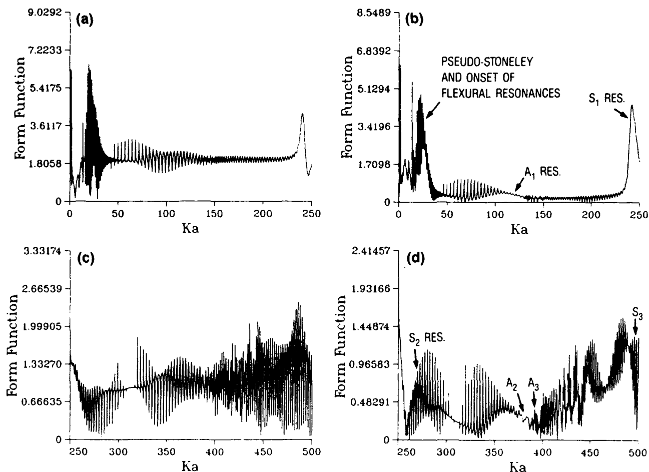
Figure 1. (a) Backscatter from 5% aluminum shell from ka = 0 to 250; (b) residual backscatter for case 1a; (c) backscatter from 5% aluminum shell from ka = 250 to 500; and (d) residual backscatter for case 1c.
