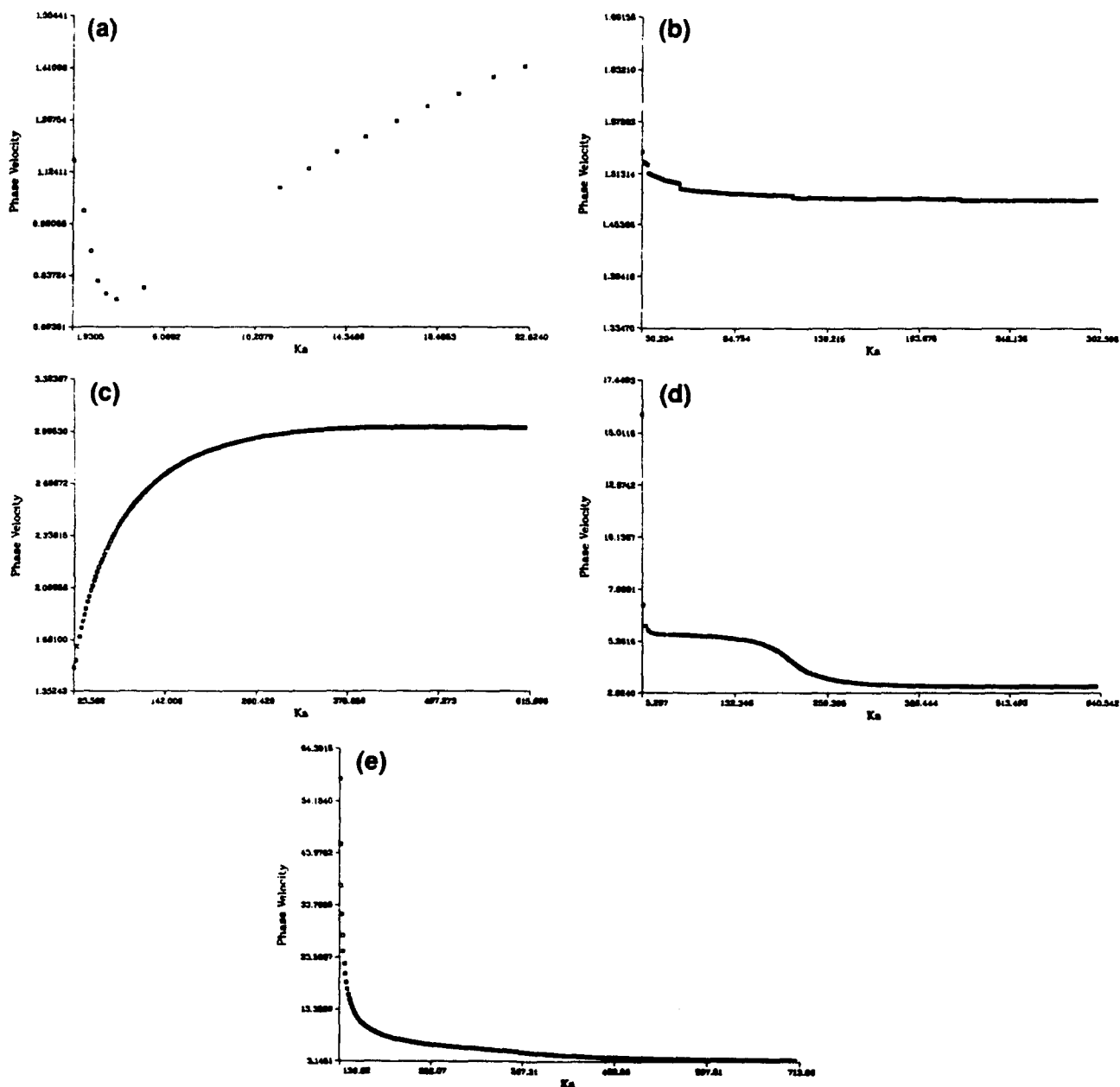
Figure 5. Phase velocity for steel: (a) pseudo-Stoneley resonance, 5% steel; (b) waterborne wave; (c) A_0 resonance; (d) S_0 resonance; (e) A_1 resonance.
