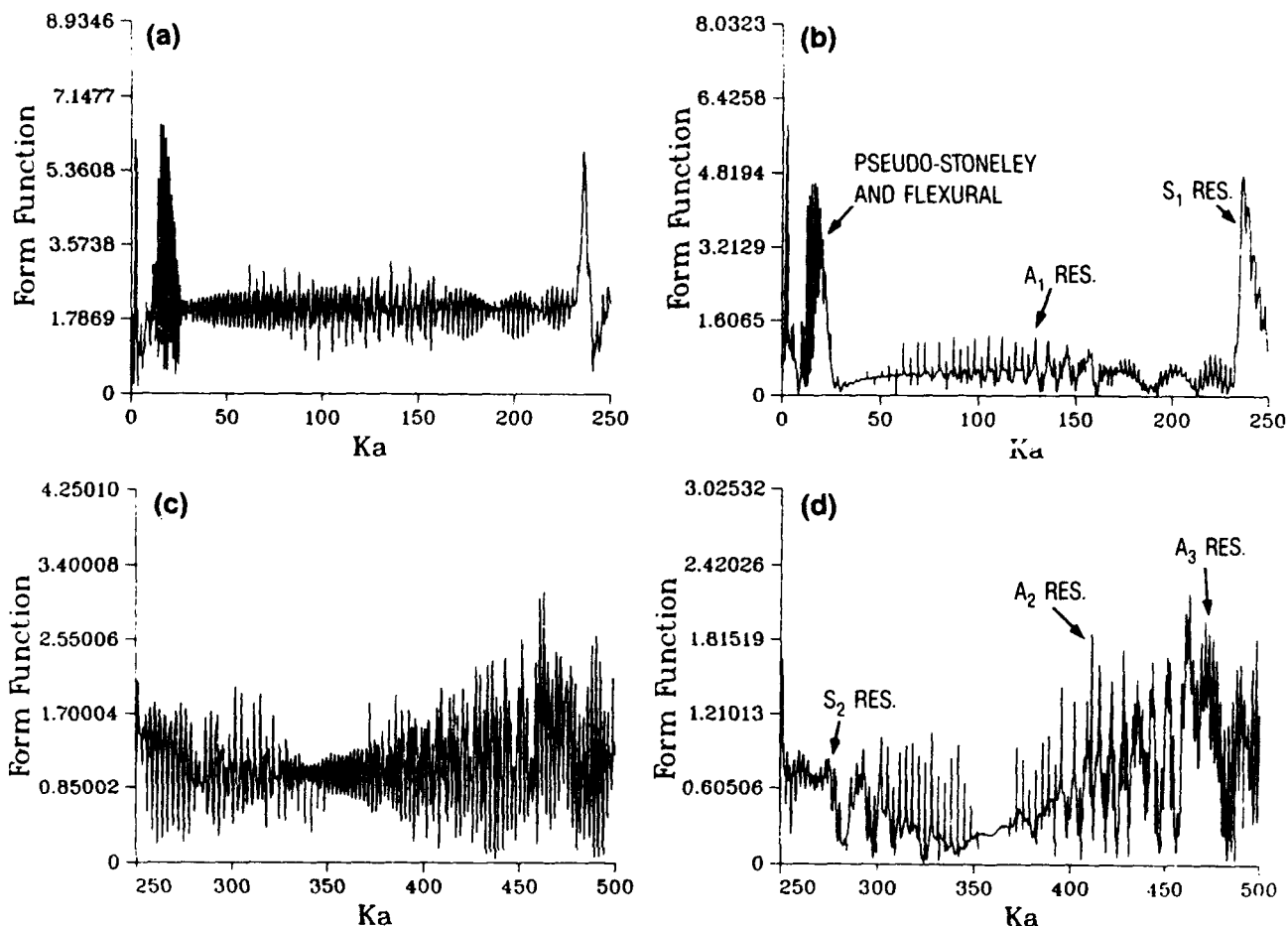
Figure 2. (a) Backscatter from 5% steel shell from ka = 0 to 250; (b) residual backscatter for case 1a; (c) backscatter from 5% steel shell from ka = 250 to 500; and (d) residual backscatter for case 1c.
