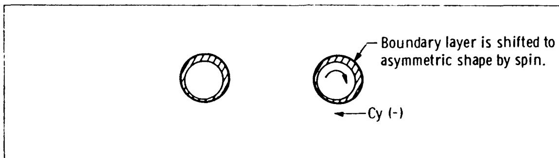
Figure 3-11 Low Angle of Attack Disturbances (15:198)
